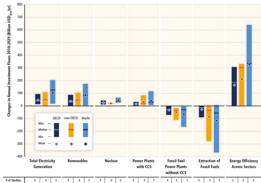
Figure 4: Annual investment over the coming two decades (2010-2029) to stabilise temperature at 2°C. Source: IPCC (2014)
