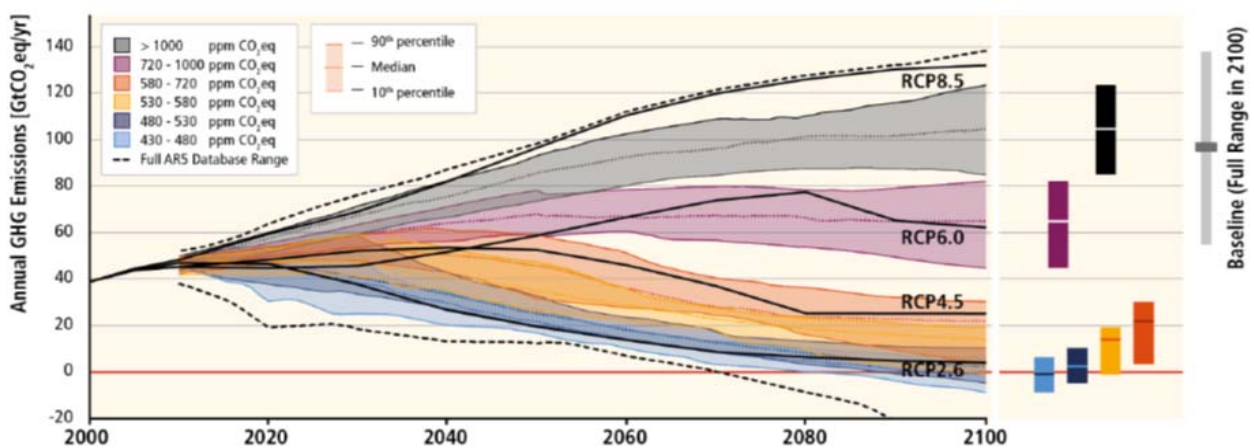
Figure 3: Emission trends (RCP 8.5) and pathway to stabilisation at 2°C (RCP 2.6) Fuente: IPCC (2014)
