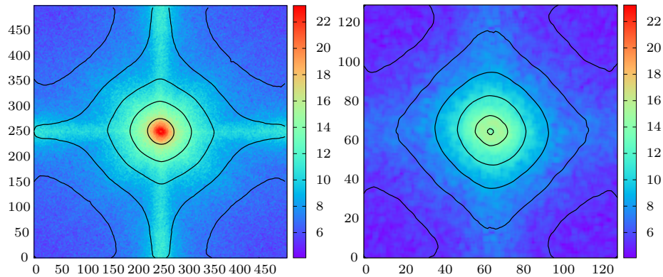
Figure 6: The same PSD: left the original 500 \times 500 pixel; right, scaled to 130 \times 130 pixels.
