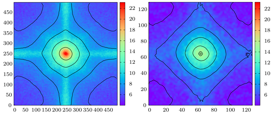
Figure 7: The same PSD: left the original 500 \times 500 pixel; right, scaled to 130 \times 130 pixels.
