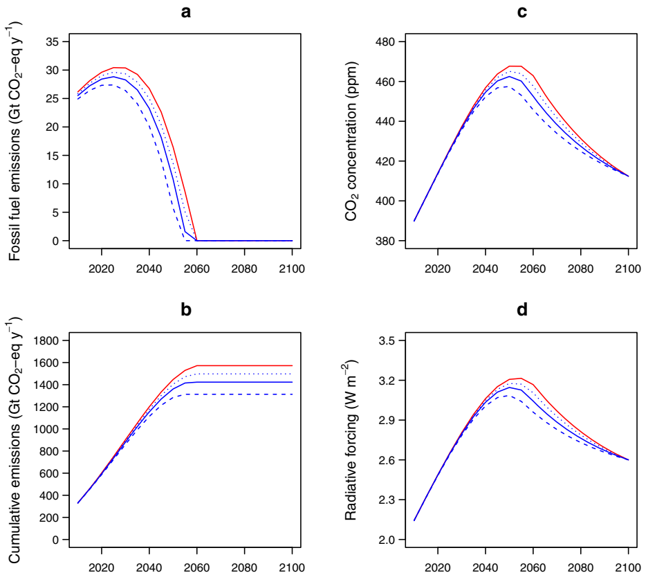
Fig. 2 Climate change control under permafrost carbon feedback. Pathway for 2010–2100 without (red) and with permafrost thawing (blue) a ) Fossil fuel and industrial \text{CO}_2 emissions, b ) Cumulative fossil fuel and industrial \text{CO}_2 emissions, c ) \text{CO}_2 concentration in the atmosphere and d ) Radiative forcing. The dashed and dotted line indicate the 68 % confidence interval associated with the permafrost emission estimates
