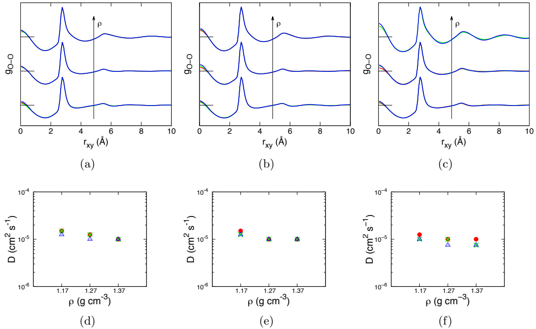
Figure 5.14: Oxygen-oxygen radial distribution function (a-c) and diffusivities (d-f) at a = 2.5 Å [(a),(e)], 2.75 Å [(b),(e)], and 3.0 Å [(c),(f)] for \alpha = 0.2 [red (a-c) and red circle (d-f)], 0.6 [green (a-c) and green cross (d-f)], 1.0 [blue (a-c) and blue triangle (d-f)]. (a-c) The RDFs are shifted on the y axis depending on the density: \rho = 1.17 g cm ^{-3} (below), 1.27 g cm ^{-3} (middle), and 1.37 g cm ^{-3} (top); the value of saturation of each curve is marked by a horizontal line.
