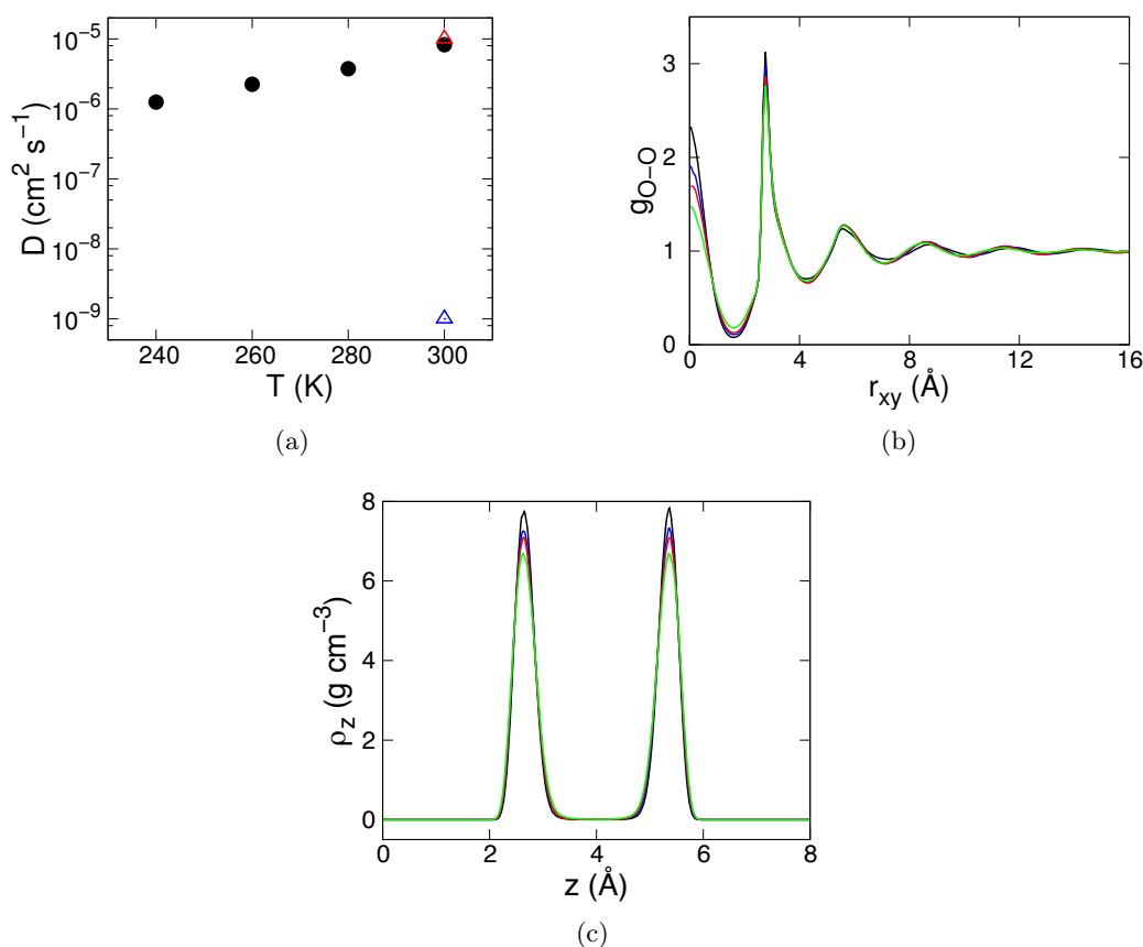
Figure 4.8: (a) In-plane diffusion constant of the oxygens at \rho = 1.37 \text{ g cm}^{-3} . The expected value of the diffusion constant for a confined bilayer water (red triangle) and bilayer ice (blue triangle) are shown for comparison. (b) In-plane oxygen-oxygen radial distribution function, and (c) density profile of the oxygens along the confining direction, both at \rho = 1.37 \text{ g cm}^{-3} and four different temperatures: 240 K (black), 260 K (blue), 280 K (red), and 300 K (green).
