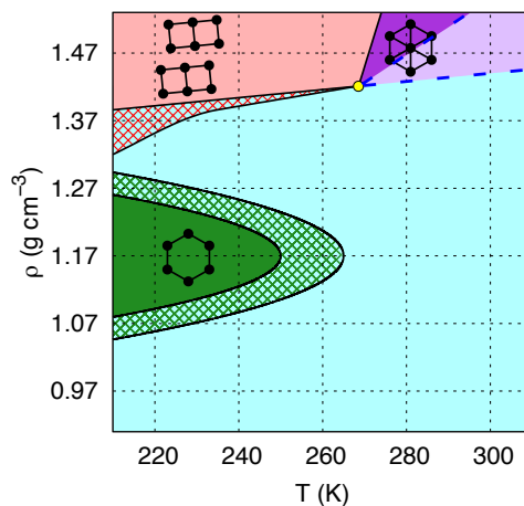
Figure 3.1: Summary of calculations and phase diagram constructed from the results. The density is defined as in Ref. [6]. The crossing points of the thin dashed grid are the points on the phase diagram sampled by MD. In the areas filled by a crosshatch we observe the coexistence of both liquid and solid phases, consistent with having a first-order phase transition in an NVT ensemble. The black lines that delimit the low temperature solid phases represent the first-order transition lines, while the blue dashed lines at high temperatures delimit the continuous phase transition lines among the liquid, hexatic and triangular ice solid phases (described in Chapter 4). These transition lines were drawn semi quantitatively from the results obtained at the sampled points. The connection point that joins the first-order and continuous phase transition lines is located at (270 \pm 10 \text{ K}, 1.42 \pm 0.05 \text{ g cm}^{-3}) .
