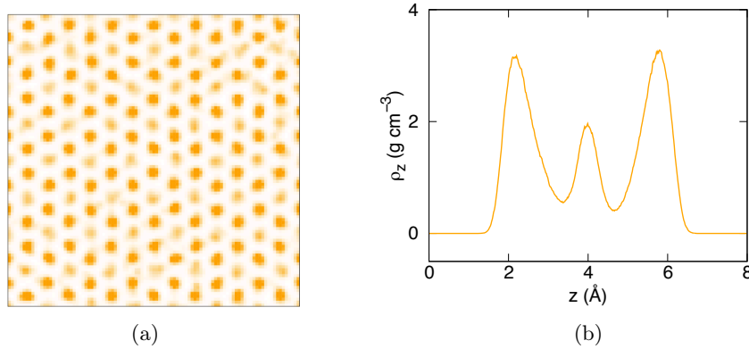
Figure 5.6: (a) xy averaged positions of the oxygens averaged over 1 ns, and (b) density profile of the oxygens, both at T = 260 K, and \rho = 1.47 \text{ g cm}^{-3} . The two exterior oxygen layers are arranged into a bilayer honeycomb lattice in a AA stacking. The oxygens from the middle layer fill the centre of the honeycomb hexagons, coinciding with the xy positions of the Lennard-Jones particles of the confining potential.
