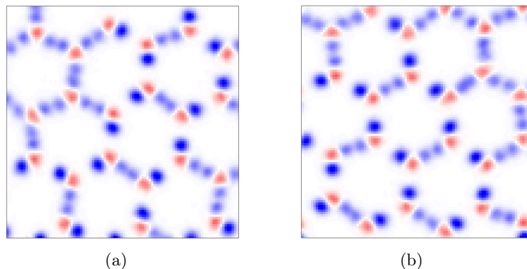
Figure 5.5: xy averaged positions of oxygen (red) and hydrogen (blue) atoms averaged over 1 ns at \rho = 1.17 \text{ g cm}^{-3} , T = 240 \text{ K} , (a) \alpha = 0.0 and (b) \alpha = 1.0 . All the images were obtained within a window of dimensions (15 \times 15) \text{ \AA}^2 in the simulation cell.
