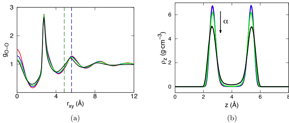
Figure 5.9: (a) Oxygen-oxygen radial distribution function, and (b) density profile both at T = 300 \text{ K} , and \rho = 1.37 \text{ g cm}^{-3} for \alpha = 0 (red), 0.2 (blue), 0.4 (green), and 0.6 (black). The vertical dashed lines in (a) highlight the second neighbor peak characteristic for the triangular ice (dark blue) and the honeycomb ice (green) RDFs.
