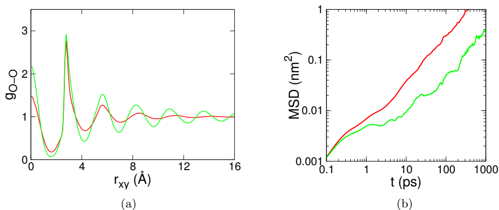
Figure 4.4: (a) In-plane oxygen-oxygen radial distribution function, and (b) mean square displacement of the oxygens at T = 300 K and \rho = 1.37 (red), and 1.47 (green) \text{g cm}^{-3}
