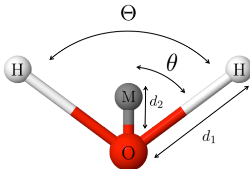
Figure 2.1: Illustration of the TIP4P/2005 water model characterized by having four sites with two distance ( d_1 , d_2 ) and two angle ( \theta , \Theta ) constraints.
