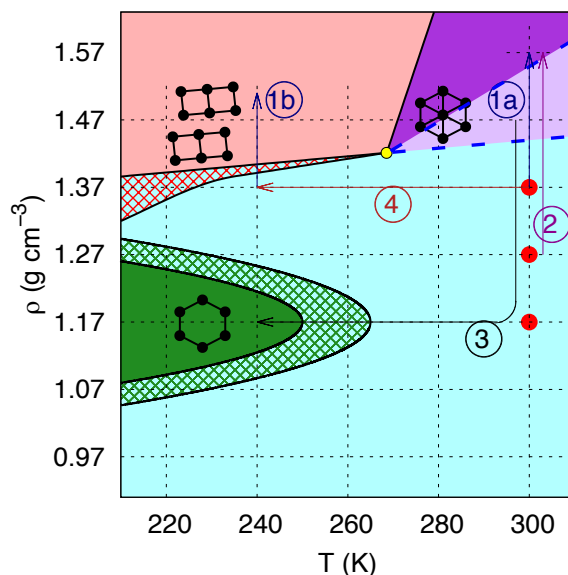
Figure 4.1: Summary of calculations and phase diagram constructed from the results (described in previous chapter). The crossing points of the thin dashed grid are the points on the phase diagram sampled by MD, while the three red circles show the points also calculated by AIMD. The numbered arrows will be useful to understand the results that are shown on the remaining part of the chapter.
