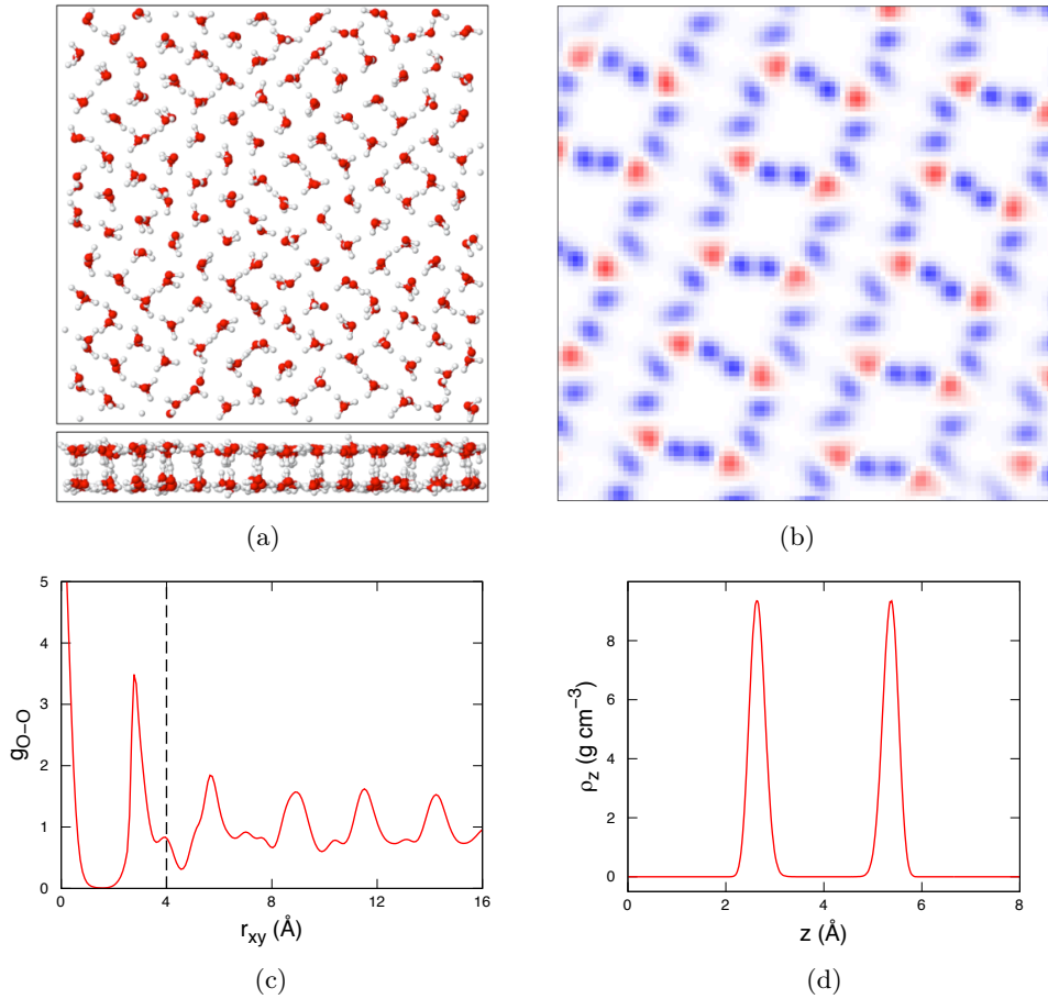
Figure 3.3: Structure of the square-tubes ice. (a) Snapshot of the simulation box showing the oxygens (red) and hydrogens (white). (b) Averaged positions of the oxygens (red) and hydrogens (blue) during 1 ns. (c) Oxygen-oxygen RDF. The vertical dashed line highlights the location of the second-neighbor peak. (d) Density profile of the oxygens.
