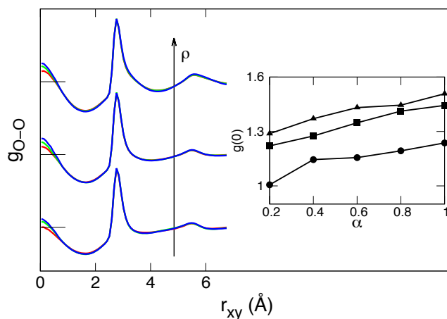
Figure 5.13: RDFs for a = 3.0 \text{ \AA} at \rho = 1.17 (below), 1.27 (middle), and 1.37 (above) \text{g cm}^{-3} at \alpha = 0.2 (red), 0.6 (green), and 1.0 (blue). The curves are shifted on the y axis; the value of saturation of each curve is marked by a horizontal finite line. The inset shows how the value g_{O-O}(0) changes for each value of density with respect to the modulation amplitude \alpha .
