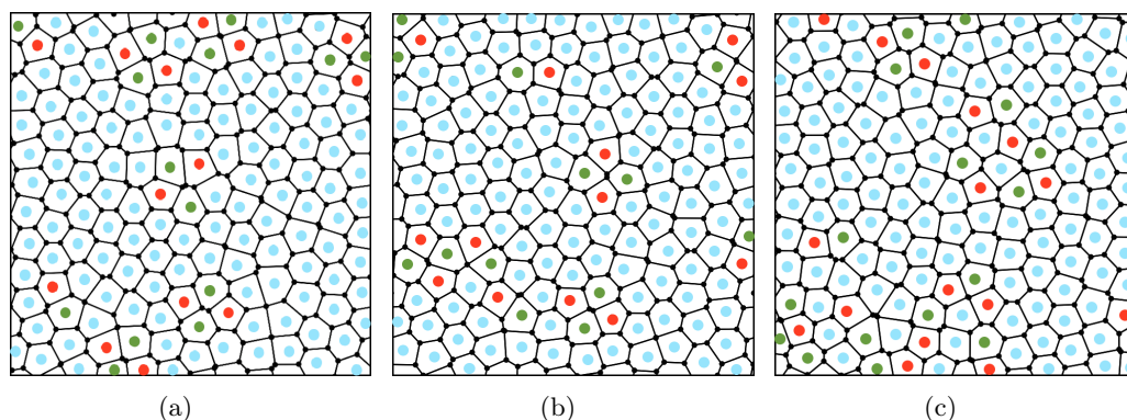
Figure 4.6: [(a)-(c)] Voronoi diagram of the oxygens located in the lower layer at \rho = 1.47 \text{ g cm}^{-3} , T = 300 \text{ K} , and three different times: (a) 0 ps, (b) 1 ps, and (c) 2 ps. Each type of polygon is marked by different colors: red (pentagon), blue (hexagon), and green (heptagon).
