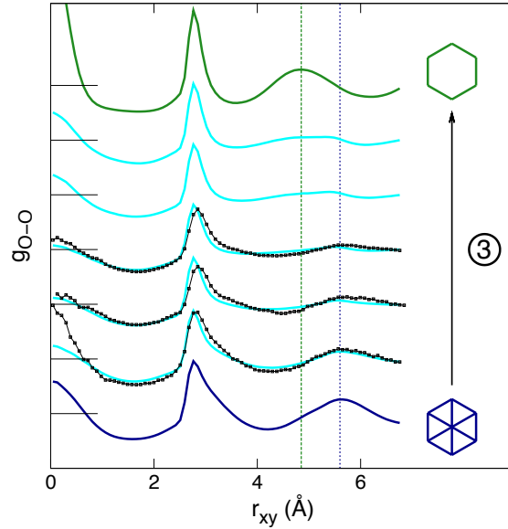
Figure 4.7: Oxygen-oxygen radial distribution functions at different densities and temperatures following the path marked by the arrow labeled 3 in Fig. 4.1. The curves are shifted on the y axis; the value of saturation of each curve is marked by a horizontal finite line. The smooth-line curves correspond to the MD calculations while the line-point curves to the AIMD calculations. The vertical dashed lines highlight the position of the second neighbor peak for the triangular ice (dark blue) and the honeycomb ice (green).
