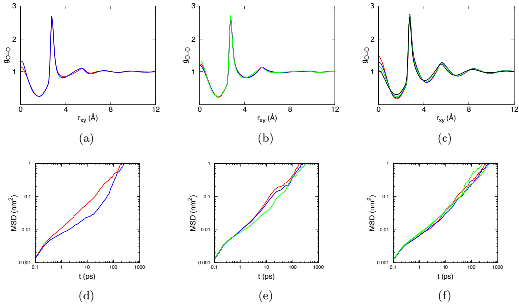
Figure 5.8: Oxygen-oxygen radial distribution function (a-c) and mean-square displacement (d-f) at \rho = 1.17 \text{ g cm}^{-3} [(a),(d)], 1.27 \text{ g cm}^{-3} [(b),(e)], and 1.37 \text{ g cm}^{-3} [(c),(f)] for \alpha = 0.0 (red), 0.2 (blue), 0.4 (green), and 0.6 (black), and a = 4.78 \text{ \AA} .
