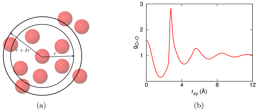
Figure 2.3: (a) To calculate the RDF, the number of particles between the radii r and r + \delta r are counted. (b) An oxygen-oxygen RDF of bilayer liquid water.
