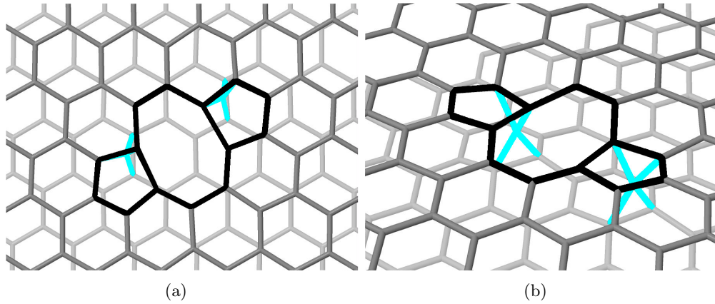
Figure 6.8: Final relaxed configuration of an intimate bi-Frenkel pair. The initial state contains a unique intimate Frenkel pair (Fig. 6.6) and a certain velocity ( T = 15 eV, \theta = 20^\circ , \varphi = 153^\circ ) is given to the scattered atom. The V_2(5-8-5) divacancy (black) is formed in the upper layer while the two scattered atoms (blue) are bridging the upper layer (dark) with the lower layer (light). (a) and (b) correspond to different perspectives.
