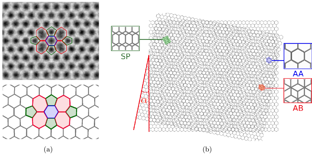
Figure 6.3: (a) Experimental image averaged over all observed butterfly defects obtained by Andrey Chuvilin [40] clearly showing its structure and a corresponding drawing of the defect. Four heptagonal (red), four pentagonal (green) and one rotated central hexagonal (blue) rings are formed instead of the original hexagonal lattice. (b) Atomic model of the graphene layers used for image simulations. One of the layers is rotated an angle \alpha = 11.2^\circ . Different local stackings are formed in different small areas within the large hexagons.
