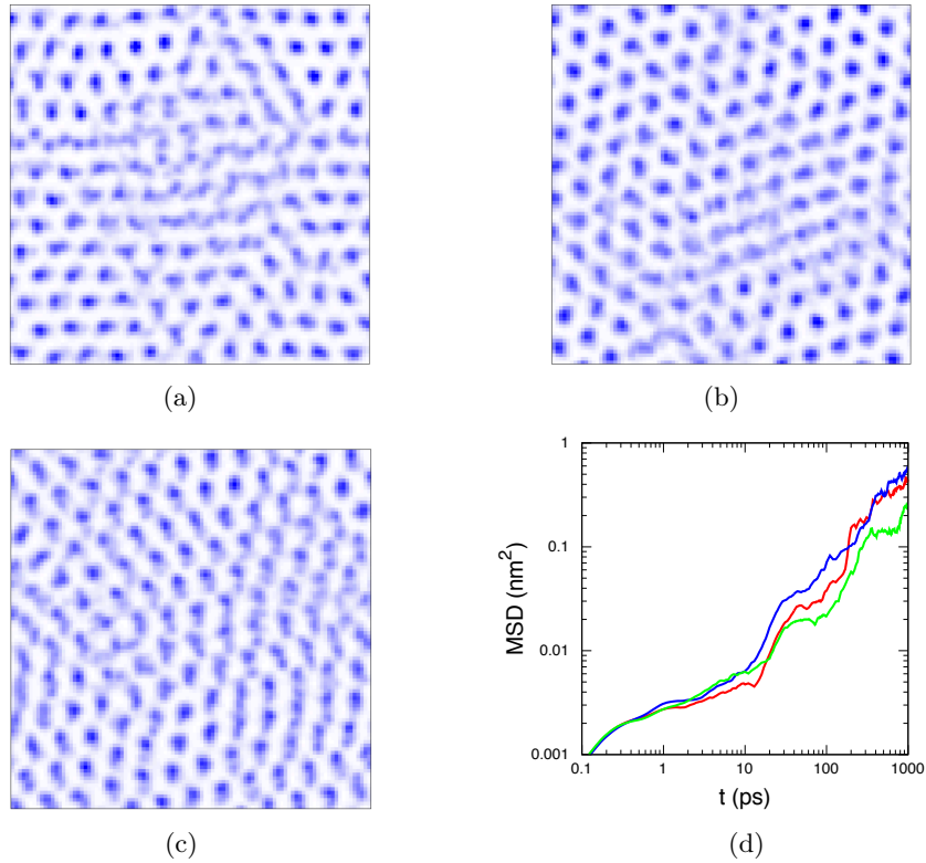
Figure 5.12: xy averaged positions of the oxygen atoms over 100 ps at T = 300 K and \rho = 1.47 \text{ g cm}^{-3} for \alpha = 1.0 and a = 2.5 \text{ \AA} (a), 2.75 \text{ \AA} (b), and 3.0 \text{ \AA} (c). (d) Mean-square displacement of oxygens at T = 300 K and \rho = 1.47 \text{ g cm}^{-3} for a = 2.5 \text{ \AA} (red), 2.75 \text{ \AA} (blue), and 3.0 \text{ \AA} (green).
