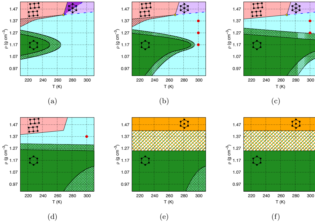
Figure 5.1: Summary of calculations and phase diagram constructed from the results for a lattice parameter a = 4.78 \text{ \AA} and \alpha = (a) 0.0, (b) 0.2, (c) 0.4, (d) 0.6, (e) 0.8 y (f) 1.0. The density is defined as in Ref. [1]. The crossing points of the thin dashed grid are the points on the phase diagram sampled by MD, while the six red circles show the points also calculated by AIMD. In the areas filled by a crosshatch we observe the solid-liquid or solid-solid coexistence, consistent with having a first-order phase transition in an NVT ensemble. The black lines represent the first-order transition lines, while the blue dashed lines delimit the continuous phase transition lines among the liquid, hexatic and triangular ice solid phases. These transition lines were drawn semi quantitatively from the results obtained at the sampled points. Blue indicates the liquid phase. The other phases are described in the text.
