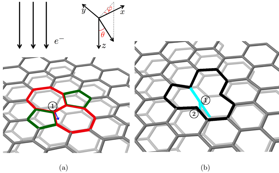
Figure 6.7: (a) Initial state of the AIMD simulation with a Stone-Wales defect. It is made by two heptagonal (red) and two pentagonal (green) carbon rings. The blue arrow points in the direction ( \theta = 12^\circ , \varphi = 1^\circ ) of the initial velocity ( T = 17 eV) which is given to the scattered atom (atom 1). (b) Final state of the same simulation in which the intimate Frenkel pair is stabilized. In the upper layer a vacancy is formed (black) and the scattered atom remains trapped between both layers (blue, atom 1) bridging the upper layer (dark) with the lower layer (light). The atom 2 is ‘kicked’ in the next simulation to obtain the intimate bi-Frenkel pair.
