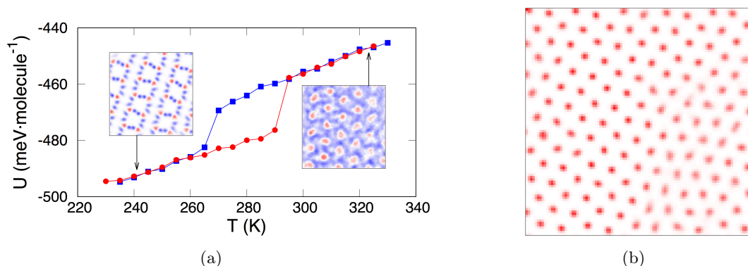
Figure 3.5: (a) Potential energy per molecule in the heating (red) and cooling (blue) processes as a function of the temperature. The insets show the averaged positions of the oxygens (red) and hydrogens (blue) for the two solids involved in the phase transition: the square-tubes ice at low temperatures, and the triangular ice at high temperatures. (b) Averaged position of the oxygens (red) at T = 265 K and \rho = 1.47 g cm ^{-3} . The coexistence of square-tubes ice (top left) and triangular ice (bottom right) can be clearly observed.
