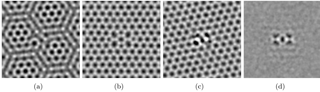
Figure 6.4: Simulated image by Andrey Chuvilin [40] of the central part shown at the same scale and with the same processing as experimental images in Figs. 6.2(c)–6.2(f). The butterfly defect is located in the first layer and the second one is kept pristine. The feature similar to Fig. 6.2(e) is observed on the simulated second layer (c) comprising pristine graphene. It can be thus concluded that this feature in the second layer is an artifact of Fourier filtering.
