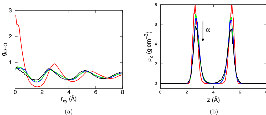
Figure 5.11: (a) Oxygen-oxygen interlayer radial distribution function, and (b) density profile both at T = 300 K and \rho = 1.37 \text{g cm}^{-3} for \alpha = 0 (red), 0.2 (blue), 0.4 (green), and 0.6 (black).
