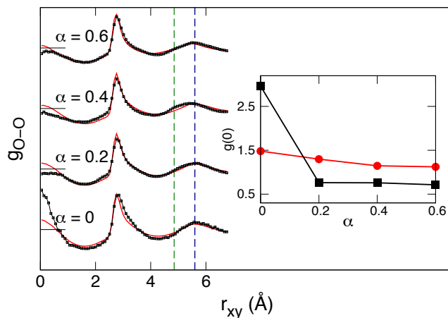
Figure 5.10: Oxygen-oxygen radial distribution functions at T = 300 K, and \rho = 1.37 \text{g cm}^{-3} for different values of \alpha . The curves are shifted on the y axis; the value of saturation of each curve is marked by a horizontal line. The smooth-line curves correspond to the MD calculations while the line-points curves to the AIMD calculations. The vertical dashed lines highlight the position of the second neighbor peak characteristic in the triangular ice (dark blue) and the honeycomb ice (green) RDFs. The inset shows the value at the origin of the RDFs obtained by MD calculations (red circles), and AIMD calculations (black squares).
