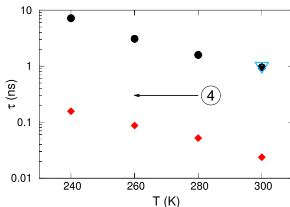
Figure 4.9: Vertical-jump lifetime ( \tau_z ) obtained from MD (circles) and AIMD (triangle) calculations and the in plane-jump lifetime ( \tau_{xy} , rhombuses) at \rho = 1.37 \text{ g cm}^{-3} and different temperatures (arrow 4 in Fig. 4.1).
