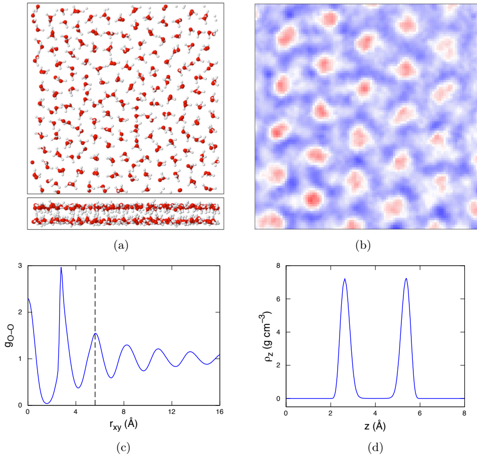
Figure 3.4: Structure of the triangular ice. (a) Instantaneous snapshot of the simulation box showing the oxygens (red) and hydrogens (white). (b) Averaged positions of the oxygens (red) and hydrogens (blue) during 1 ns. (c) Oxygen-oxygen RDF. The vertical dashed line highlights the position of the second-neighbor peak. (d) Density profile of oxygens.
