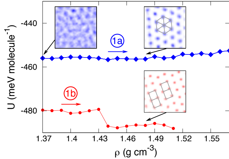
Figure 4.3: Potential energy as a function of density for T = 240 K (bottom, red) and T = 300 K (top, blue). The 1a and 1b arrows refer to the paths on the phase diagram (see Fig. 4.1). The insets show the averaged positions of the oxygens during 100 ps in a window of dimensions (15 \times 15) \text{ \AA}^2 within the cell. The gray lines within the high-density insets are drawn to illustrate the different structures of each ice.
