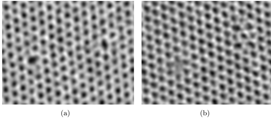
Figure 6.5: Enlarged experimental HRTEM images obtained during experiment by Andrey Chuvilin [40]. The second honeycomb lattice is filtered out. (a) Two V_2(5-8-5) divacancies are distinguished in the first. (b) After 7.5 e/nm^2 of electronic dose, one of the divacancies (left) is in the process of transformation while the other (right) is converted into a butterfly defect.
