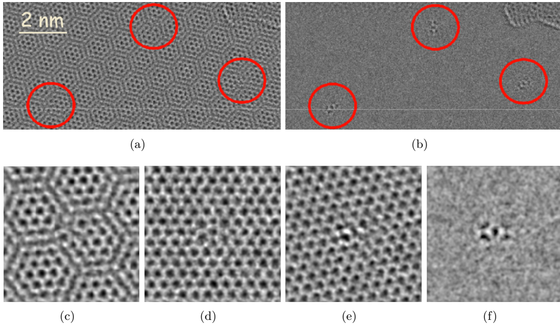
Figure 6.2: HRTEM images of bilayer graphene obtained by Andrey Chuvilin [40]. (a) Overview image showing the obtained Moiré pattern. In the regions marked by the circles the distortions of the pattern are visible. (b) The same area, but the honeycomb lattices of both layers are removed by Fourier filtering. Characteristic patterns in the shape of double dumbbells appear inside the circles indicating the same type of lattice distortion in all three places. (c) Enlarged image of one of the distorted Moiré pattern areas. (d)–(f) Fourier filtered images of the enlarged area with the second (d), first (e) and both graphene layers filtered out (f). The image of the first layer only (d) can be directly interpreted in terms of atom positions and reveals a V_2(5555-6-7777) butterfly defect formation in this layer. Image of the second layer (e) cannot be interpreted directly and needs simulations in order to find its origin.
