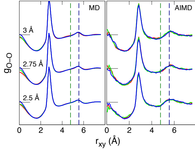
Figure 5.16: RDFs obtained by MD (left), and AIMD (right) calculations at T = 300 K, and P_{\parallel} = 0 . A different height is given to the curves for each lattice parameter: a = 2.5 (bottom), 2.75 (middle), and 3.0 Å (top). For each lattice parameter, there are three curves, each one corresponding to a different value of \alpha = 0.2 (red), 0.6 (green), and 1.0 (blue). The value of saturation of each curve is marked by a horizontal line. The vertical dashed lines highlight the position of the second neighbor peak for the triangular ice (dark blue) r_t = 2r_{\text{O-O}} and the honeycomb ice (green) r_h = \sqrt{3}r_{\text{O-O}} .
