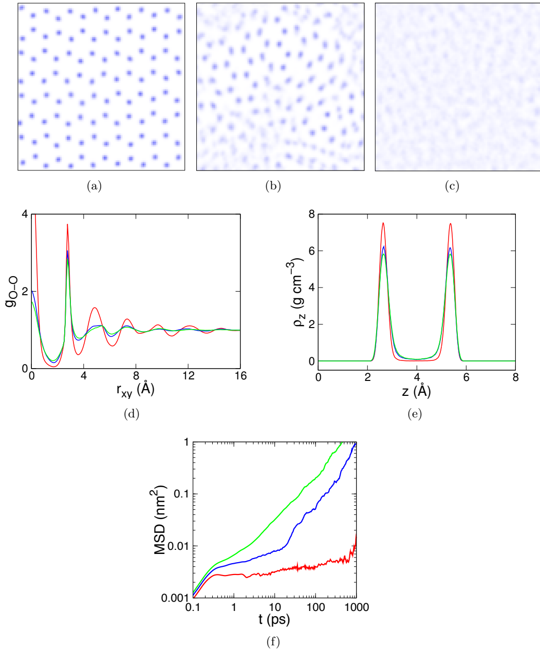
Figure 4.2: [(a)-(c)] Averaged positions of the oxygens (blue) during 100 ps at \rho = 1.17 \text{ g cm}^{-3} and three different temperatures: (a) 240 K, (b) 260 K, and (c) 280 K. (d) In-plane oxygen-oxygen radial distribution function, (e) density profile of the oxygens along the confining direction, and (f) in-plane mean square displacement of the oxygens at \rho = 1.17 \text{ g cm}^{-3} and three different temperatures: 240 K (red), 260 K (blue), and 280 K (green).
