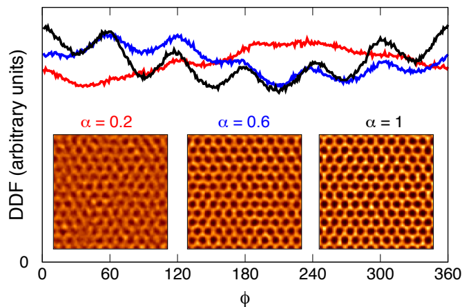
Figure 5.15: Dipolar angle distribution function of the water molecules for a = 3.0 \text{ \AA} at T = 300 \text{ K} , \rho = 1.27 \text{ g cm}^{-3} , and \alpha = 0.2 (red), 0.6 (blue), and 1.0 (black). The insets show the xy averaged positions of the oxygens at the three values of \alpha : the brighter the color, the larger the density.
