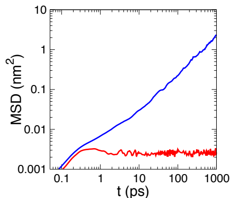
Figure 2.4: Mean square displacement of a two-dimensionally confined liquid (blue) and solid (red). Until t \sim 0.2 ps, the particles from both phases are in the ballistic regime and follow \Delta_{xy}(t) \propto t^2 . In the diffusive regime, the curve of the solid saturates while the one of the liquid scales linearly with time.
