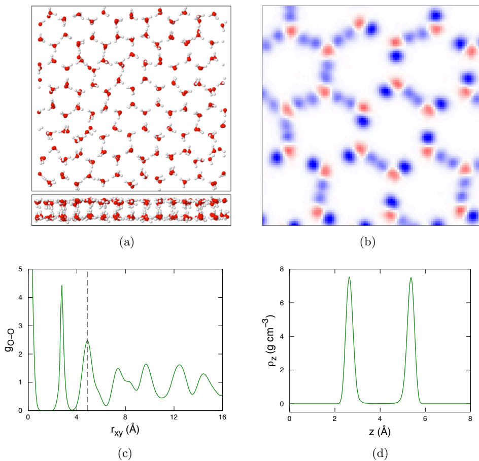
Figure 3.2: Structure of the honeycomb ice obtained at T = 240 K, and \rho = 1.17 g cm -3 . (a) Instantaneous snapshot of the simulation box showing the oxygens (red) and hydrogens (white). (b) Averaged positions of the oxygens (red) and hydrogens (blue) during 1 ns in a window of dimensions (15 \times 15) Å 2 within the cell. (c) Oxygen-oxygen RDF. The vertical dashed line highlights the location of the second-neighbor peak. (d) Density profile of the oxygens.
