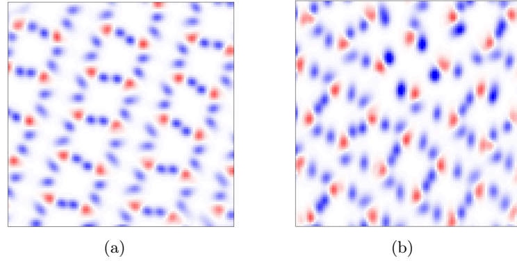
Figure 5.3: xy averaged positions of oxygen (red) and hydrogen (blue) atoms averaged over 1 ns at T = 220 K, \rho = 1.47 g cm ^{-3} , and \alpha = 0 (a), 0.6 (b). All the images were obtained within a window of dimensions (15 \times 15) Å ^2 in the simulation cell.
