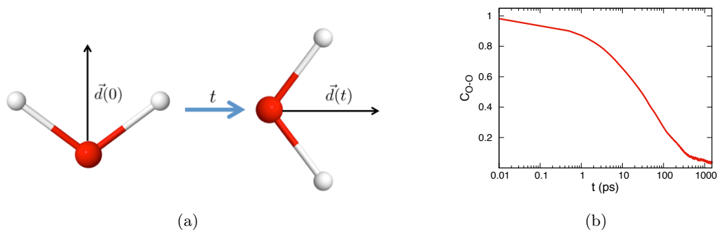
Figure 2.5: (a) After time t , the orientation of a molecule changes and the projection of the dipole with the initial dipole is smaller than 1. (b) Dipole-dipole autocorrelation function in liquid water. After a characteristic time, the information of the initial molecular orientation is lost.
