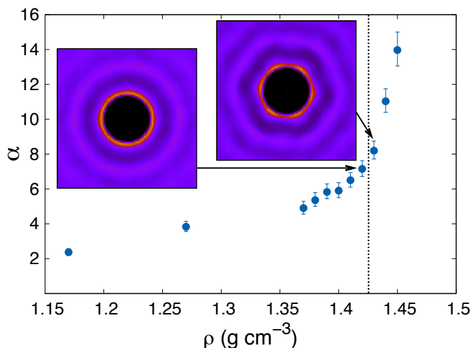
Figure 4.10: Ratio between the characteristic times of \text{C}_{\text{O-O}} and \text{C}_{\text{H}_2\text{O}} at T = 300 K with respect to density (main plot) and 2D oxygen-oxygen correlation function (insets) at \rho = 1.42 (left) and 1.43 \text{g cm}^{-3} (right): the brighter the color, the larger the value of the 2D oxygen-oxygen correlation function. The vertical dashed line represents the estimated density in which the liquid-hexatic transition occurs.
