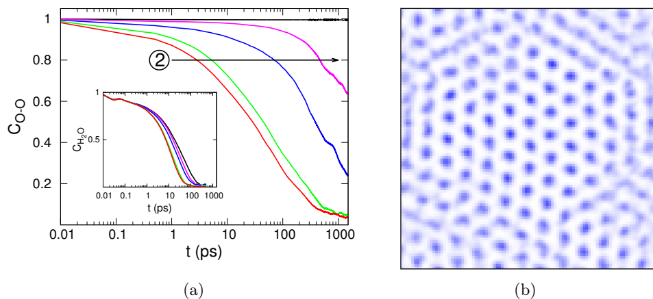
Figure 4.5: (a) Oxygen-oxygen first-neighbor correlation function (main plot) and dipole-dipole autocorrelation function (inset) as a function of time at T = 300 K and five different densities: \rho = 1.27 (red), 1.37 (green), 1.47 (blue), 1.54 (pink), and 1.57 (black) \text{g cm}^{-3} . The path followed on the phase diagram is the one shown by the arrow labeled 2 in Fig. 4.1. (b) Averaged positions of the oxygens during 100 ps.
