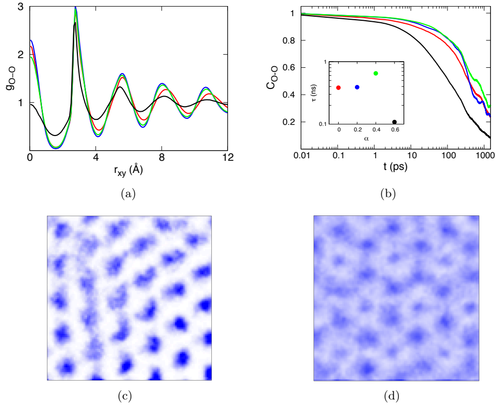
Figure 5.4: (a) Oxygen-oxygen radial distribution function and (b) oxygen-oxygen first-neighbor correlation function at T = 300 K and \rho = 1.47 g cm ^{-3} for a = 4.78 Å and \alpha = 0 (red), 0.2 (blue), 0.4 (green), and 0.6 (black). The inset in (b) shows the characteristic time for each curve. (c-d): averaged position of oxygens (blue) during 100 ps at T = 300 K, \rho = 1.47 g cm ^{-3} , and \alpha = 0.4 (b), 0.6 (c). The images were obtained by averaging in time, within a window of dimensions (15 \times 15) Å ^2 in the simulation cell.
