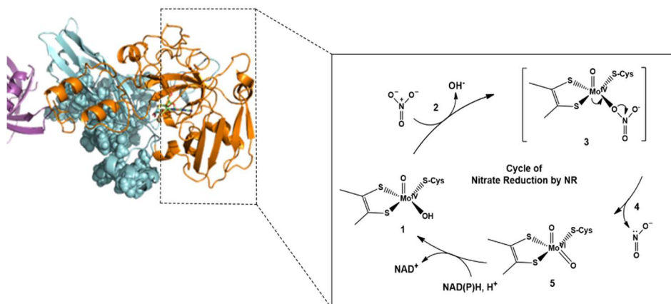
Figure 4.1. Hypothetical reaction cycle of nitrate reduction by NR. The reaction starts with the reduced \text{Mo}^{\text{IV}} form (1). Then, nitrate binds to the active site (2) and replaces the equatorial hydroxo/water ligand, forming an intermediate (3). The bond between the nitrate oxygen and nitrogen is broken and nitrite is released (4); consequently, the Mo center is oxidized to \text{Mo}^{\text{VI}} (5). After completion of the reductive half-reaction, the Mo is regenerated [ \text{Mo}(\text{IV}) ] for the next cycle. Adapted from the reference 12 .
