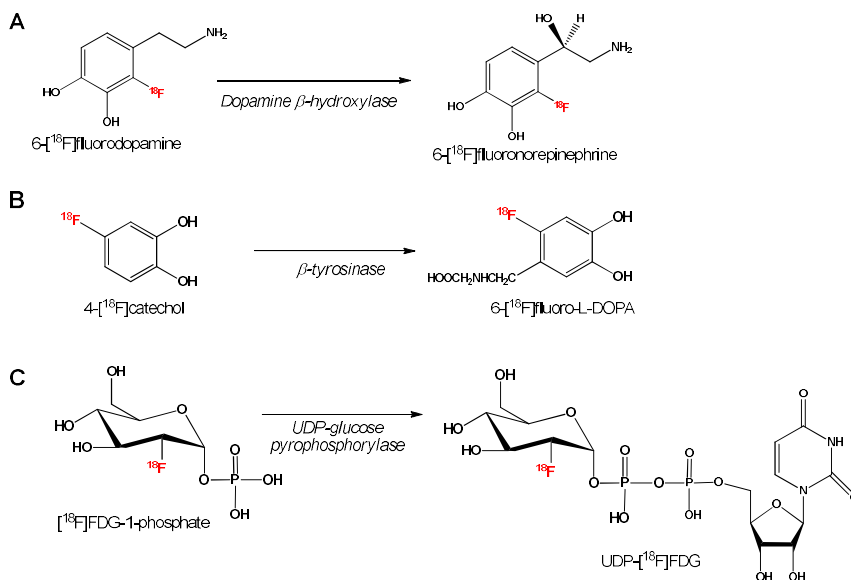
Figure 2.7. Schematic representation of the enzymatic reaction to synthesize (–)-6-[ 18 F]fluoronorepinephrine (A), 6-[ 18 F]fluoro- L -DOPA (B) and UDP-[ 18 F]FDG (C). The radiosynthesis of these molecules was achieved starting from the respective 18 F-labeled substrates using dopamine β-hydroxylase, β-tyrosinase and UDP-glucose pyrophosphorylase, respectively.
