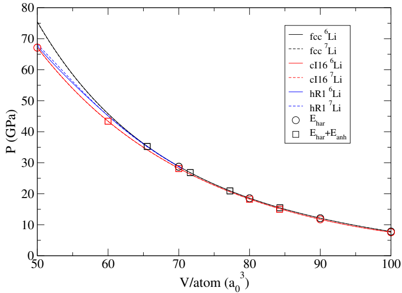
Figure 10.10: Pressure of fcc, cI16 and hR1 Li for both isotopes. The symbols show data points in which harmonic ( E_{har} ) and anharmonic ( E_{anh} ) vibrational data has been explicitly calculated.
