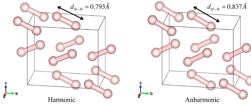
Figure 7.1: Crystal structure of Cmca-4 hydrogen at 414 GPa at the harmonic and anharmonic level in the conventional orthorhombic lattice. The hydrogen intramolecular distance d_{H-H} is shown for each case.
