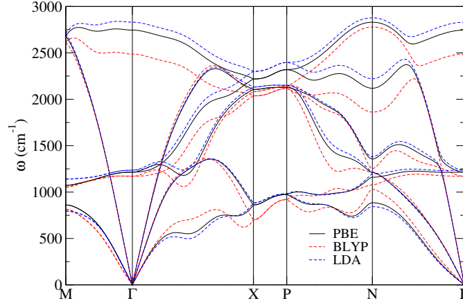
Figure 6.8: Phonon spectra of I4_1/amd hydrogen at 500 GPa within different approximations for the exchange and correlation functional [45, 46, 173].
