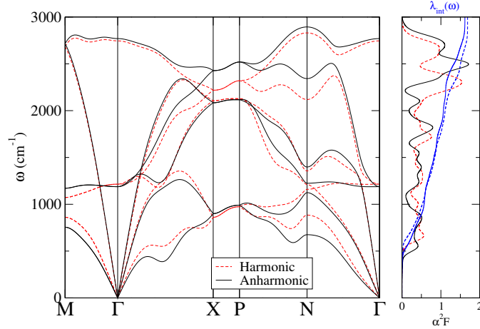
Figure 6.9: Left: harmonic and anharmonic phonon spectra of I4_1/amd hydrogen at 500 GPa. Right: harmonic and anharmonic electron-phonon spectral function \alpha^2F(\omega) and frequency dependent electron-phonon coupling constant \lambda_{\text{int}}(\omega) .
