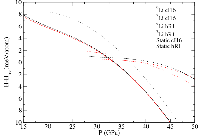
Figure 10.11: Relative enthalpies of cI16 and hR1 {}^6\text{Li} and {}^7\text{Li} isotopes with respect to their fcc counterparts. In solid and dashed lines E_v has been included, while in dotted curves only electronic energy has been considered. The low pressure limit for the hR1 curves has been set at the pressure which corresponds, in each case, to the maximum volume at which the phase shows a local minimum in the total energy surface (see Fig. 10.9).
