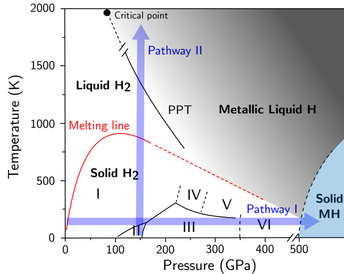
Figure 5.1: Experimental/theoretical pressure vs. temperature phase diagram of hydrogen. It shows the two pathways to metallic hydrogen: I the low temperature pathway and II the high temperature pathway. In pathway I phases of solid hydrogen are shown with their Latin number names. The plasma phase transition (PPT) is the liquid-liquid transition to metallic atomic hydrogen. Dashed lines emphasize uncertainty in the phase boundaries. This graph has been adapted from Ref. [138].
