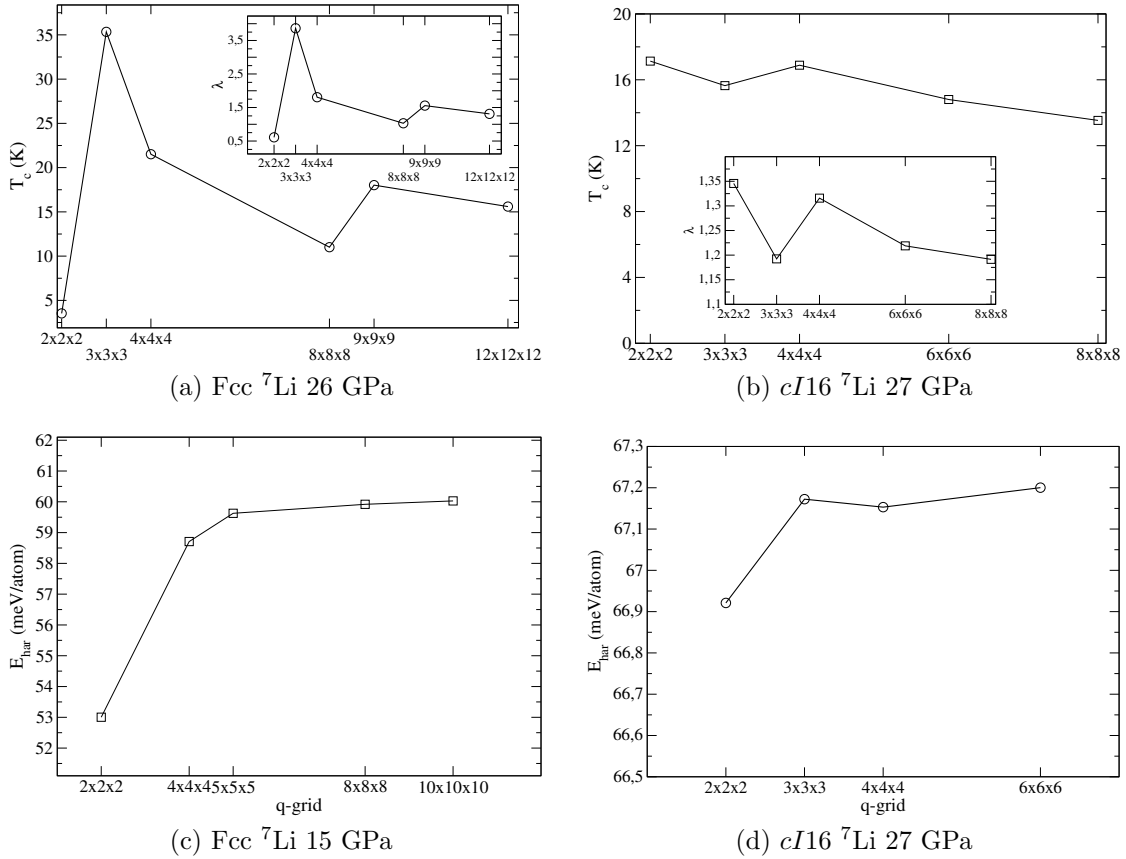
Figure 10.4: Convergence of T_c and \lambda with the \mathbf{q} -grid for (a) fcc and (b) cI16 {}^7\text{Li} , using McMillan equation and \mu^* = 0.17 and convergence of E_{har} with the \mathbf{q} -grid for (c) fcc and (d) cI16 {}^7\text{Li} .
