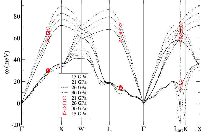
Figure 10.1: Harmonic (black curves) and anharmonic (red symbols) phonon spectra of fcc {}^7\text{Li} at different pressures. Harmonic spectra are obtained by Fourier interpolating the 9 \times 9 \times 9 \mathbf{q} -grid data to the desired path. Anharmonic data corresponds to SSCHA calculations in a 3 \times 3 \times 3 \mathbf{q} -point grid.
