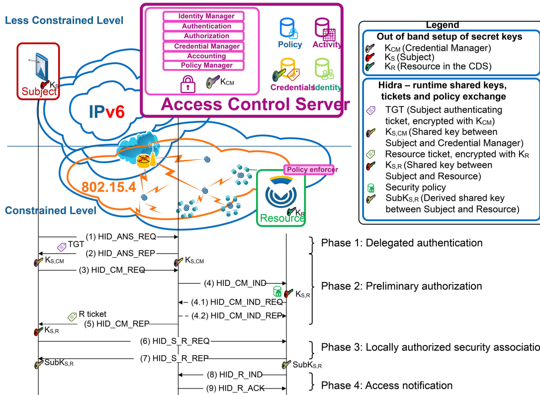
Fig. 4 Hidra protocol messages and security association establishment related authentication, authorisation, key exchange and notifications
