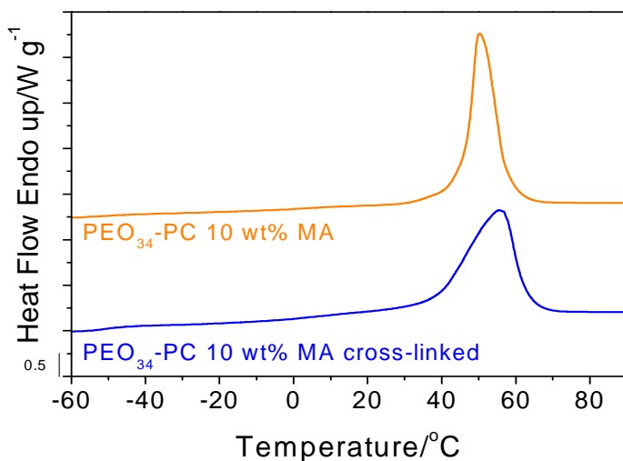
Figure S2. DSC traces of non-cross-linked and cross-linked PEO 34 -PC 10 wt% MA during the second heating scan at 20 K min -1 .
