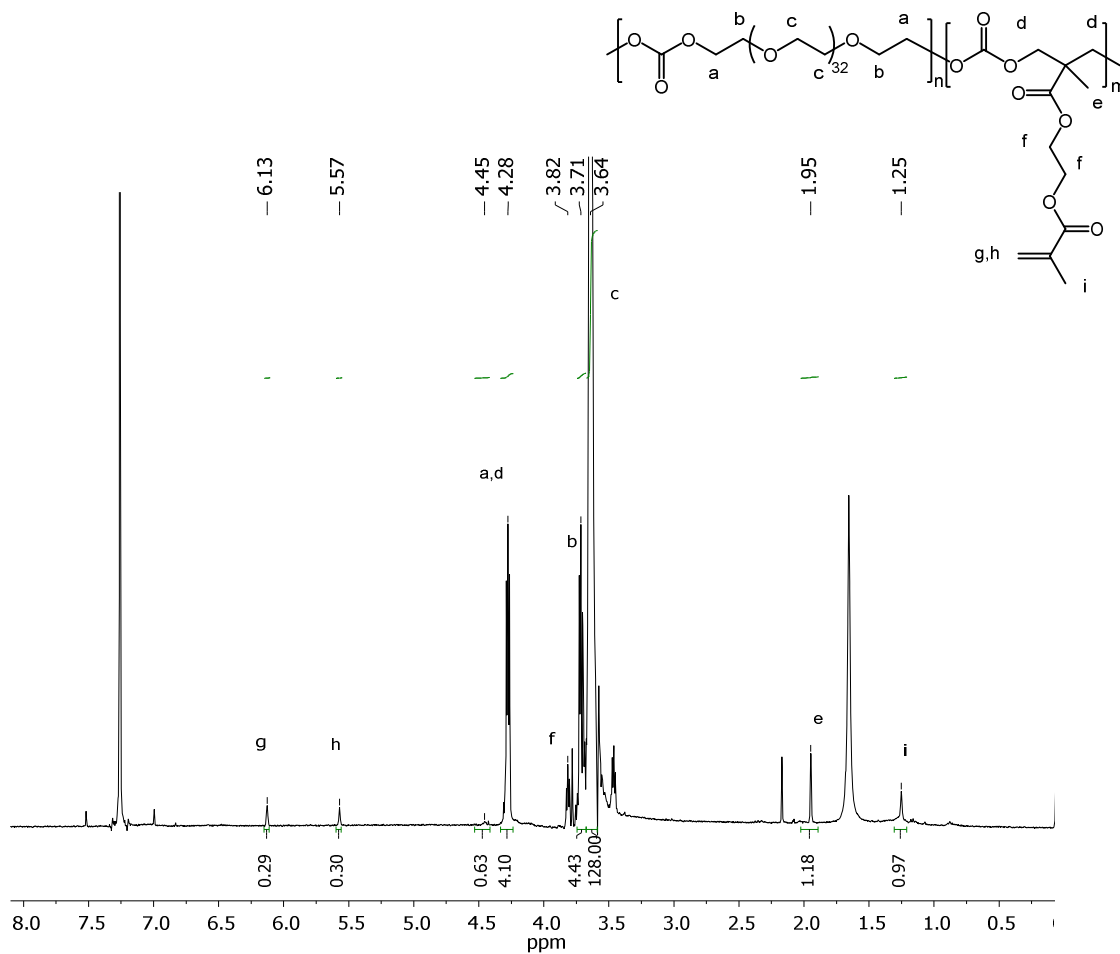
Figure S1. 1 H NMR of PEO 34 -PC 10 wt% MA
