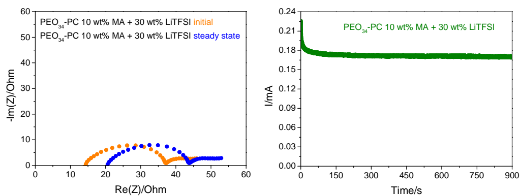
Figure S4. Lithium transference number analysis at 70 °C. Impedance spectroscopy and chronoamperometry analysis for PEO 34 -PC 10 wt% MA containing 30 wt% LiTFSI.
