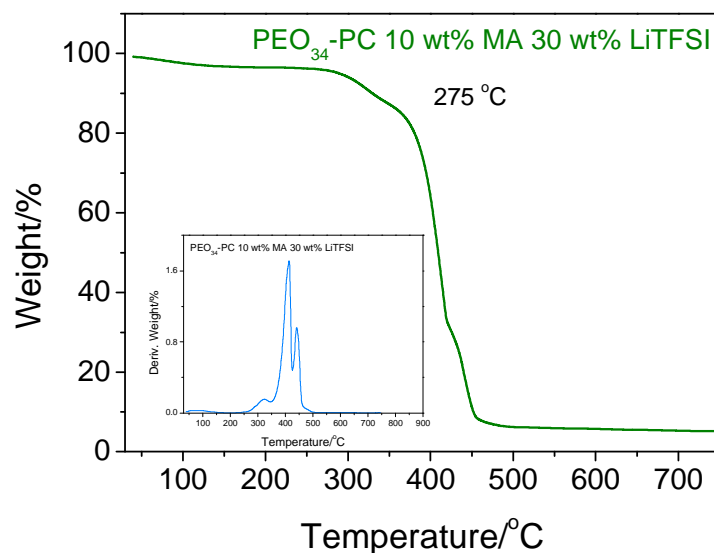
Figure S3. Thermogravimetric analysis of cross-linked PEO 34 -PC 10 wt% MA containing 30 wt% LiTFSI.
