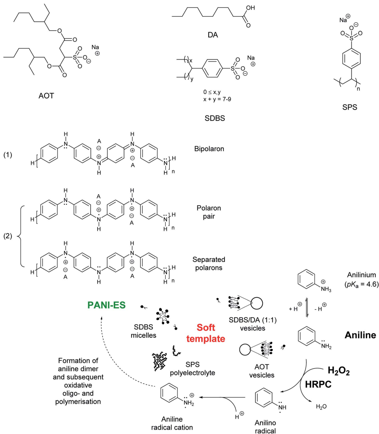
Scheme 1 Schematic illustration of the horseradish peroxidase isoenzyme C (HRPC)/ H_2O_2 -catalysed oxidation of aniline at pH = 4.3 ( 0.1 M NaH_2PO_4 + H_3PO_4 ) and T \approx 25^\circ C in the presence of one of four different types of soft anionic templates: AOT vesicles, vesicles from a 1 : 1 molar mixture of sodium dodecylbenzenesulfonate (SDBS) and decanoic acid (DA), SDBS micelles, or sulfonated polystyrene (SPS) polyelectrolyte. All template molecules have one or more sulfonate groups and the reactions are initiated by adding aniline, HRP, and H_2O_2 to the template solutions or suspensions. Each reaction can be run under conditions which result in products that are rich in the conductive PANI-ES form. Chemical structures of the ideal PANI-ES repeating unit are shown in its diamagnetic bipolaron (1) and paramagnetic polaron forms (2). Mechanistically, HRP is first oxidised by H_2O_2 in a two-electron oxidation. Oxidised HRP then oxidises two aniline molecules in two one-electron oxidations to yield two anilino radicals. After protonation to yield aniline radical cations, coupling reactions and further oxidation steps lead to the formation of PANI-ES repeating units (and other undesired side products). The templates "promote" desired PANI-ES product formation, act as counter ions ( A^- ), and prevent precipitation of the otherwise insoluble PANI-ES reaction products.
