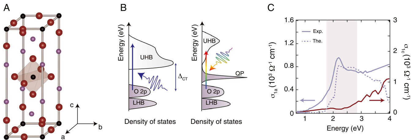
Fig. 1. (A) Crystallographic structure of \text{La}_2\text{CuO}_4 in its low-temperature orthorhombic unit cell. The Cu atoms are depicted in black, the O atoms in red, and the La atoms in violet. The brown shading emphasizes the \text{CuO}_6 octahedron in the center. (B) Schematic representation of the interacting density of states in undoped insulating (Left) and photodoped metallic (Right) \text{La}_2\text{CuO}_4 . The O-2p, lower Hubbard band (LHB), upper Hubbard band (UHB), and quasiparticle (QP) peak are indicated. In the insulating case, the optical charge-transfer gap ( \Delta_{\text{CT}} ) is also specified. The blue arrow indicates the 3.10-eV pump pulse, which photodopes the material and creates particle–hole pairs across the charge-transfer gap. The multicolored arrow is the broadband probe pulse, which monitors the high-energy response of the material after photoexcitation. (C) Real part of the optical conductivity at 10 K, measured with the electric field polarized along the a axis (violet solid curve) and the c axis (brown solid curve). The shaded area represents the spectral region monitored by the broadband probe pulse in the nonequilibrium experiment. The theory data for the in-plane response are shown as a violet dashed curve. The a -axis response comprises a well-defined peak in correspondence to the optical charge-transfer gap around 2.20 eV and a tail extending toward low energies down to 1.00 eV. In contrast, the c -axis response is featureless and increases monotonically with increasing energy, as expected from a particle–hole continuum. Exp. and The. in C refer to the experimental and theoretical results, respectively.
