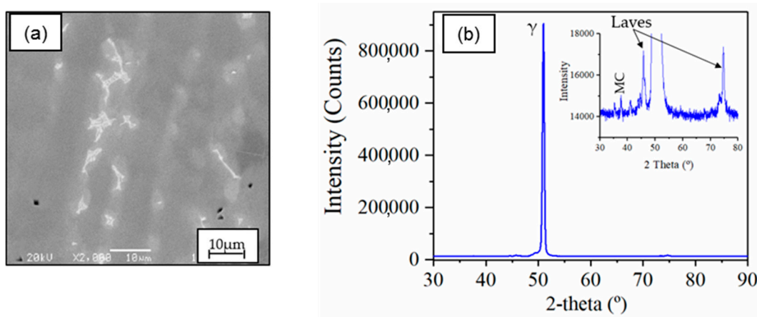
Figure 11. (a) the microstructure and corresponding (b) XRD pattern of WAAM IN718.
