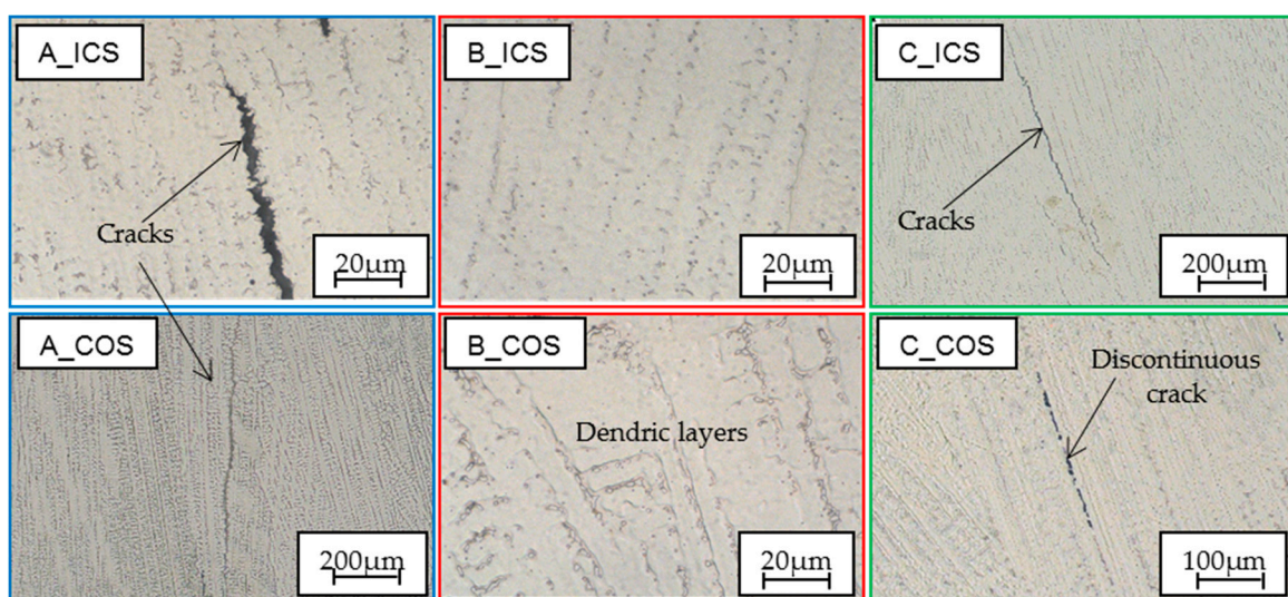
Figure 10. Micrograph of dendritic structure for the ICS and COS samples.
