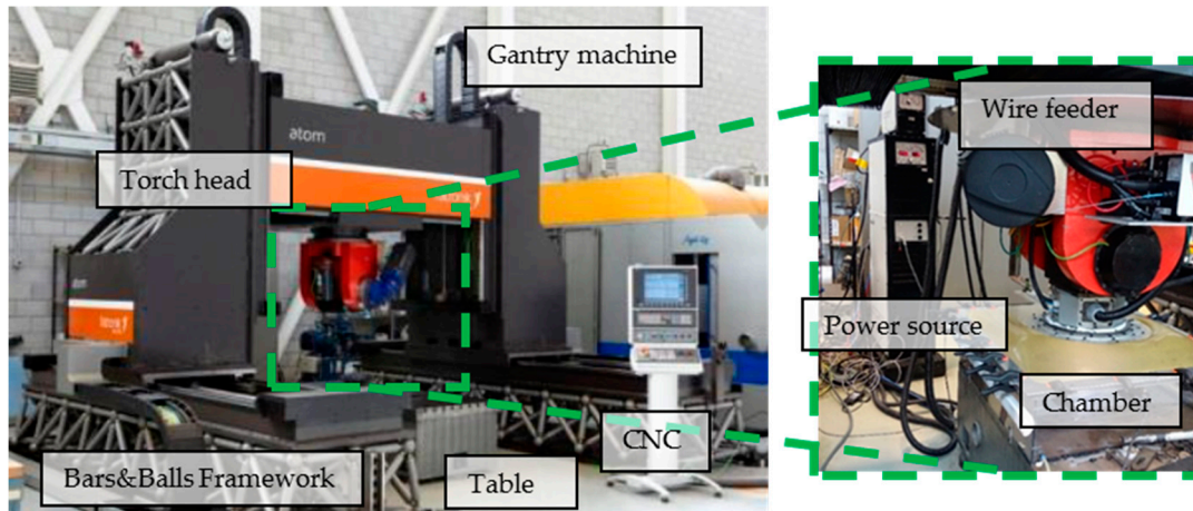
Figure 1. Shaft gantry machine with EWM welding equipment.
