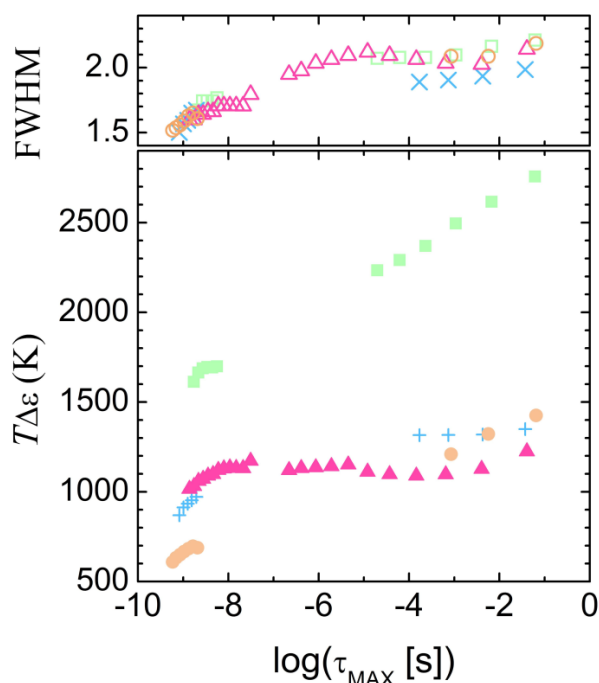
Figure 5. Relaxation strength ( T\Delta\varepsilon ) and FWHM as a function of the relaxation time ( \tau_{MAX} ). Solid symbols correspond to: ■ PTF, + PBF, ▲ PPeF, ● PHF. Empty symbols show the FWHM data: □ PTF, × PBF, △ PPeF, ○ PHF.
