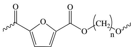
Scheme 1. Chemical structure of the investigated poly(alkylene 2,5-furanoate)s. n refers to the number of methylene groups: 3, 4, 5 and 6 for PTF, PBF, PPeF and PHF, respectively.
