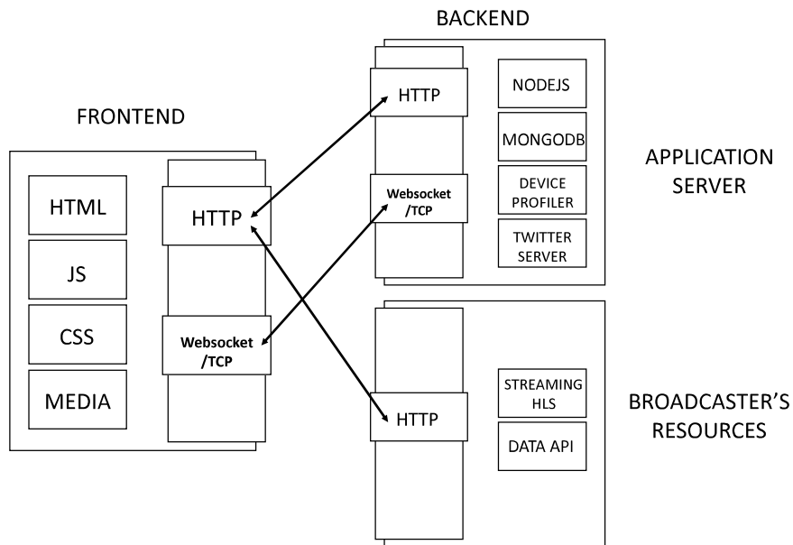
Figure 3.2: Service implementation
