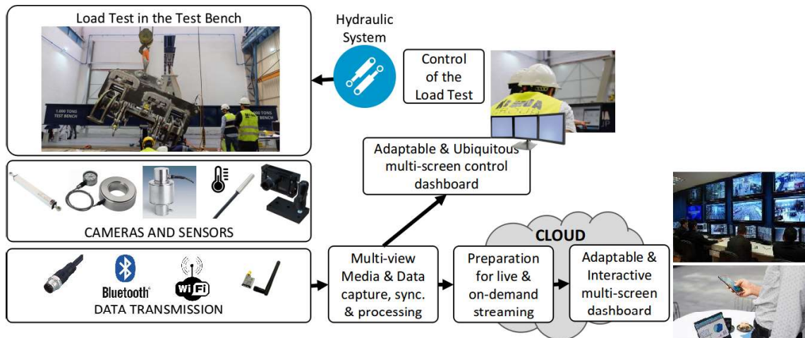
Figure 5.3: Dynamic multiscreen dashboards for operators in Industry 4.0
