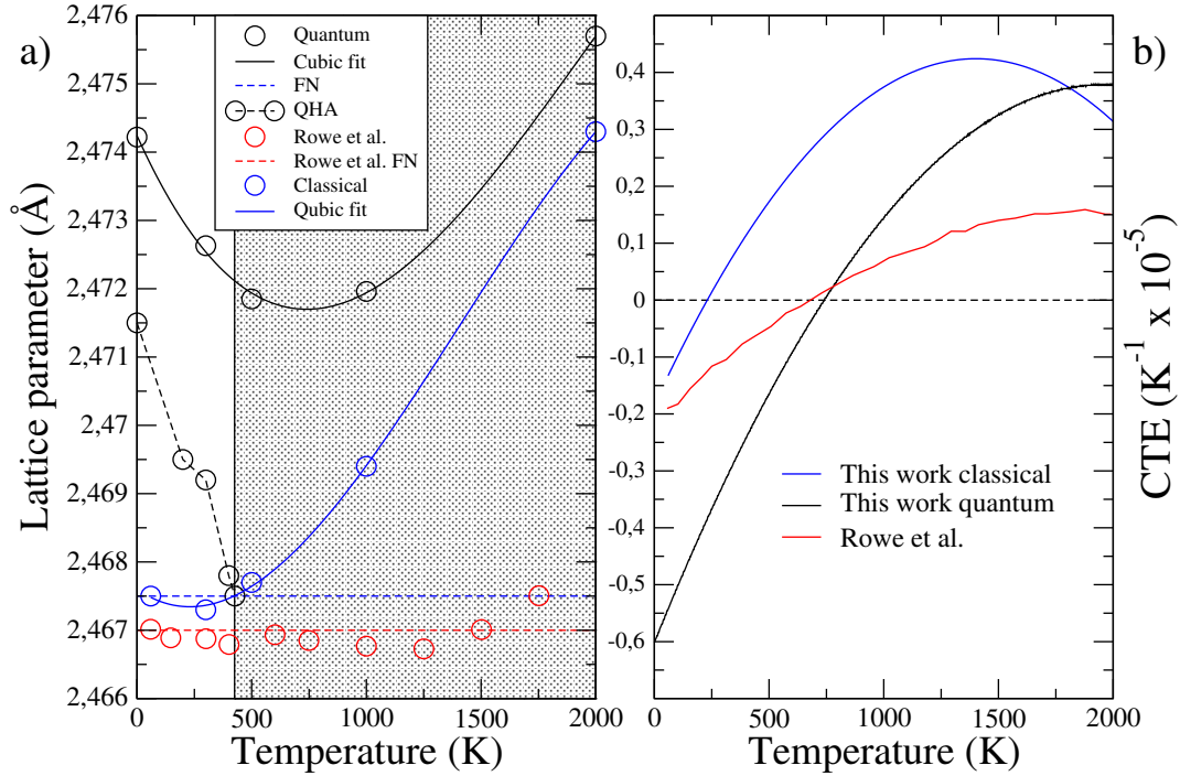
FIGURE 8.7: (a) Lattice parameter of graphene as a function of temperature obtained with the SSCHA using a machine learning atomistic potential. Both quantum (black) and classical (blue) calculations are included. The classical result is calculated setting \hbar = 0 in the SSCHA free energy. The temperature-independent frozen nuclei (FN) result corresponds to the lattice parameter that minimizes the Born Oppenheimer potential U . Results obtained by Rowe et al.[163] are also included for comparison. Solid black and blue lines correspond to cubic fits. The black dashed line corresponds to the quasiharmonic result (QHA). (b) Thermal expansion coefficient (CTE) calculated as CTE = \frac{1}{A} \frac{\partial A}{\partial T} , A being the area of the membrane. Red line is directly taken from [163]. Black and blue lines are calculated using the cubic fits in (a).
