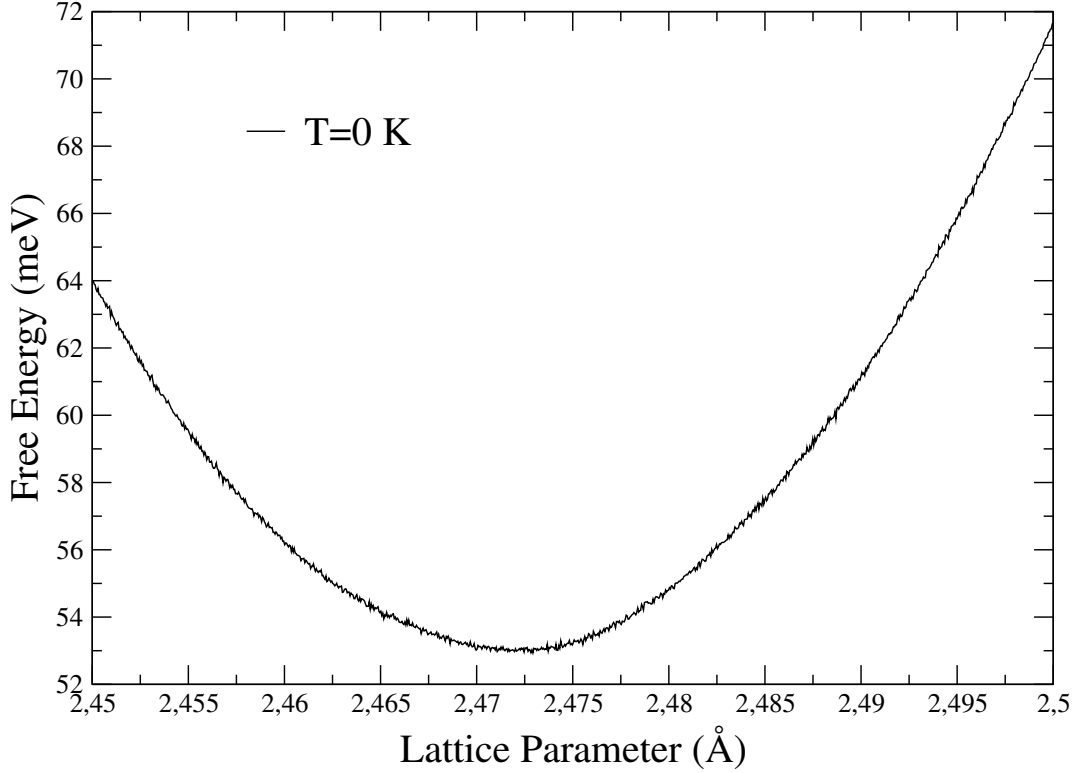
FIGURE 8.11: Quasiharmonic free energy of graphene at 0 K.
