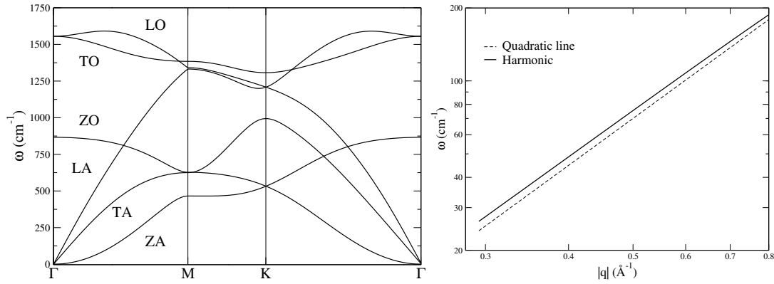
FIGURE 8.2: Left: Harmonic phonon spectrum of graphene. Right: Harmonic ZA phonon dispersion of graphene in logarithmic scale. We include a quadratic line for reference.
