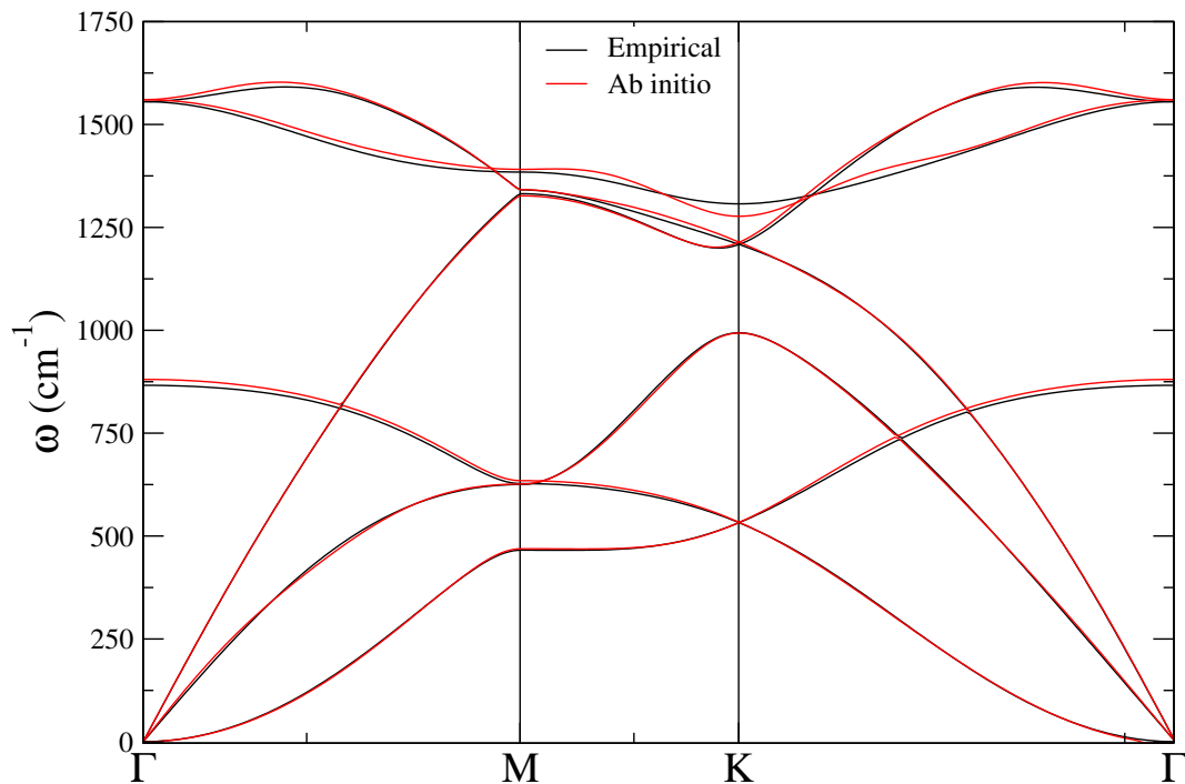
FIGURE 8.4: Harmonic phonon spectrum of graphene calculated with the empirical potential and ab initio . The calculations are done in a 6 \times 6 supercell.
