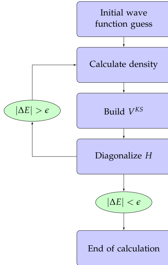
FIGURE 2.1: Flowchart of the self-consistent cycle for solving the Kohn-Sham equation. \Delta E and \epsilon are the energy difference between current cycle and the previous and the chosen threshold, respectively.
