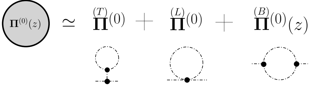
FIGURE 3.3: Diagrammatic representation of the self-energy and Feynman diagrams for the tadpole, loop, and bubble self-energies. The dashed line corresponds to the harmonic phonons and dots represent the interaction vertices. Within perturbation theory at the lowest-order there are third and fourth-order vertices, which means that there are three and four phonon interactions.
