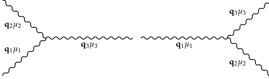
FIGURE 4.3: Feynman diagrams for three phonon scattering events. The one in the left corresponds to P_{\mathbf{q}_1\mu_1, \mathbf{q}_2\mu_2}^{\mathbf{q}_3\mu_3} , where two phonons collide ( \mathbf{q}_1\mu_1, \mathbf{q}_2\mu_2 ) to create a new one ( \mathbf{q}_3\mu_3 ), and the one in the right corresponds to P_{\mathbf{q}_1\mu_1}^{\mathbf{q}_2\mu_2, \mathbf{q}_3\mu_3} , where one phonon ( \mathbf{q}_1\mu_1 ) is splitted in two phonon modes ( \mathbf{q}_2\mu_2, \mathbf{q}_3\mu_3 ).
