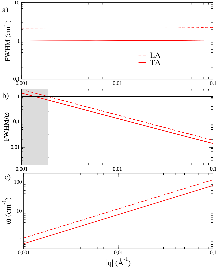
FIGURE 8.3: (a) Linewidths (full width at half maximum, FWHM) of the LA and TA modes calculated using perturbation theory at 300 K. (b) FWHM divided by the phonon frequency. We shadow the region where FWHM/\omega > 1 . All the calculations are done in the membrane model in Eq. 8.1. (c) LA and TA harmonic frequencies within the membrane model.
