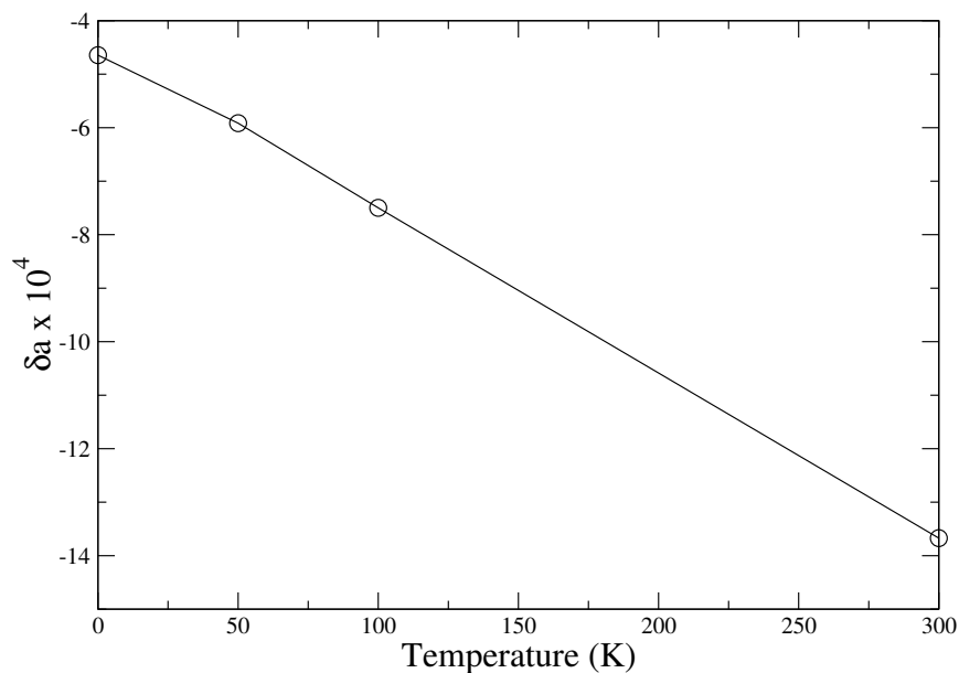
FIGURE 8.17: \delta a as a function of temperature in the membrane model.
