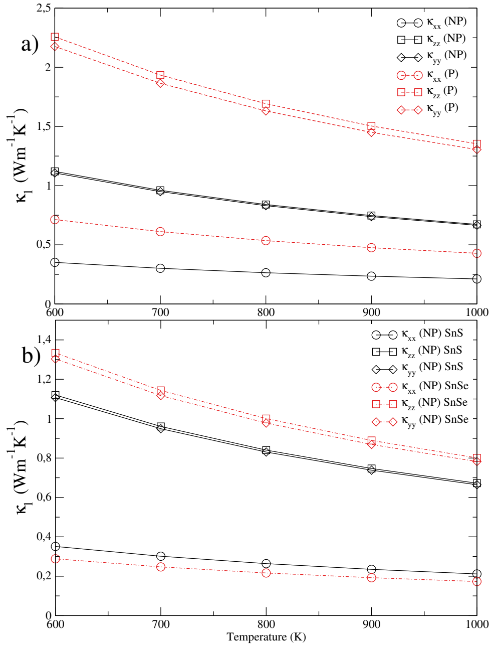
FIGURE 6.4: (a) Lattice thermal conductivity of Cmcm SnS calculated within nonperturbative (NP) and perturbative (P) approaches. We have used \Omega_{\mu}^{(S)}(\mathbf{q}) at 800 K for both and SSCHA 3BFCs at 800 K for the calculation in both cases. Calculations are within the LDA. (b) Lattice thermal conductivity of Cmcm SnS and SnSe calculated within the nonperturbative (NP) approach.
