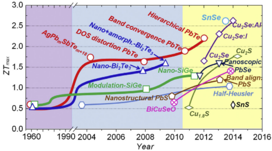
FIGURE 1: Record ZT materials as a function of the year. The figure is taken from reference[5].
