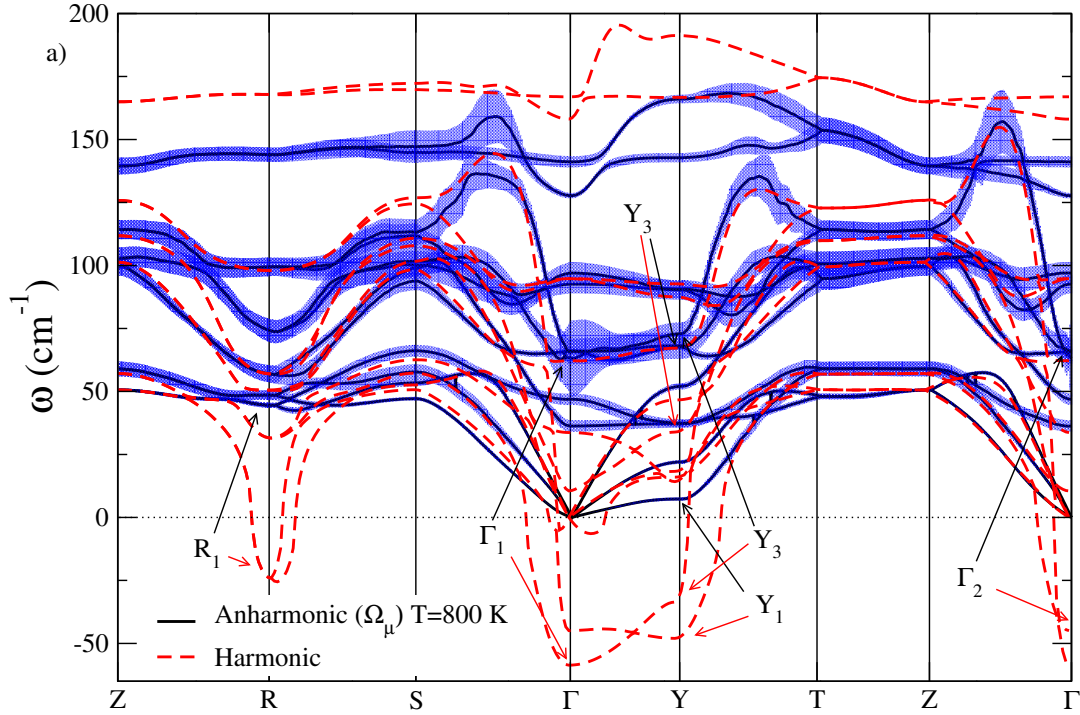
FIGURE 5.8: Harmonic and anharmonic phonons in the Lorentzian approximation ( \Omega_\mu(\mathbf{q}) ). The length of the bars corresponds to the linewidth (full length of the line is the full width at half maximum divided by a factor of 1.5). The calculations are done within LDA in the experimental structure using SSCHA 3BFC at 800 K and \Omega_\mu^{(S)}(\mathbf{q}) at 800 K.
