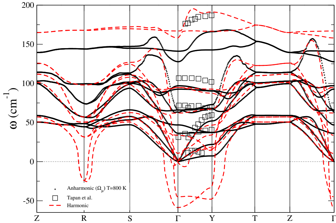
FIGURE 5.9: Harmonic and anharmonic phonons in the Lorentzian approximation ( \Omega_\mu(\mathbf{q}) ). We include experimental points [113] at 853 K.
