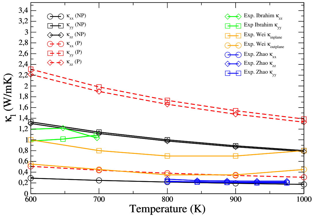
FIGURE 5.12: Lattice thermal conductivity of SnSe calculated with perturbative (P) and nonperturbative (NP) at 800 K compared to the experiments by Ibrahim et al.[115], Zhao et al.[6], and Wei et al.[127]. We use the \Omega_{\mu}^{(S)}(\mathbf{q}) phonon frequencies calculated at 800 K at all temperatures. Calculations are performed within LDA using the experimental structure.
