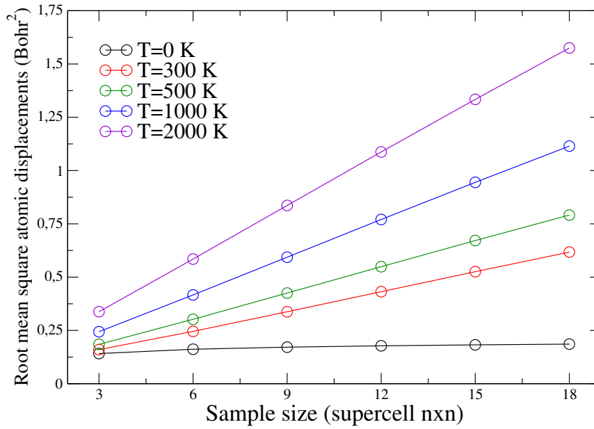
FIGURE 8.1: Root mean square atomic displacements of carbon atoms in graphene calculated using the harmonic dispersion as a function of the supercell size for different temperatures. The calculation is done by using the harmonic formula for \langle u^2 \rangle [40].
