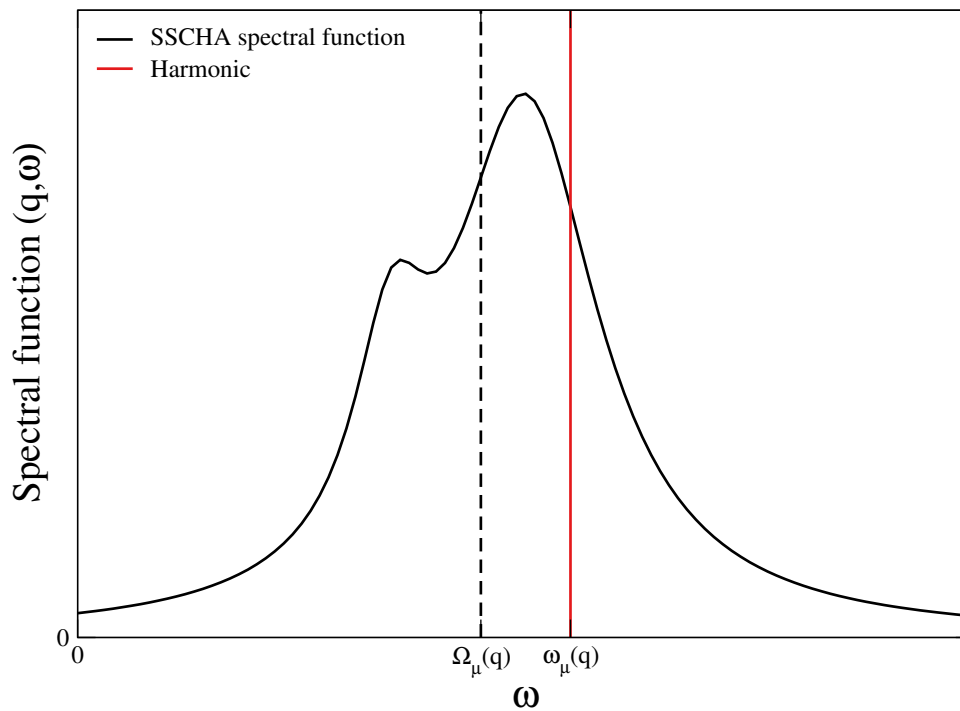
FIGURE 3.9: SSCHA and harmonic spectral functions where the Lorentzian approximation does not hold.
