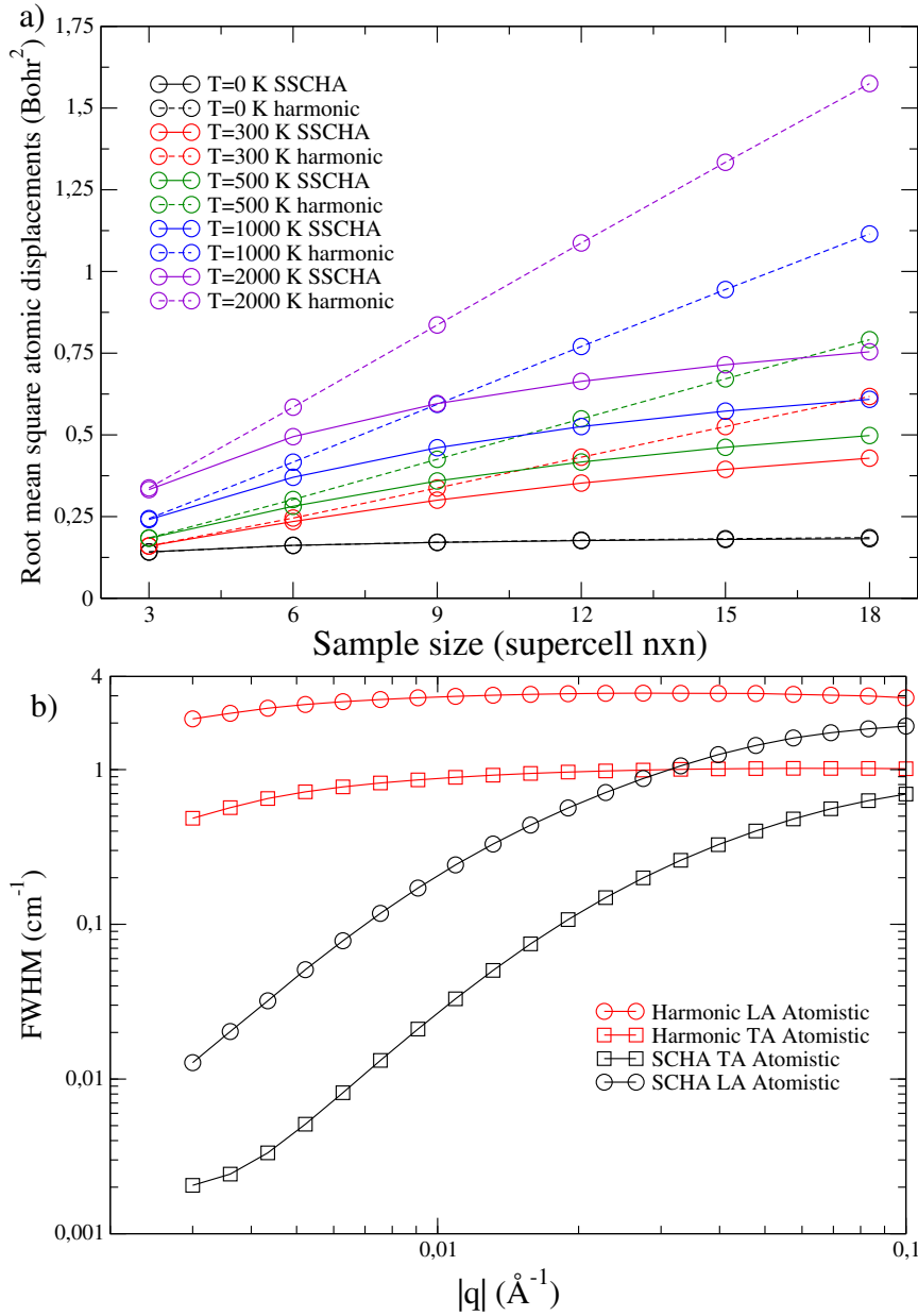
FIGURE 8.15: (a) Root mean square atomic displacement of carbon atoms in graphene calculated using the harmonic and the SSCHA density matrices. The harmonic result is always computed at the lattice parameter that minimizes U , while the SSCHA results include thermal expansion (see Fig. 8.7). (b) Linewidths (full width at half maximum) of LA and TA phonon modes at 300 K calculated within perturbation theory and the SSCHA. Results in both figures are obtained with the machine learning atomistic potential.
