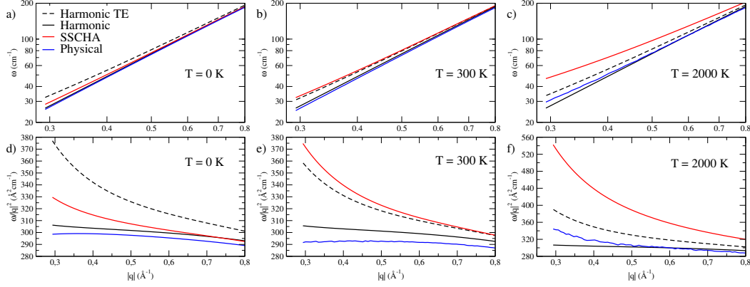
FIGURE 8.12: Harmonic ZA phonon spectra in logarithmic scale together with the SSCHA phonons, D^{(S)} , (labeled as “SSCHA”) and those obtained from the phonon spectral function, \Omega_\mu(\mathbf{q}) , (labeled as “Physical”). Results at 0 K (a), 300 K (b), and 2000 K (c) are shown. (d), (e) and (f) show the frequency divided by the squared momentum. The dispersion corresponds to the \Gamma M direction. For reference, the M point is at 1.4662 \text{ \AA}^{-1} at 0 K, at 1.4671 \text{ \AA}^{-1} at 300 K, and at 1.4652 \text{ \AA}^{-1} at 2000 K. The harmonic result (solid black) is computed at the lattice parameter that minimizes U , while the other results include thermal expansion (see Fig. 8.7). The dashed black lines correspond to harmonic calculations including thermal expansion (TE). All these calculations are performed with the machine learning atomistic potential.
