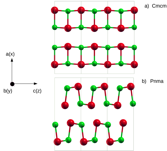
FIGURE 5.1: SnSe crystal structure in the (a) Cmcm and (b) Pnma phases.
