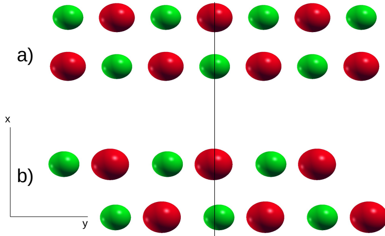
FIGURE 7.1: Monolayer SnSe crystal structure in the (a) Pnmm (high symmetry) and (b) Pnm2_1 (low symmetry) phases.
