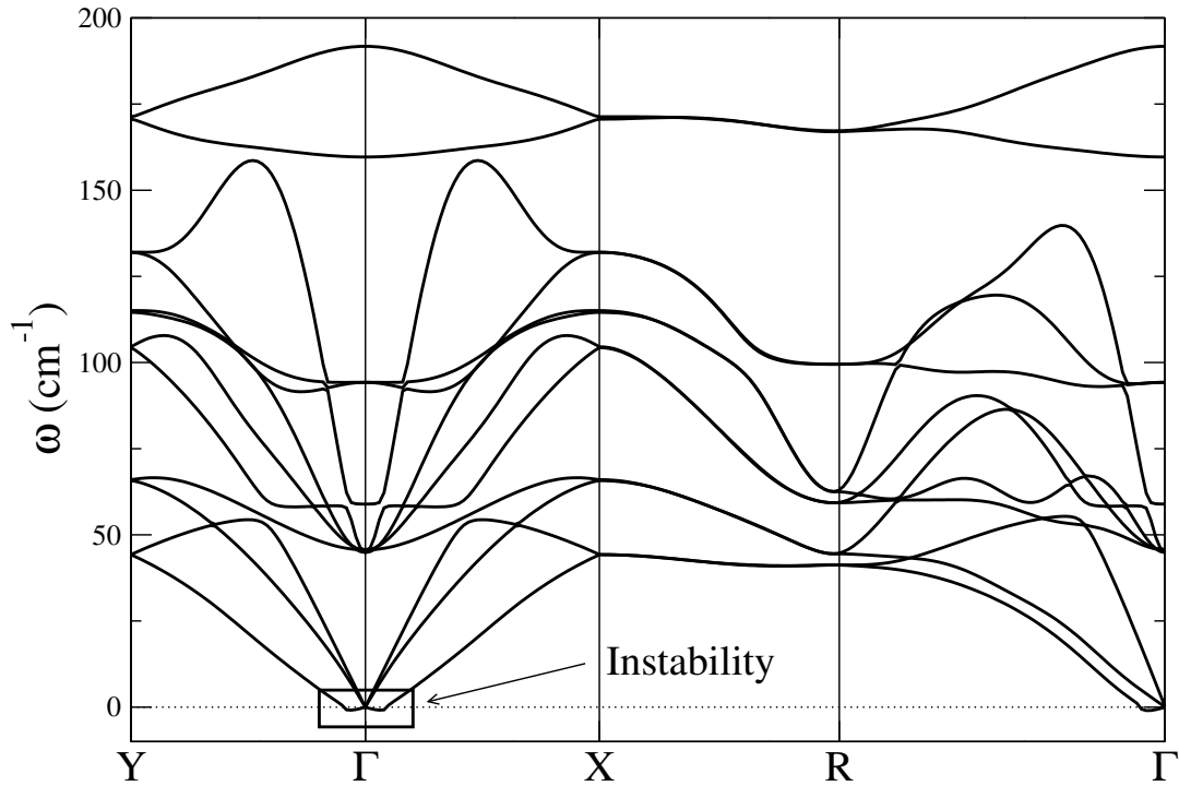
FIGURE 7.5: \Omega_{\mu}^{(S)}(\mathbf{q}) phonon spectrum at 300 K within PBE using the theoretical lattice parameters.
