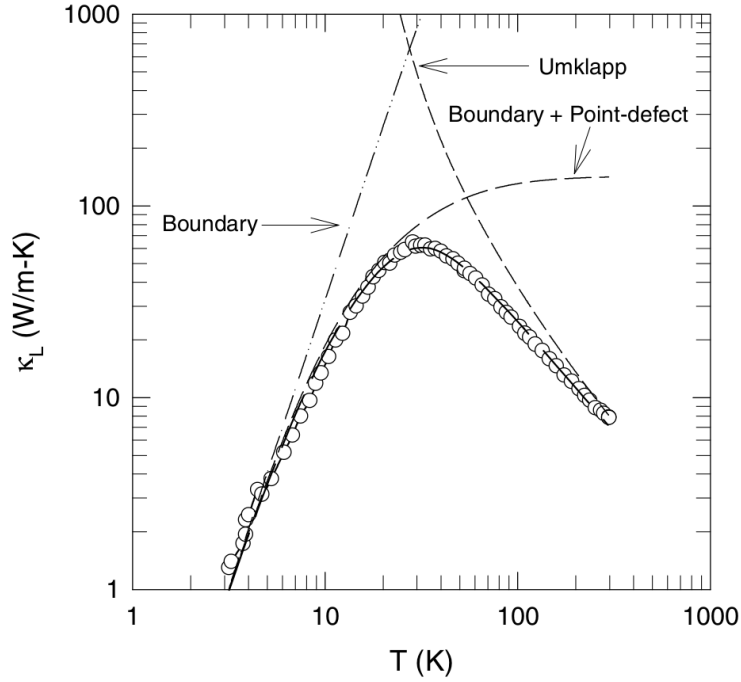
FIGURE 4.2: Experimental thermal conductivity of CoSb_3 [94] as a function of temperature and theoretical fitting with different power laws corresponding to different scattering mechanisms.
