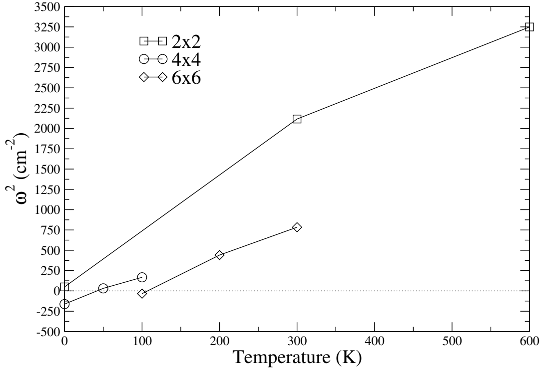
FIGURE 7.4: \Omega_{\Gamma_1}^{(F)2} as a function of temperature within PBE using the theoretical lattice parameters. We show the calculation for the 2 \times 2 , 4 \times 4 , and 6 \times 6 supercells.
