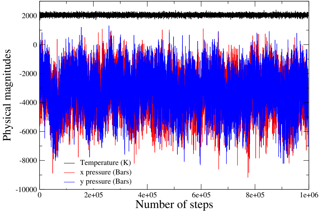
FIGURE 8.9: Temperature and in-plane pressure Cartesian components as a function of the step number. Each steps corresponds to 0.001 ps. The Temperatures is in K and the pressure in Bars. The lattice parameter is fixed to 2.48 Å. The simulation is done in the microcanonical ensemble.
