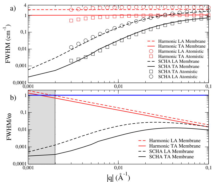
FIGURE 8.18: (a) Atomistic and membrane linewidths calculated within the SSCHA and within perturbation theory at 300 K. (b) Membrane linewidths at 300 K divided by the phonon frequency calculated within the SCHA and perturbation theory.
