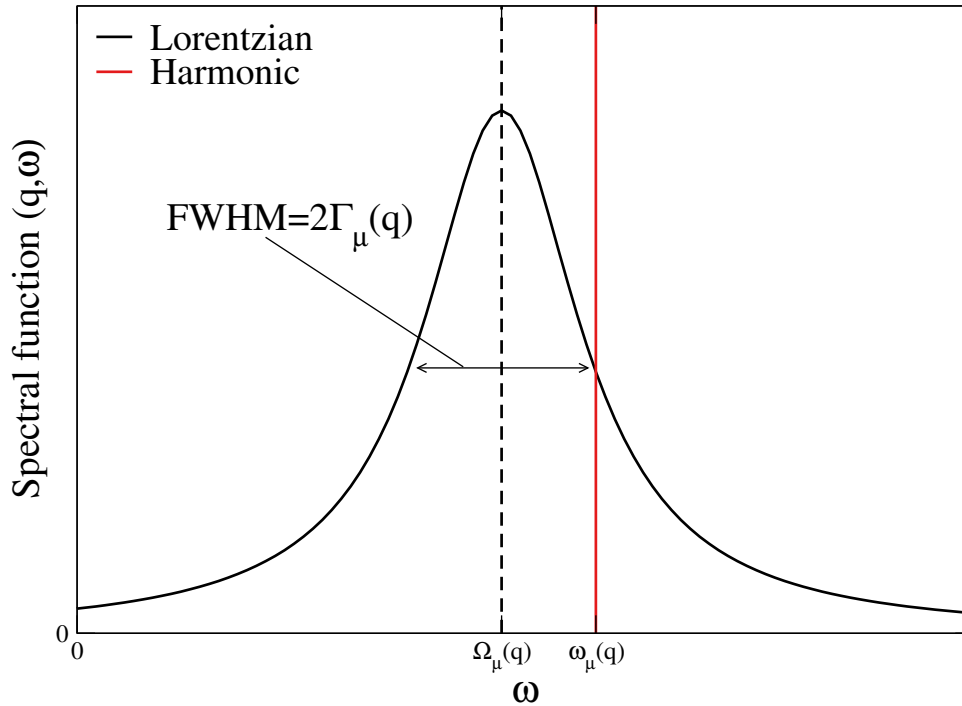
FIGURE 3.4: Lorentzian and harmonic spectral functions. The harmonic spectral function is a Dirac's delta. The Lorentzian has a well defined full width at half maximum (FWHM) and a well defined energy \Omega_\mu(q) .
