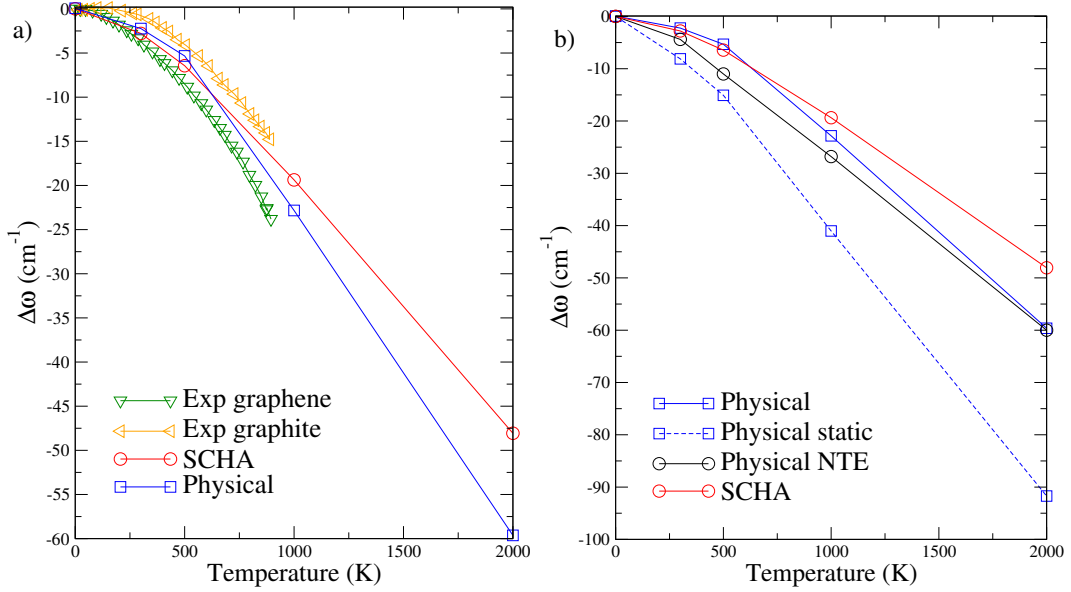
FIGURE 8.14: (a) SCHA and physical E_{2g} phonon frequency shift as a function of temperature. We include experimental results in graphene[168] and graphite[169, 170]. (b) The same as (a) without experiments and including the physical phonons without thermal expansion (Physical NTE) and the physical static phonons.
