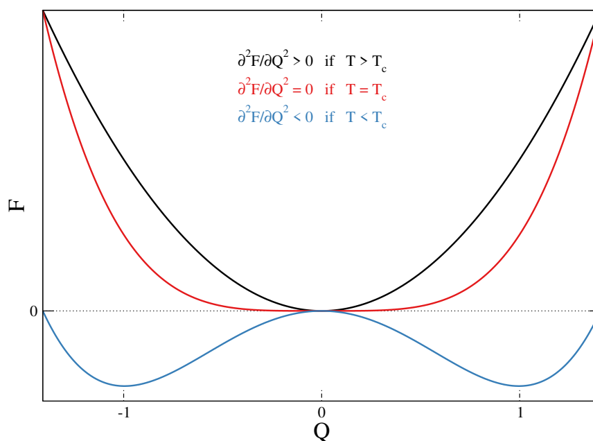
FIGURE 3.7: Free energy as a function of the order parameter for three different temperatures in a system with a second-order phase transition. The blue line corresponds to a temperature below the critical temperature, the red line to the critical temperature and the black line to a temperature above the critical temperature.
