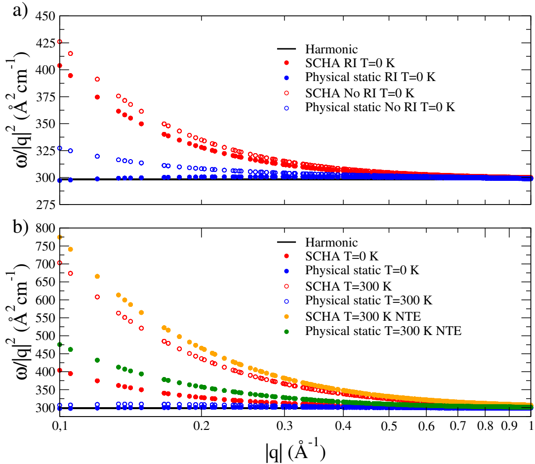
FIGURE 8.16: (a) Frequency of the ZA mode divided by the squared momentum in the harmonic approximation, within the SCHA and obtained from the Hessian of the SCHA (labeled as “Physical static”) at 0 K in the membrane model. We name rotationally invariant (RI) the results considering the full potential in Eq. 8.1. We name no rotationally invariant (No RI) the results neglecting the last three terms in Eq. 8.1. (b) Frequency of the ZA mode in the harmonic approximation, within the SCHA and obtained from the Hessian of the SCHA at 0 K and 300 K in the membrane model. We also include the SCHA and physical phonons at 300 K without considering thermal expansion (NTE).
