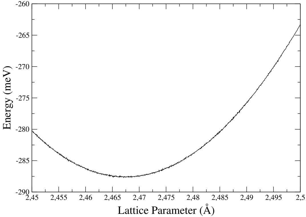
FIGURE 8.8: Graphene total energy U as a function of the lattice parameter.
