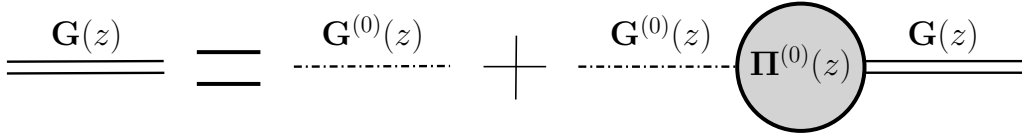
FIGURE 3.2: Diagrammatic representation of the Dyson equation in Eq. 3.43. The dashed line corresponds to the harmonic propagator. The double solid line corresponds to the full propagator.
