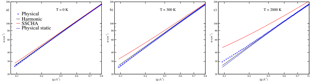
FIGURE 8.13: Harmonic, SSCHA, and physical phonons (static and dynamic) calculated at 0 K (a), 300 K (b), and 2000 K (c).
