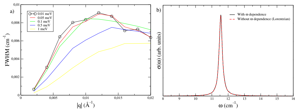
FIGURE 8.19: (a) SCHA Linewidth (full width at half maximum, FWHM) contribution of the term containing the fourth-order tensor of the LA mode calculated in the membrane model at 100 K. The value of the smearing is in the legend. (b) Spectral function of the LA mode with momentum 0.01 \text{\AA}^{-1} at 100 K with and without considering the frequency dependence of the self energy.
