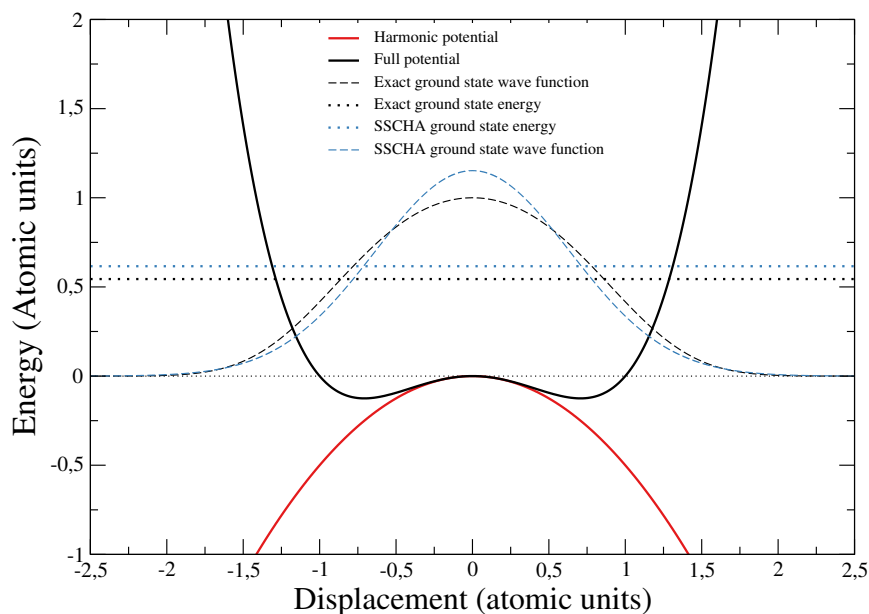
FIGURE 3.6: One dimensional example of the SSCHA with atomic units for energy and displacement. The actual potential and the harmonic one are the black and red solid curves, respectively. The ground state SSCHA at zero temperature and exact wave functions are shown with dashed curves. Dotted lines show the energy of each ground state wave function.
