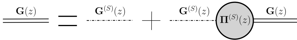
FIGURE 3.8: Diagrammatic representation of the Dyson equation got with a dynamical ansatz within the SSCHA. The dashed line corresponds to the SSCHA propagator. The double solid line corresponds to the full propagator.
