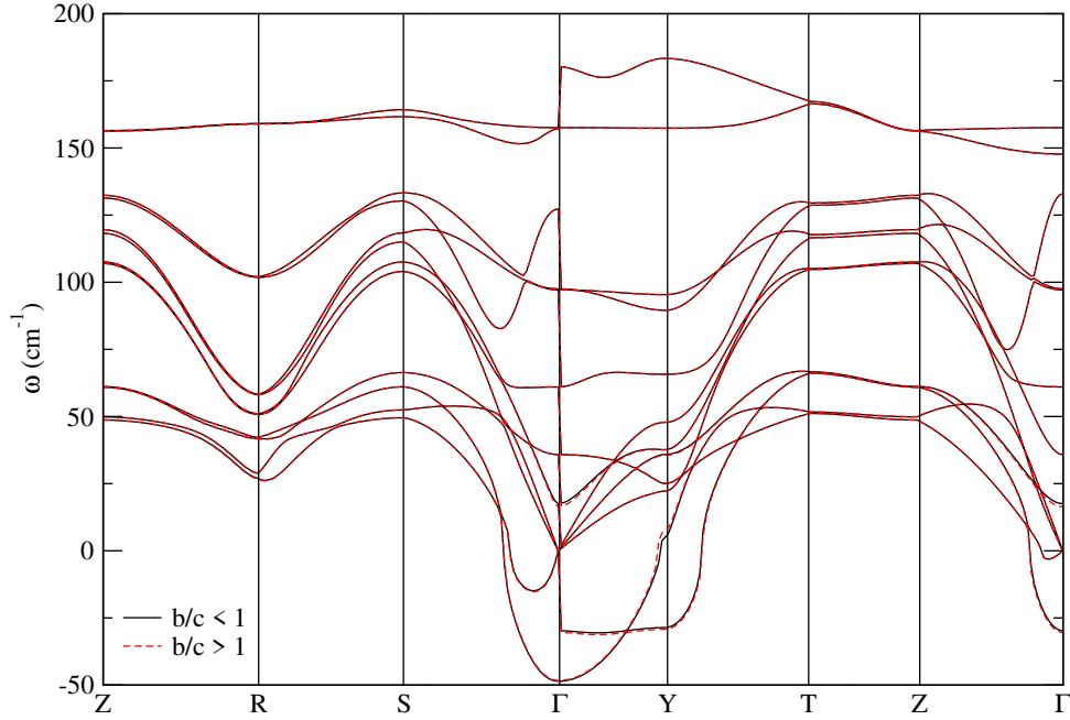
FIGURE 5.6: PBE harmonic phonon spectra with the following lattice parameters: a = 22.492 , b = 8.094 and c = 8.090 (in Bohr units) (red) in one case and exchanging b and c (black) in the other. We have done the calculation in a 2 \times 2 \times 2 supercell and Fourier interpolated to plot the spectrum. The effective charges are included in the calculations.
