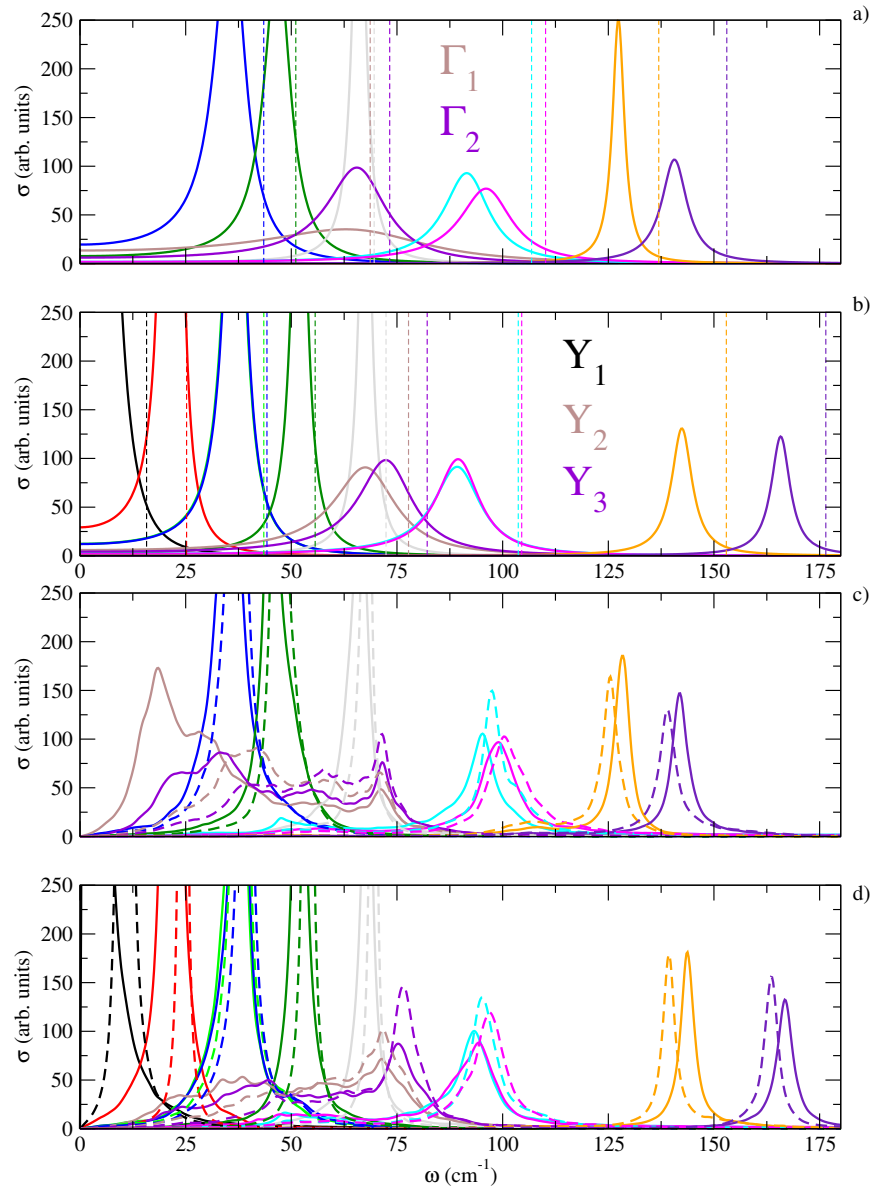
FIGURE 5.11: (a) Nonperturbative spectral functions calculated in the Lorentzian approximation at the \Gamma point. (b) The same as (a) at the point Y. Dashed vertical lines correspond to \Omega_\mu^{(S)} frequencies. (c) Nonperturbative (solid lines) and perturbative (dashed lines) spectral functions calculated at the \Gamma point. (d) The same as (c) at the point Y. The calculations are done using \Omega_\mu^{(S)} SSCHA frequencies at 800 K within LDA in the experimental structure. Nonperturbative calculations are done with 3BFC at 800 K.
