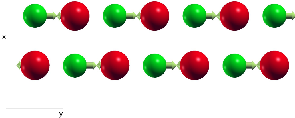
FIGURE 7.2: Distortion pattern associated to the \Gamma_1 mode.
