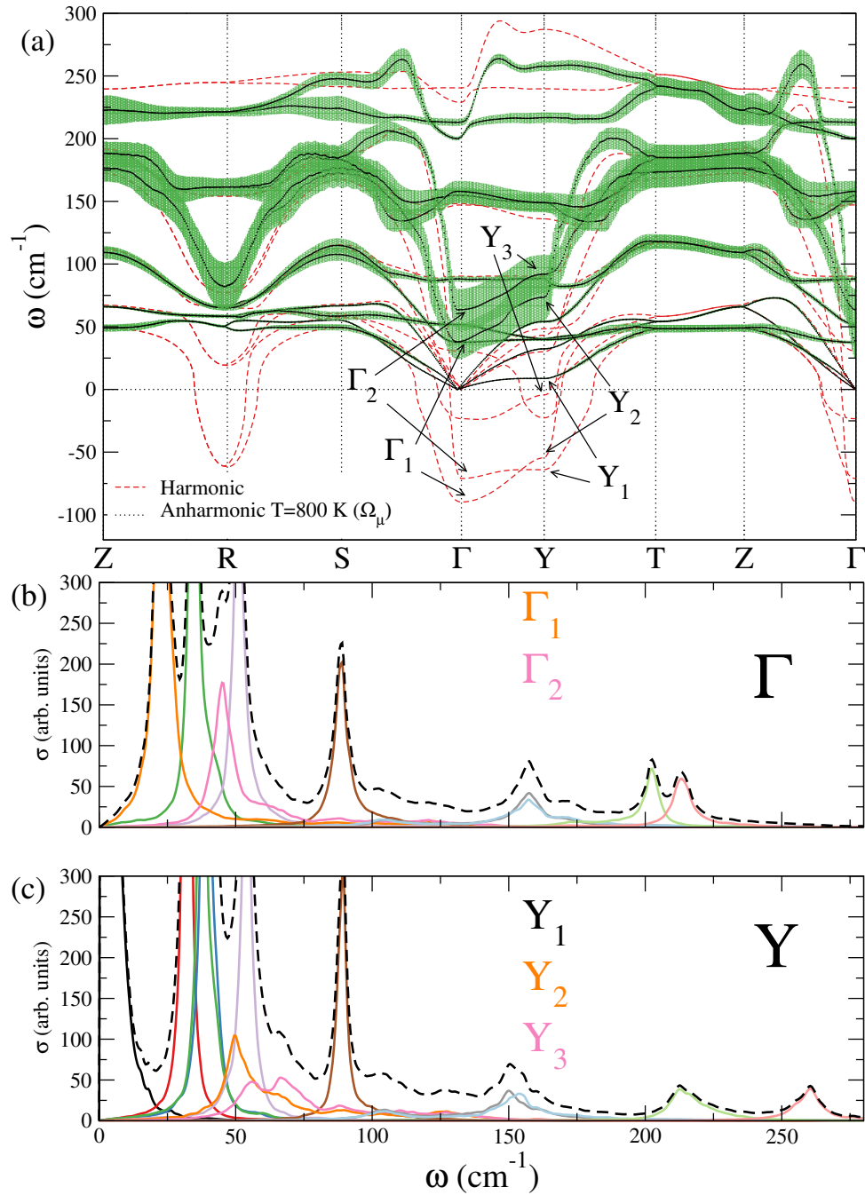
FIGURE 6.3: (a) Harmonic and anharmonic [\Omega_\mu(\mathbf{q})] phonon spectra within the Lorentzian approximation. The length of the bars corresponds to the linewidth (full length of the line is the half width at half maximum). The calculations are done within the LDA using SSCHA 3BFCs at 800 K and \Omega_\mu^{(S)}(\mathbf{q}) at 800 K. (b) and (c) \tilde{\sigma}(\omega) spectral functions at the points \Gamma and Y , respectively. Solid lines correspond to individual modes and dashed lines are the total spectral functions.
