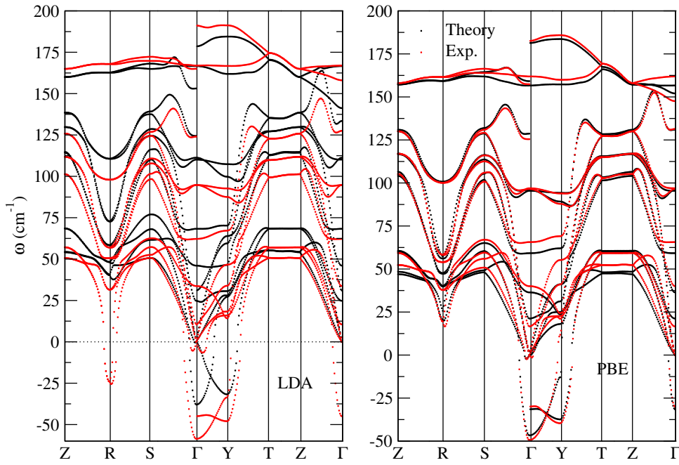
FIGURE 5.7: (a) LDA harmonic phonon spectra in the theoretical and experimental structures. (b) The same as (a) within PBE. The effective charges are included in the calculations.
