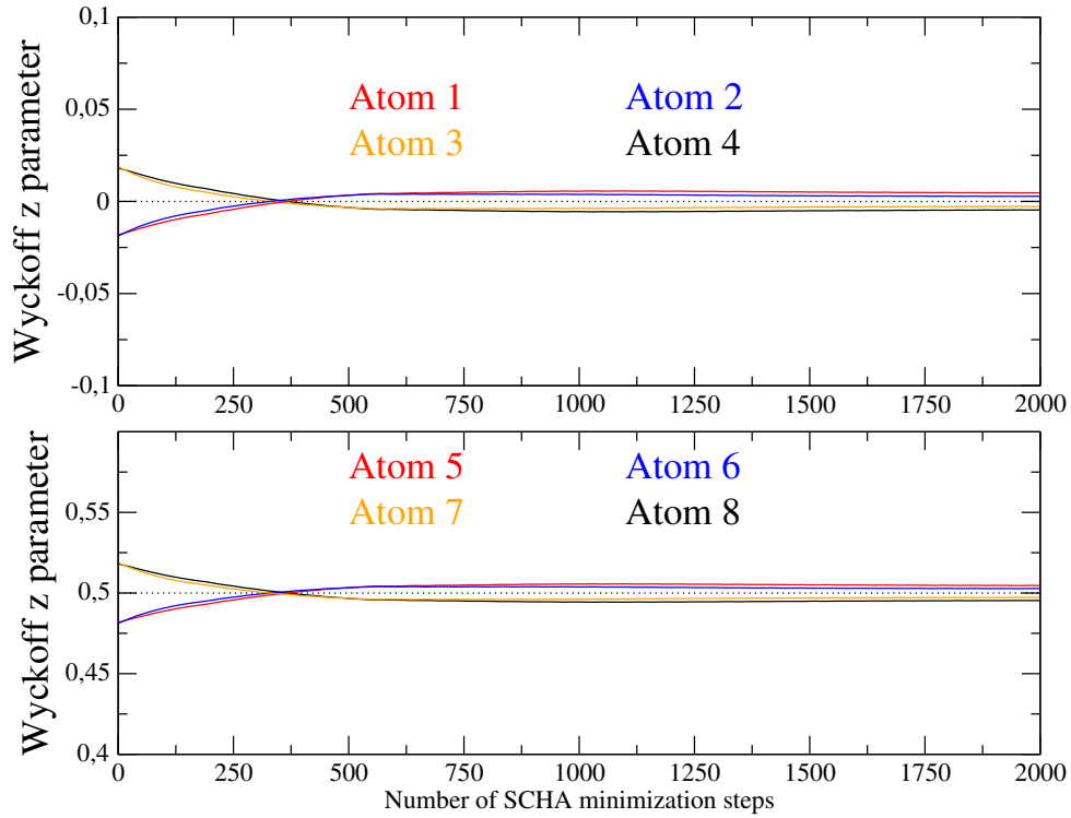
FIGURE 5.5: Wyckoff z parameter of the 4c Wyckoff position in the Pnma phase as a function of the SSCHA minimization step. Each color corresponds to a different atom in a given high symmetry position in the Cmcm phase.
