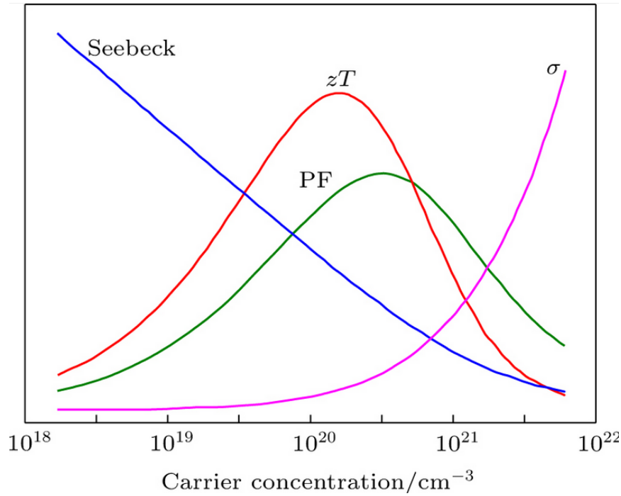
FIGURE 2: Electrical conductivity and Seebeck coefficient as a function of the carrier concentration in a typical semiconductor.
