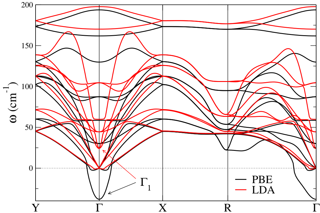
FIGURE 7.3: Harmonic phonons of monolayer SnSe in the Pnmm phase within the LDA and PBE approximations in the theoretical structure.
