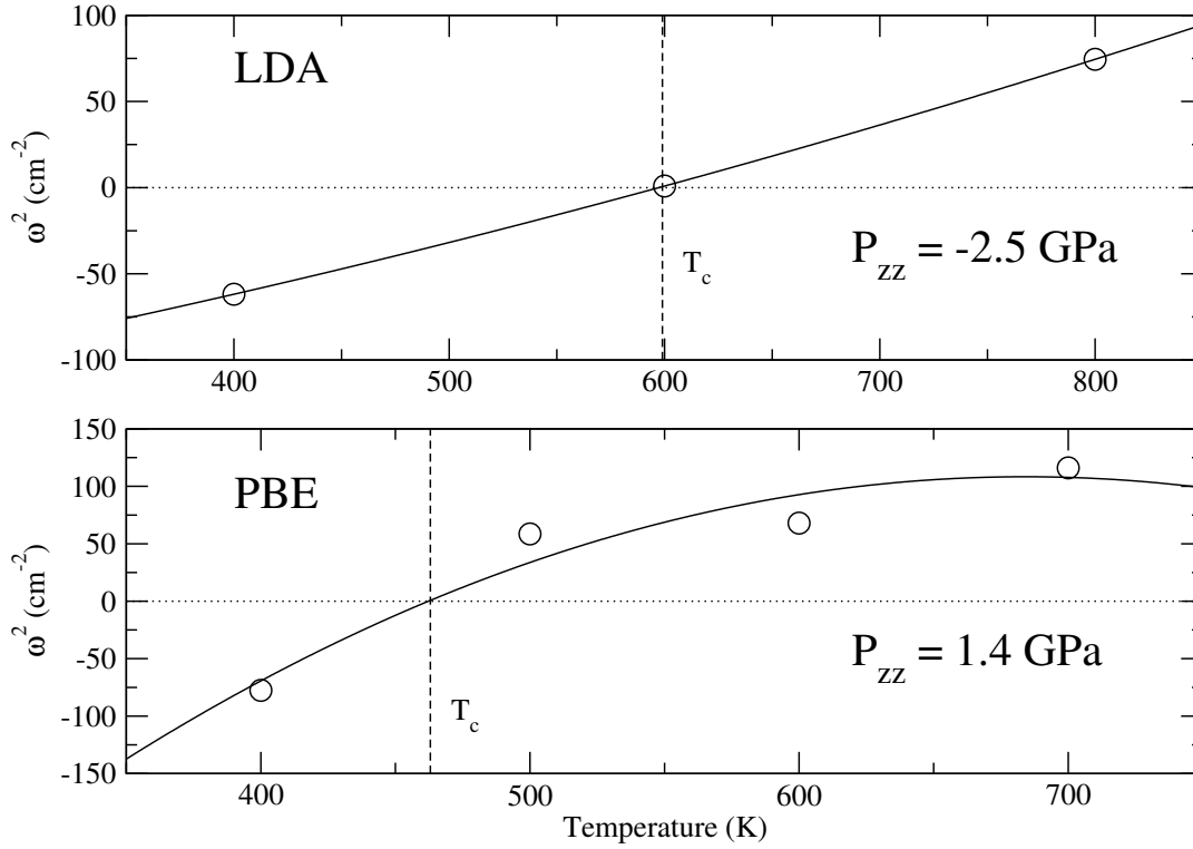
FIGURE 6.2: \Omega_{Y_1}^{(F)2} as a function of temperature within LDA and PBE approximations using the experimental lattice parameters (circles). The solid lines correspond to a polynomial fit. We include the pressure component P_{zz} , which is the pressure in the direction where the atoms move in the transition. This pressure is calculated including the anharmonic vibrational energy within the SSCHA.
