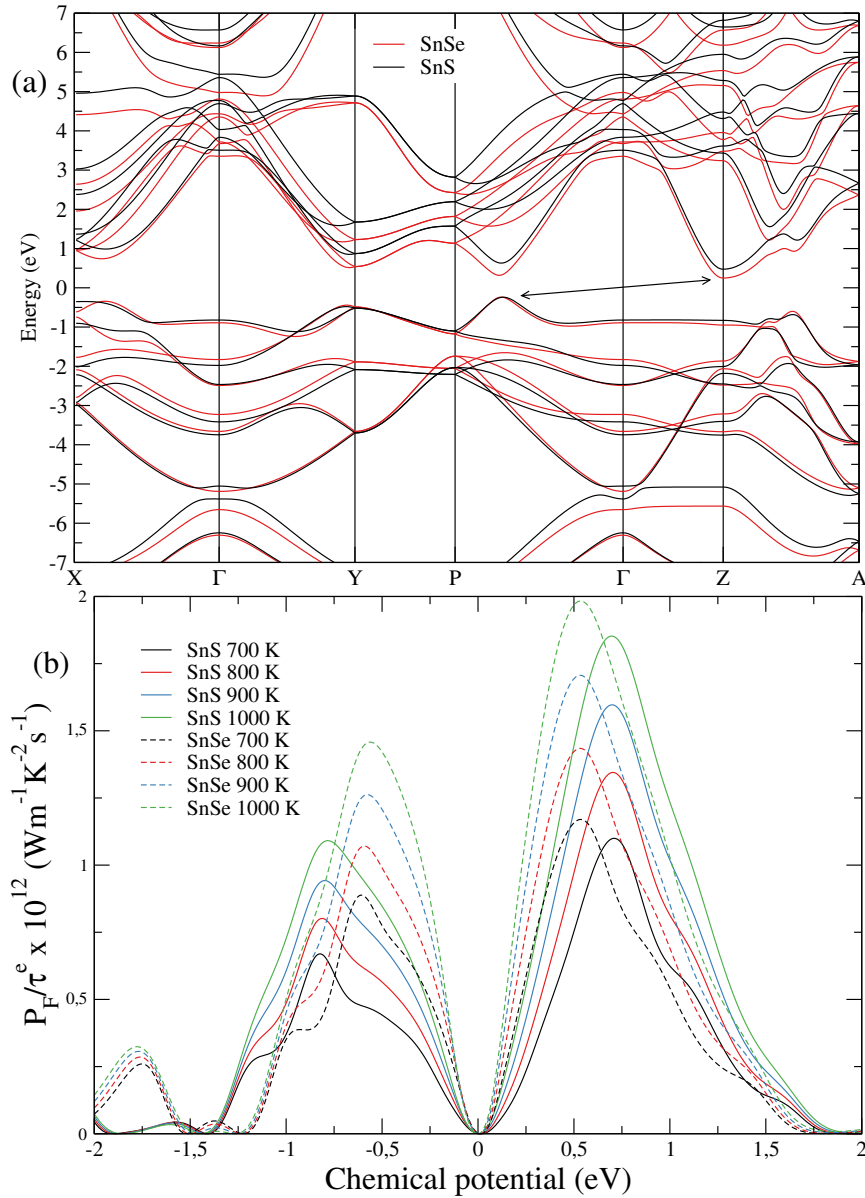
FIGURE 6.1: (a) Electronic band structure of Cmc m SnS and SnSe using experimental lattice parameters. (b) P_F/\tau^e of Cmc m SnS and SnSe for different temperatures as a function of the chemical potential. The 0 value corresponds to the middle of the gap in both figures.
