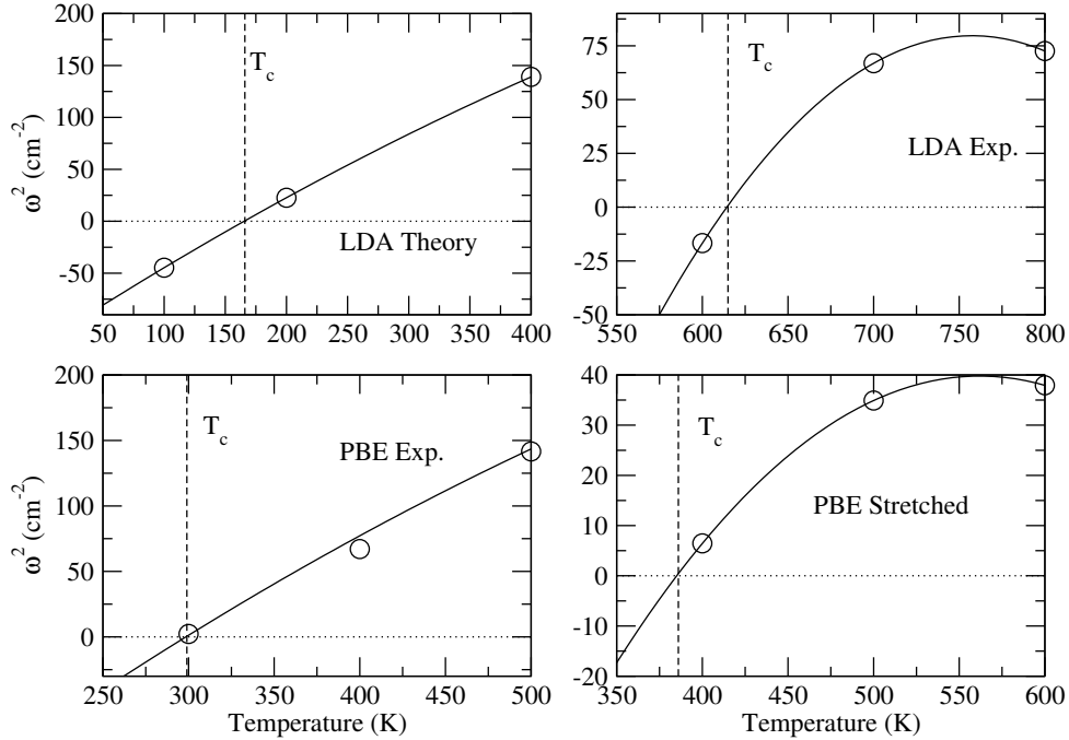
FIGURE 5.4: \Omega_{Y_1}^{(F)2} as a function of temperature within LDA and PBE approximations for different lattice volumes (circles). In the LDA we compare the results obtained with the theoretical and experimental[6] lattice parameters. In the PBE calculation we present the results for the experimental lattice parameters and a stretched unit cell (see Table 5.2 for the lattice parameters). The solid lines correspond to a polynomial fit.
