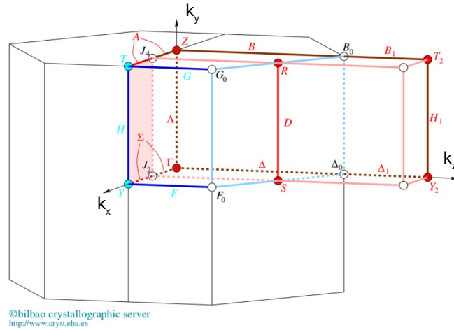
FIGURE 5.2: 1BZ of Cmcm SnSe. The figure is taken from the Bilbao crystallographic server.
