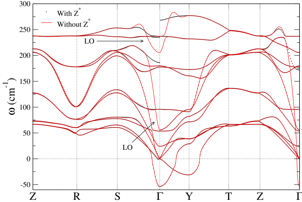
FIGURE 3.1: Ab initio phonon dispersion of SnS including the coupling of the longitudinal optic modes with the macroscopic electric field (black circles) and without including it (red lines). The LO modes are denoted with arrows.
