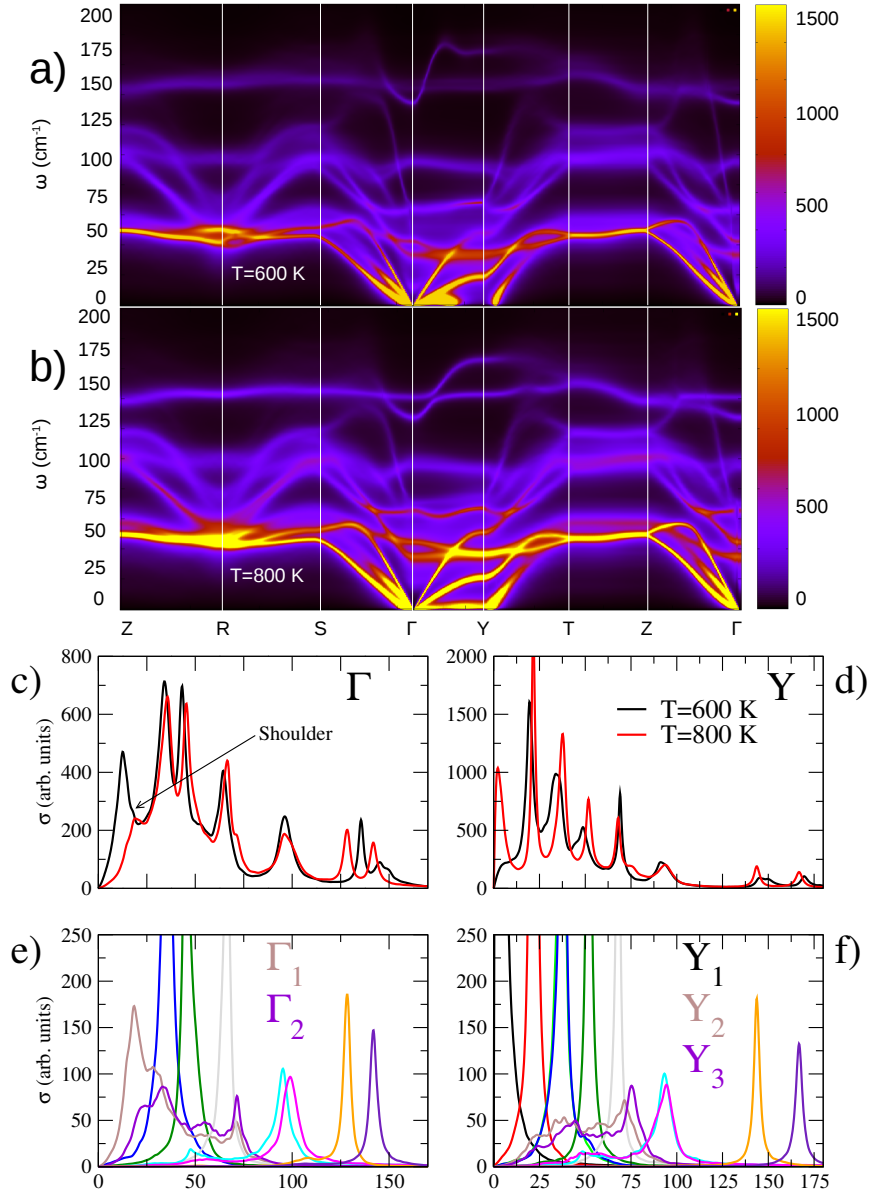
FIGURE 5.10: Spectral function of SnSe in the Cmc m phase calculated at (a) 600 K and (b) 800 K using the SSCHA 3BFC at the corresponding temperature. The spectral function at the (c) \Gamma and (d) Y points at 600 and 800 K. The contribution of each mode to the spectral function is also shown at the \Gamma point (e) and the Y point (f) at 800 K. Different colors correspond to different modes. All the calculations are performed within LDA in the experimental structure. In each case we use \Omega_{\mu}^{(S)}(\mathbf{q}) calculated at the same temperature as the SSCHA 3BFC.
