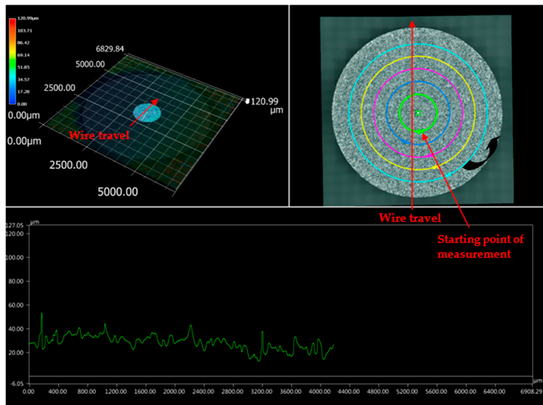
Figure 6. Surface analysis of machined sample at innermost periphery.
