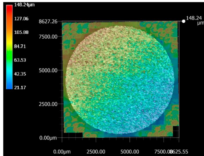
Figure 4. Machined surface representing surface roughness (SR) values for superelastic nitinol [22].
