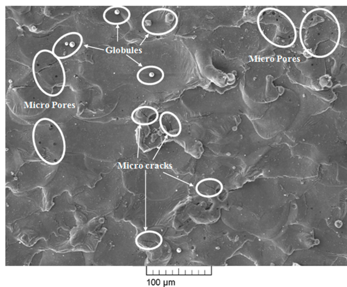
Figure 8. SEM micrograph at high discharge energy level.
