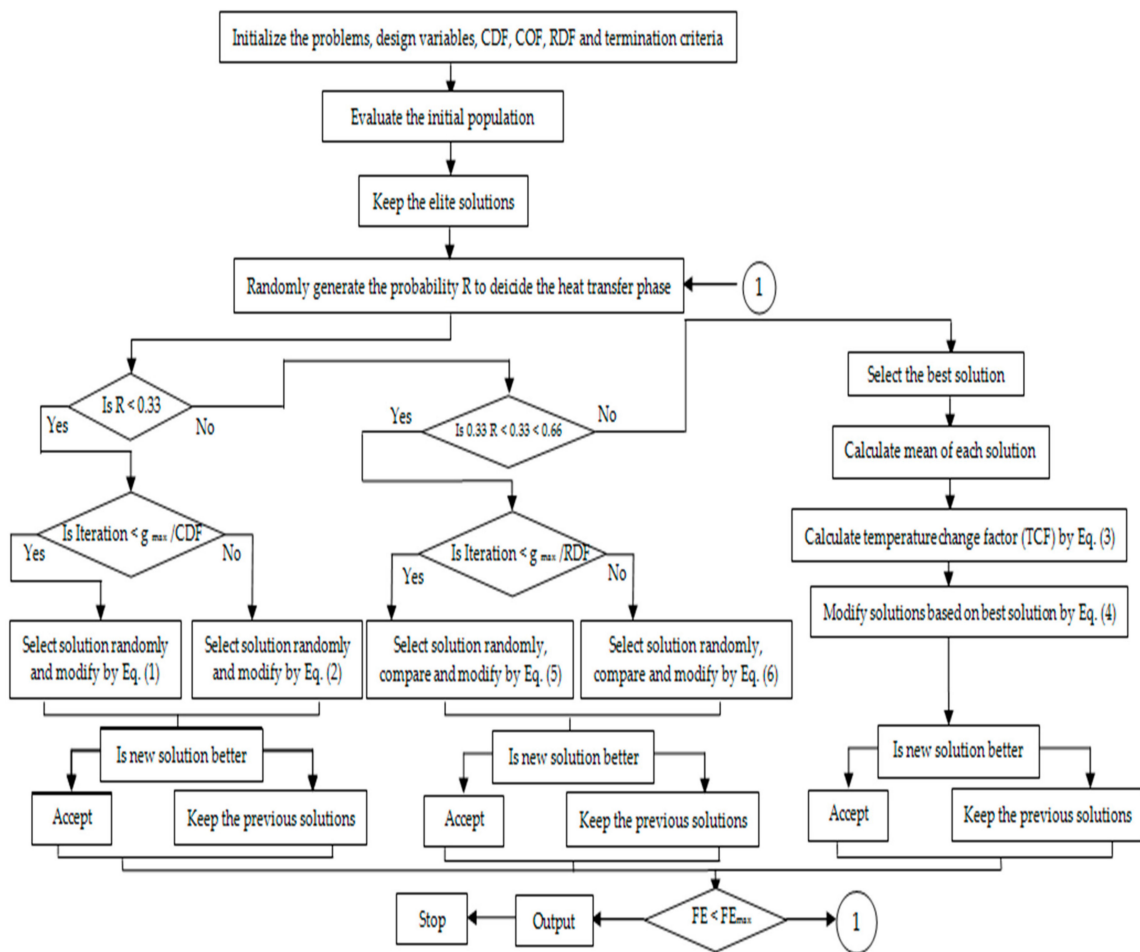
Figure 1. Flow chart of the heat transfer search (HTS) algorithm.
