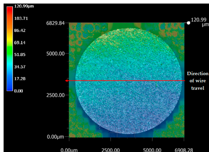
Figure 3. Surface machined under optimized process parameters.
