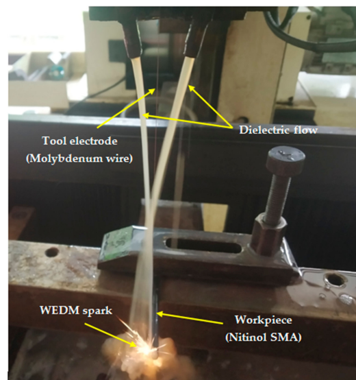
Figure 2. Flushing mechanism for the wire electrical discharge machining (WEDM) process.
