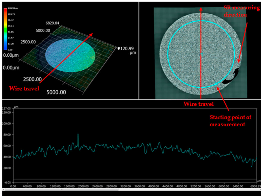
Figure 5. Surface analysis of machined sample at outermost periphery.
