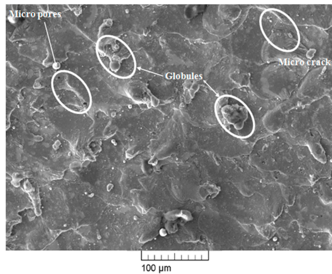
Figure 9. SEM micrograph at optimized parameter settings.
