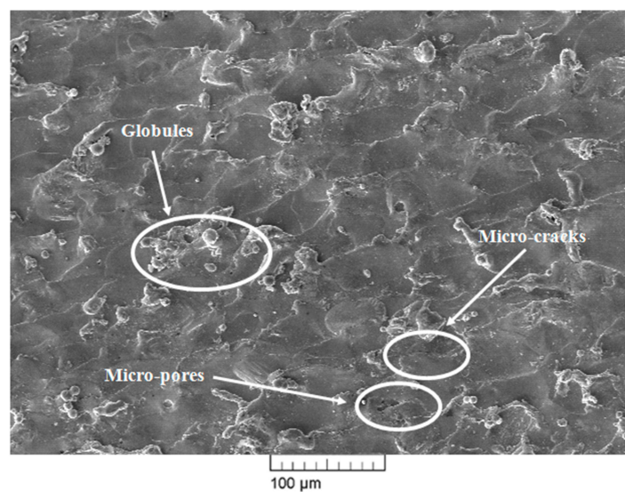
Figure 7. SEM micrograph at low discharge energy level.
