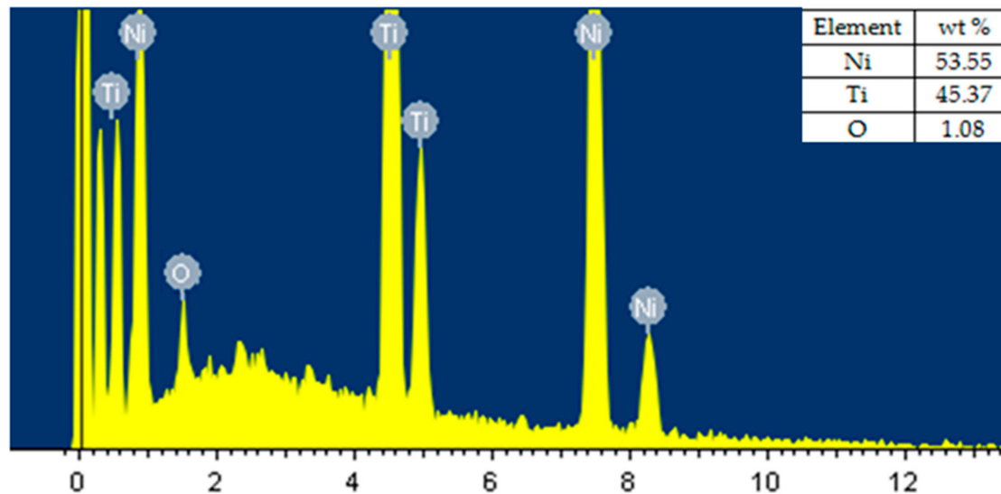
Figure 10. EDX analysis at optimized process parameters.
