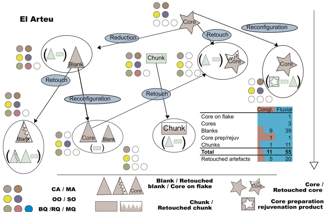
FIGURE 9 A schematic and basic reduction sequence at El Arteu, based on Prieto et al. (2020). The types of quartzite represented are highlighted in colors and associated with each process. Icons in green are byproducts. The association between types of cortex and basic technological categories is shown in the table. BQ, bulging recrystallized quartzite; CA, clastic quartzarenite; MA, matrix or cemented quartzarenite; MQ, grain boundary migration recrystallised quartzite; OO, syntaxially overgrown orthoquartzite; RQ, subgrain rotation recrystallized quartzite; SO, saturated grain orthoquartzite [Color figure can be viewed at wileyonlinelibrary.com ]
