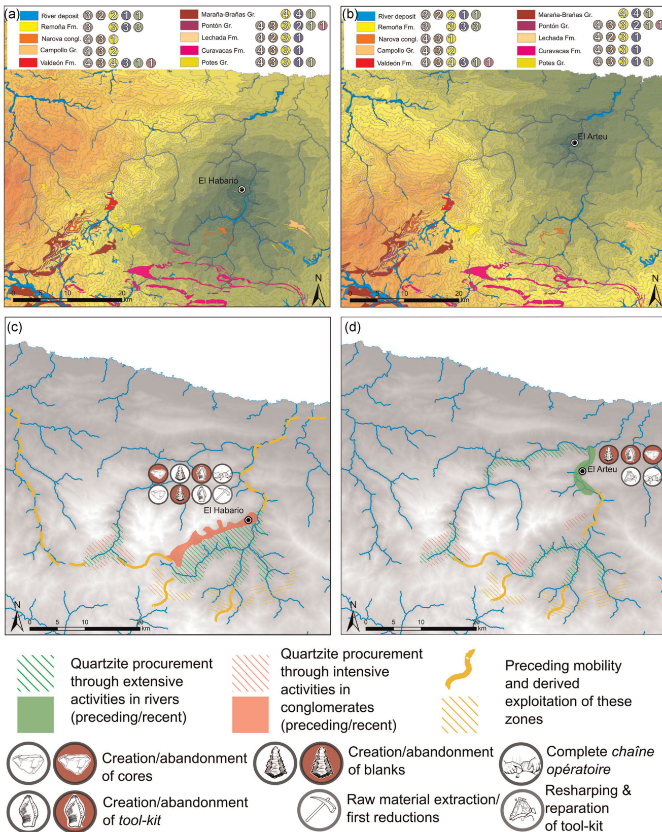
FIGURE 11 Cost maps from (a) El Habario and (b) El Arteu to geological strata where quartzite types are represented. The colored circles in the key represent the lithologies in each geological formation (following the color code of previous figures). Numbers are used to quantify the proportion of each type: 4 when the frequency is >30%; 3 for 10%–30%; 2 for 2%–10%; and 1 when frequencies <2% are found. Quartzite procurement area map of (c) El Habario and (d) El Arteu. Most representative management of raw material according to Prieto et al. (2020) is highlighted [Color figure can be viewed at wileyonlinelibrary.com ]
