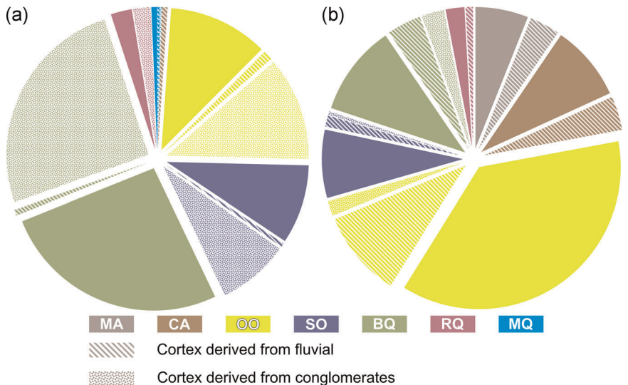
FIGURE 7 A pie chart representing the quartzite distribution grouped by petrogenetic types and cortex types at the assemblage of (a) El Habario and (b) El Arteu. BQ, bulging recrystallized quartzite; CA, clastic quartzarenite; MA, matrix or cemented quartzarenite; MQ, grain boundary migration recrystallised quartzite; OO, syntaxially overgrown orthoquartzite; RQ, subgrain rotation recrystallized quartzite; SO, saturated grain orthoquartzite [Color figure can be viewed at wileyonlinelibrary.com ]
