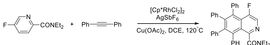
Scheme 4.20 Rh-catalysed synthesis of fluoroisoquinoline.
