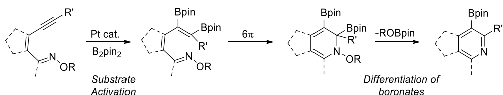
Scheme 4.38 Diboration/ 6\pi -electrocyclisation strategy.
