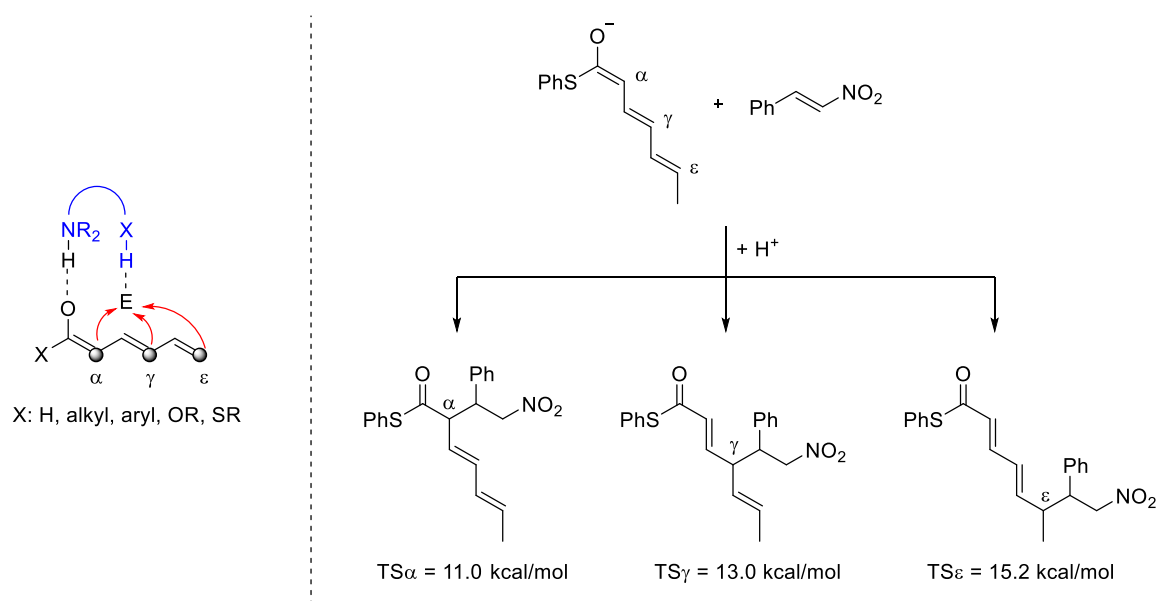
Figure 2.32 Generic bifunctional activation model involving trienolates (on the left); activation energies of the transition states of the reaction of nitrostyrene with thioester enolate XI through C_\alpha , C_\gamma and C_\epsilon , respectively (on the right).
