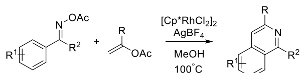
Scheme 4.26 A Rh-catalysed sequential oxidative C–H activation/annulation.
