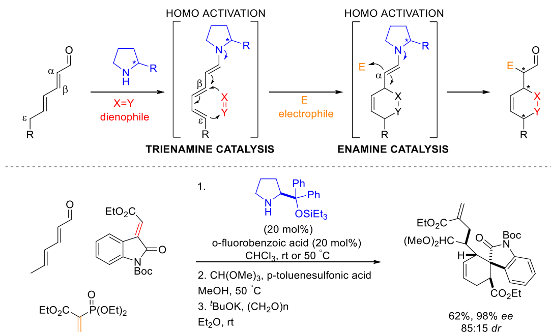
Scheme 2.34 Sequential and cycle specific trienamine and enamine tandem reaction by Chen and Jørgensen.
