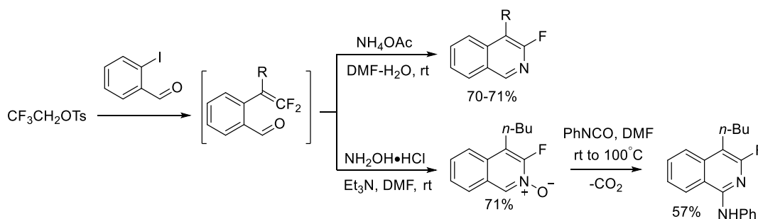
Scheme 4.19 Synthesis of 3-fluoroisoquinolines via intramolecular \text{S}_{\text{N}}\text{V} reaction of difluorostyrenes bearing a formyl group.
