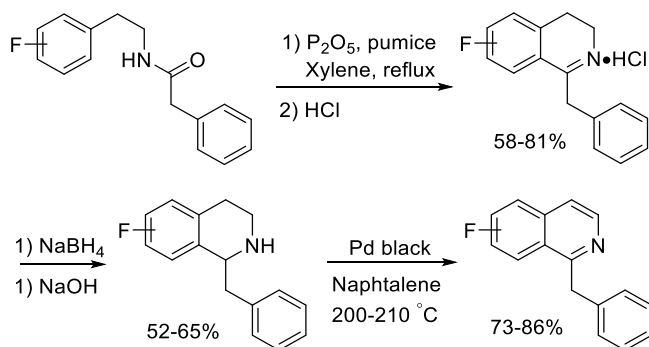
Scheme 4.7 Bischler-Napieralski reaction for the synthesis of fluoroisoquinolines.
