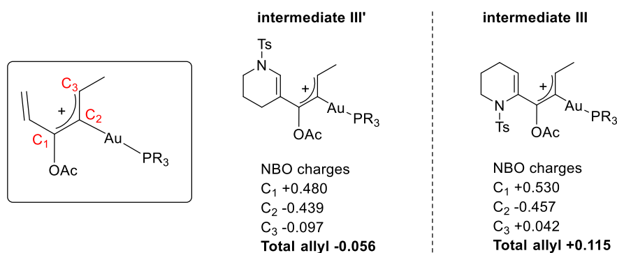
Figure 3.8 NBO charges of the two pentadienyl intermediates III' and III .
