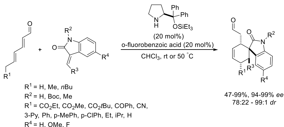
Scheme 2.33 First trienamine mediated catalytic Diels Alder by Chen and Jørgensen. 94
