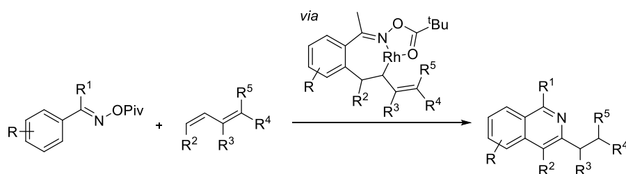
Scheme 4.25 Rh(III)-catalysed isoquinoline synthesis from 1,3-dienes.
