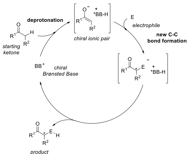
Scheme 2.11 General catalytic cycle for Brønsted Base-catalysed reactions.
