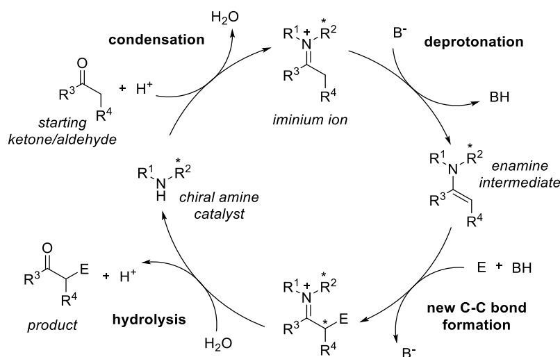
Scheme 2.7 Catalytic cycle for enamine mediated processes. 22
