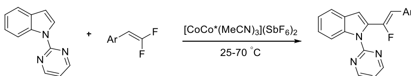
Scheme 4.31 Cobalt(III)-catalysed regio- and stereoselective \alpha -fluoroalkenylation of arenes with gem -difluorostyrene.
