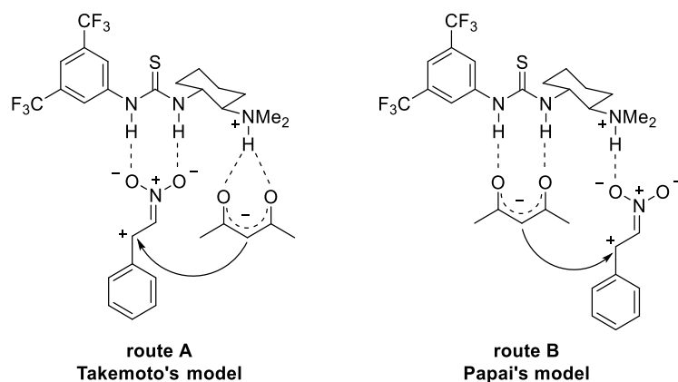
Scheme 2.15 Two alternative reaction routes for the Michael addition catalysed by bifunctional catalyst. 51
