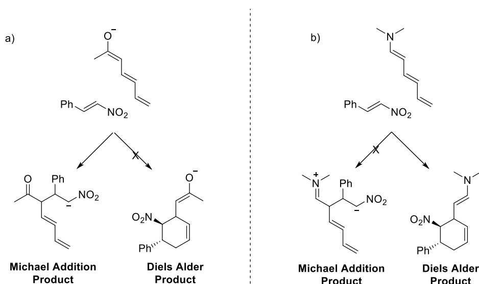
Figure 2.31 Potential reactivity of a) trienolates and b) trienamines with nitroolefins.
