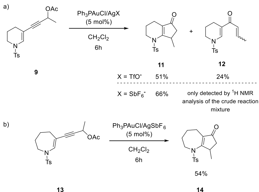
Scheme 3.33 Gold(I) catalysed [3,3]-rearrangement/Nazarov reactions.
