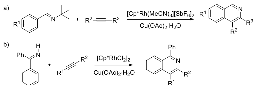
Scheme 4.2 Rh-catalysed synthesis of isoquinolines by a) Fagnou and b) Miura groups.
