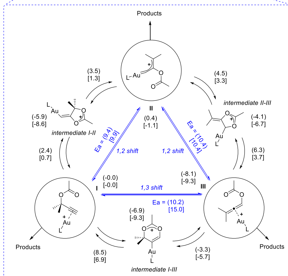
Scheme 3.14 On the top, key intermediates along the catalytic cycle of propargylic ester in equilibrium; on the bottom, a look into the equilibrium cycle thermodynamics, computed by Cavallo and co-workers. Energies in kcal/mol (in round/square brackets for L=Ime and PMe_3 , respectively) are calculated relative to I. Numbers close to the arrows represent the energies of the transition states associated with that reaction step.
