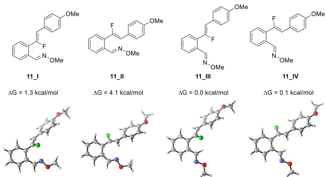
Figure 4.3 Conformers of azatriene 11 and relative energies. Energies ( \Delta G ) referred to the lowest energy conformation, \Delta G=0.0 kcal/mol.
