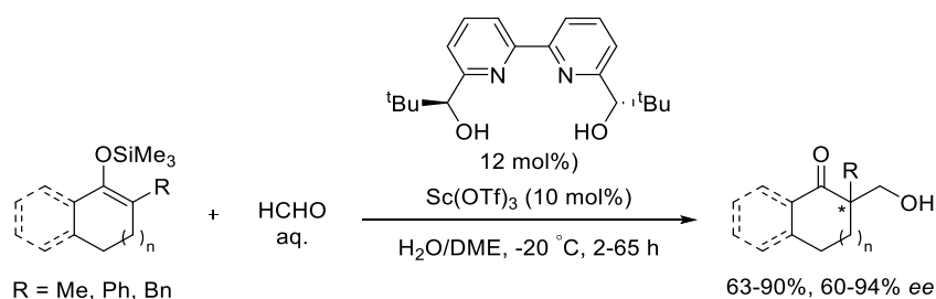
Scheme 2.18 Hydroxymethylation of silyl enolates using a chiral scandium complex by Kobayashi et al.
