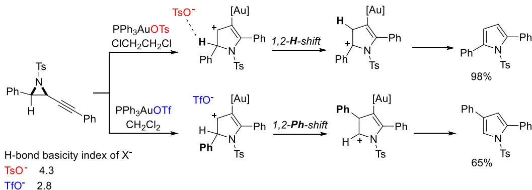
Scheme 3.8 Effects of the counterion on regioselectivity.
