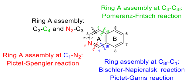
Figure 4.1 Generic representation of synthetic strategies to build the isoquinoline core.
