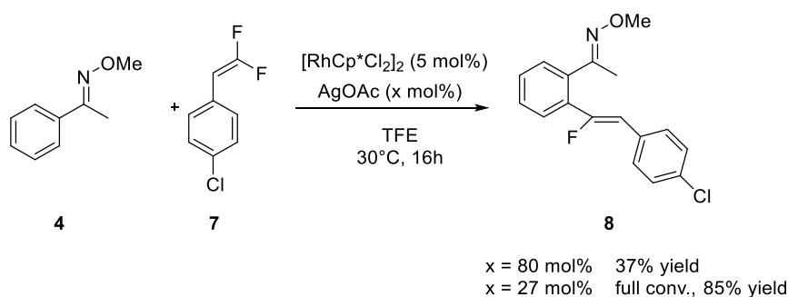
Scheme 4.44 Rh-catalysed reaction of oxime 4 with difluoroalkene 7 .
