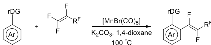
Scheme 4.35 C–F/C–H functionalisation through Mn(I) Catalysis: (per)fluoro-allylations and alkenylations.
