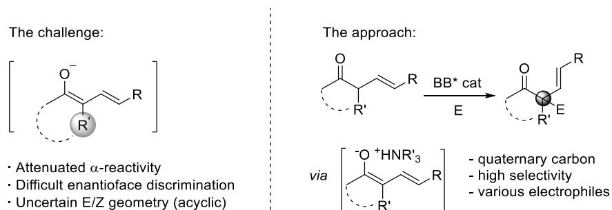
Figure 2.23 \alpha -substituted dienolates issues and the approach based on BB catalysis.
