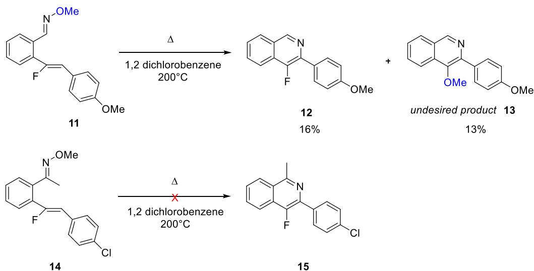
Scheme 4.45 Electrocyclisation reactions of azatrienes obtained through Rh(III)-catalysed C-H activation.
