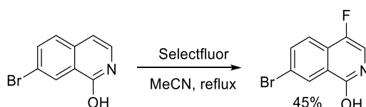
Scheme 4.11 Electrophilic fluorination with Selectfluor.
