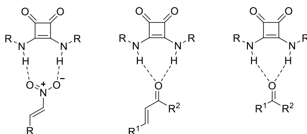
Figure 2.10 Activation of different substrates by squaramides.
