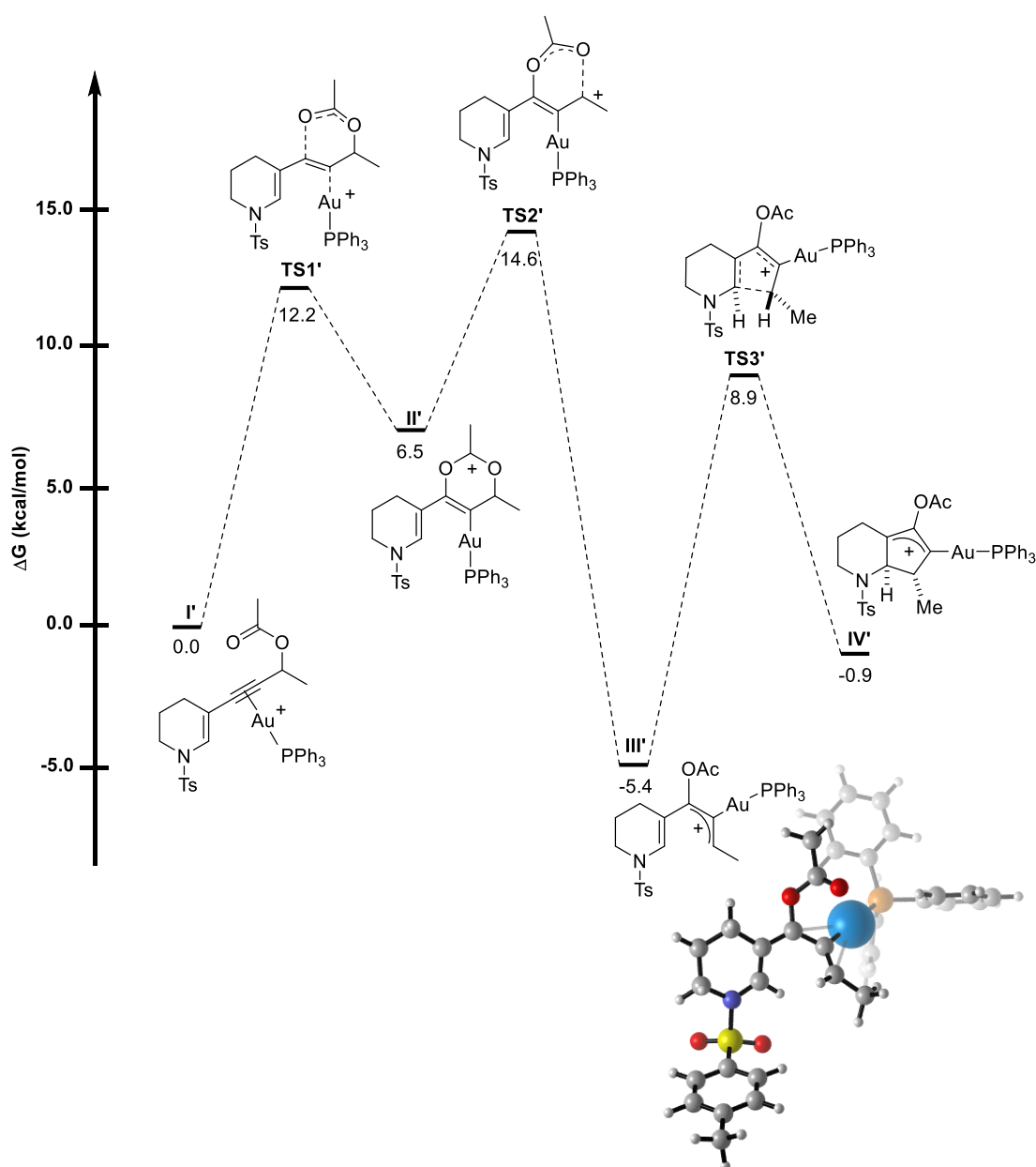
Scheme 3.28 DFT computed energy surface for the tandem Au(I)-catalysed [3,3]-rearrangement/Nazarov reaction of 3-substituted piperidine derivatives.
