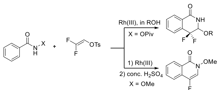
Scheme 4.30 Rh-catalysed coupling of benzamides with 2,2-difluorovinyl tosylate.
