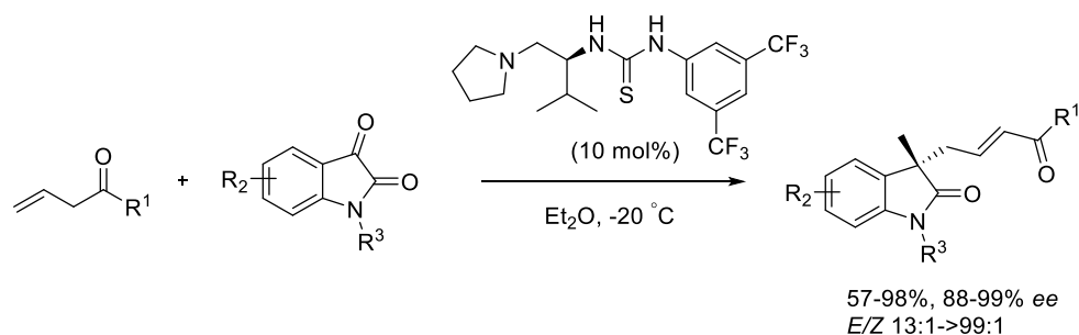
Scheme 2.26 Direct asymmetric vinylogous aldol reaction of allyl ketones with isatins catalysed by a readily prepared L-valine-derived bifunctional tertiary amine/thiourea catalyst by Jiang et al.
