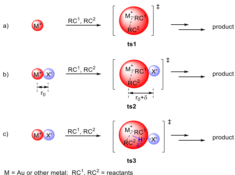
Figure 3.6 Simplified representation of cationic metal-catalysed reactions.
