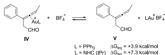
Scheme 8. Calculated Energies for the Dissociation of Complex IV
