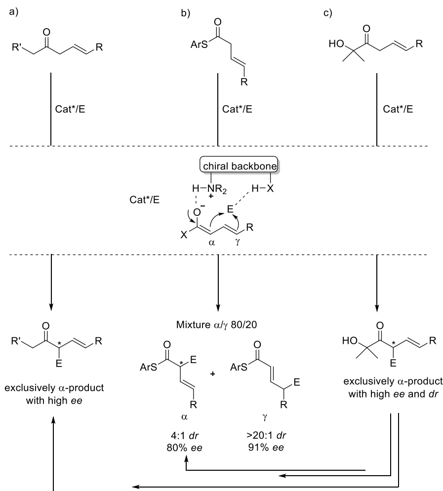
Scheme 2.37 BB/H-bond donor catalysed addition of \beta,\gamma -unsaturated substrates with nitroolefins by Palomo et al.
