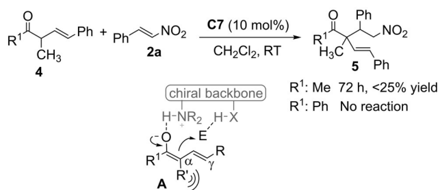
Scheme 1. Impact of \alpha -substitution on the reactivity of transiently formed acyclic ketone dienolates.
