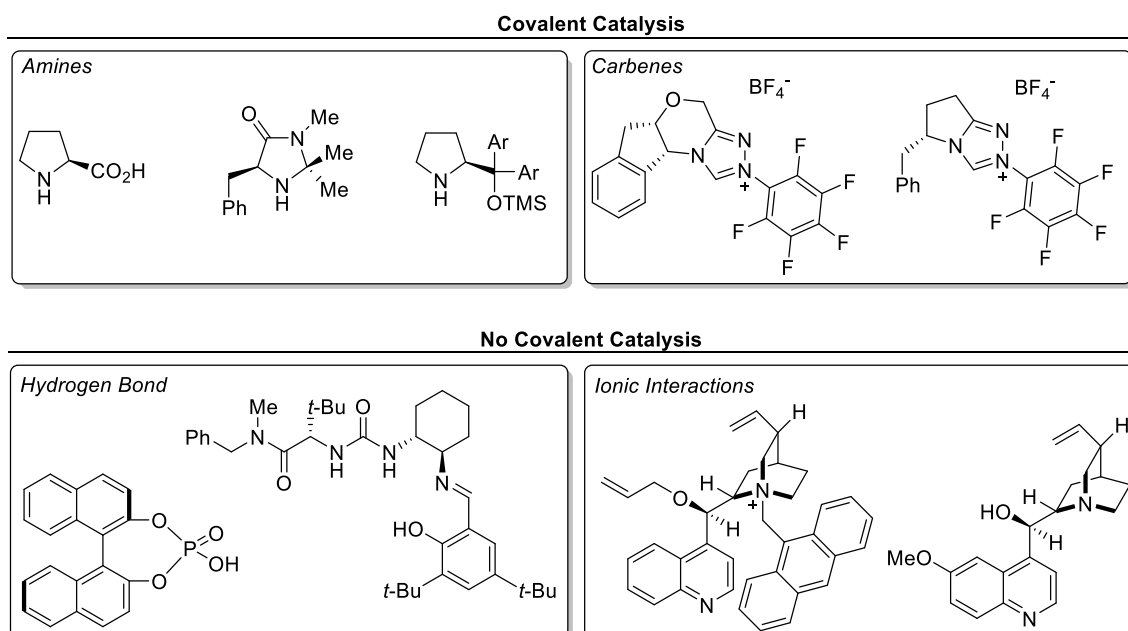
Figure 2.1 Activation modes in organocatalysis.
