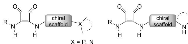
Figure 2.11 General structures of squaramide asymmetric organocatalysts.
