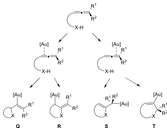
Scheme 3.44 Regioselectivity of the nucleophilic attack.
