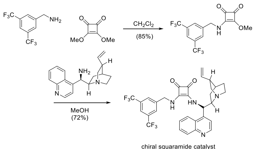
Scheme 2.13 Synthesis of a chiral squaramide catalyst by Rawal et al. 35
