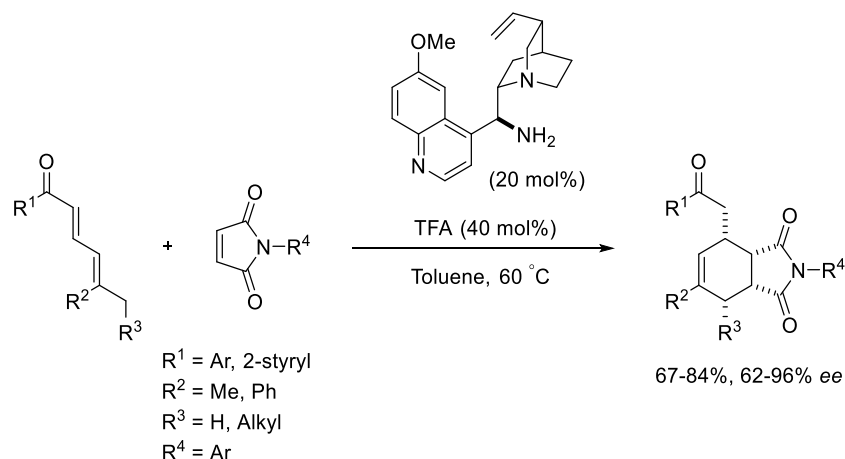
Scheme 2.35 Trienamine mediated catalytic Diels Alder of 2,4-dienones by Chen et al.
