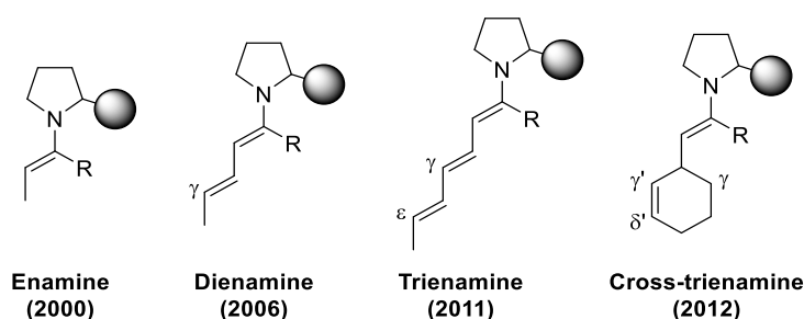
Figure 2.28 Advances in amine catalysis through HOMO-raising activation strategy.
