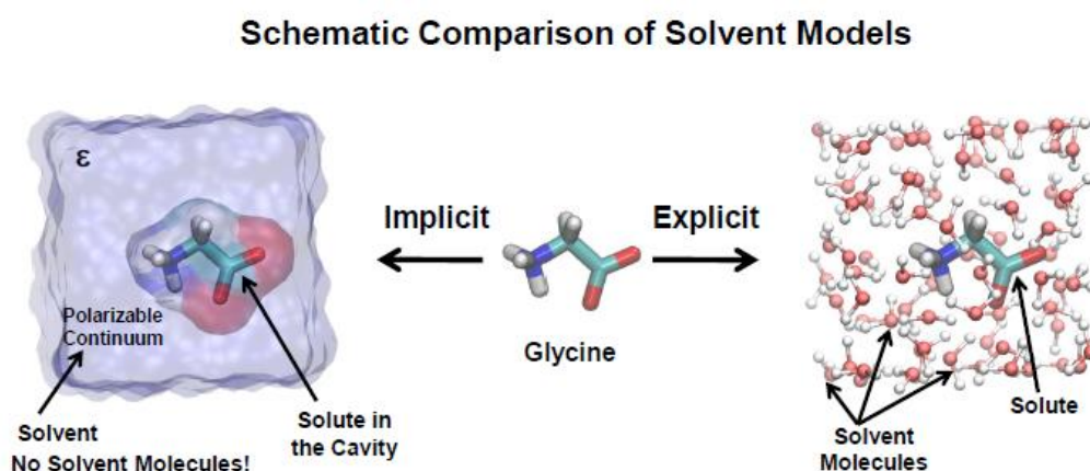
Figure 1.3 Schematic comparison of implicit and explicit solvation model. 30
