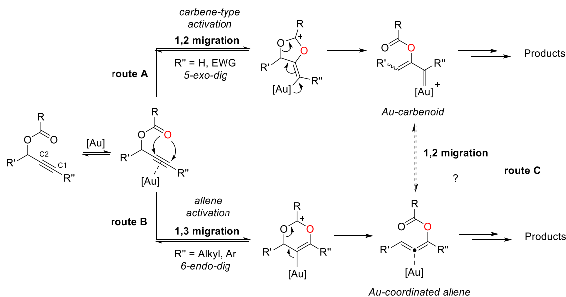
Scheme 3.13 General reactivity patterns for propargyl esters.
