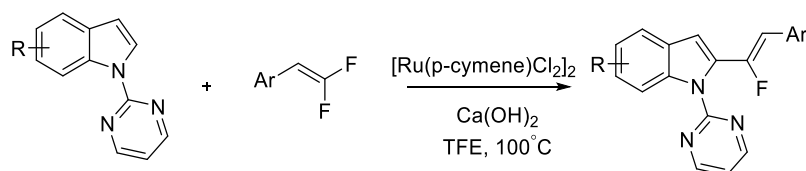
Scheme 4.36 Ru(II)-catalysed \alpha -fluoroalkenylation of arenes.
