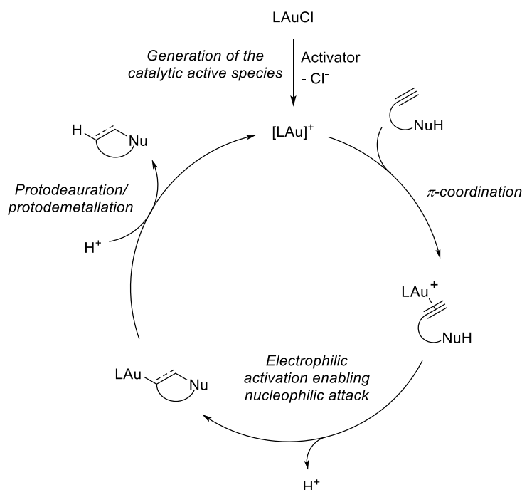
Scheme 3.1 Proposed gold(I) catalytic cycle.
