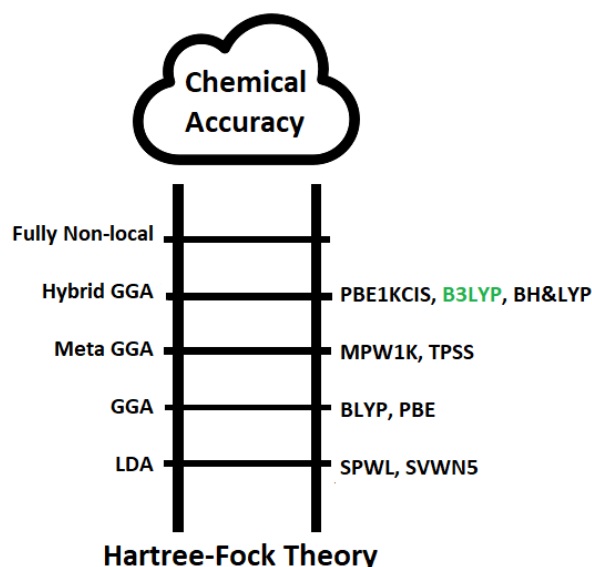
Figure 1.1 Jacob's Ladder representation.
