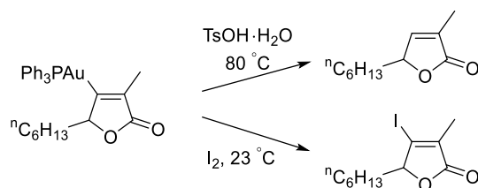
Scheme 3.4 Electrophilic attack to an alkenyl gold(I) complex.
