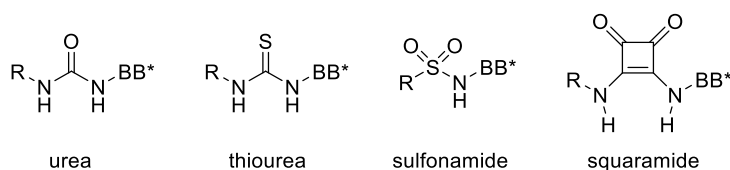
Figure 2.7 Examples of H-bond donor groups.
