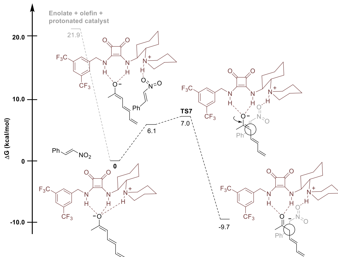
Scheme 2.46 Energetic profile of C2 -catalysed Michael addition of trienolate IX and nitrostyrene. The energies are Gibbs energies in kcal/mol.
