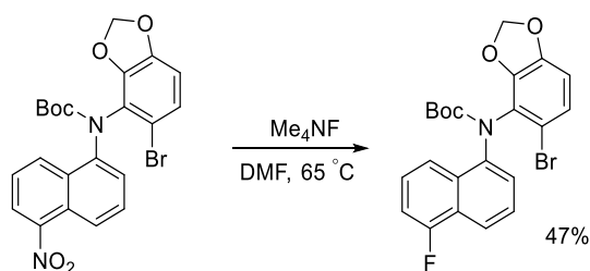
Scheme 4.9 Synthesis of 8-fluoroisoquinoline via fluorodenitration with Me 4 NF.
