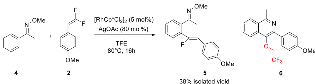
Scheme 4.43 Rh-catalysed reaction of oxime 4 with difluoroalkene 2 .
