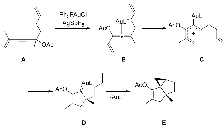
Scheme 3.5 Nazarov-type cyclisation of substrate A.
