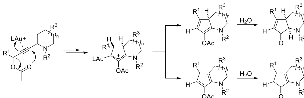
Scheme 3.21 Sequence of gold(I)-catalysed [3,3]-rearrangement/Nazarov reaction for the synthesis of cyclopenta-fused N -heterocycles.
