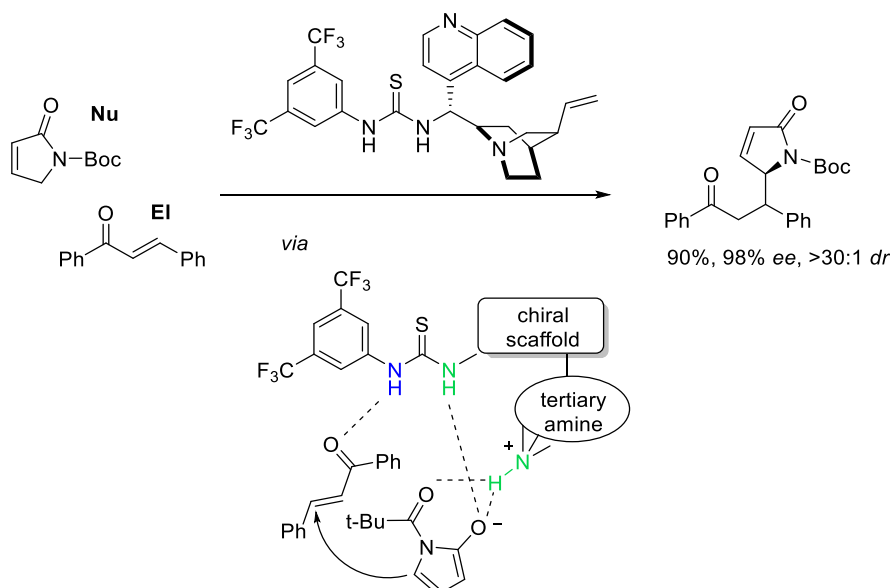
Scheme 2.17 Vinylogous Michael addition of \alpha,\beta -unsaturated butyrolactam to chalcone catalysed by bifunctional cinchona alkaloid thiourea organocatalyst that follows the mechanism by Wang.
