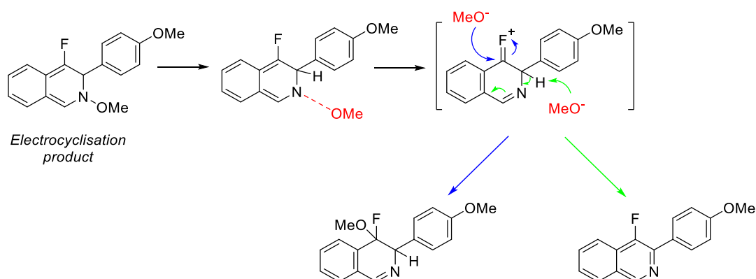
Scheme 4.51 Mechanism for the spontaneous displacement of the methoxy group and following possible routes.
