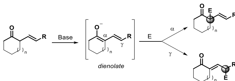
Figure 2.19 Enolisation of \alpha -alkenyl cycloalkanones and the issue of \alpha vs \gamma reaction selectivity.
