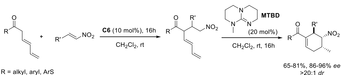
Scheme 2.41 Suitability of the Brønsted base-catalysed one pot strategy to various unsaturated carbonyl compounds.
