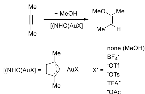
Scheme 3.9 Study of counterion effect on NHC gold(I)-catalysed alkoxylation of alkynes by Ciancaleoni et al.
