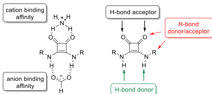
Figure 2.8 Duality in ditopic- and hydrogen-bonding of squaramides. 36
