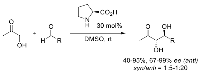
Scheme 2.8 Proline-catalysed aldol reaction by Notz and List. 23
