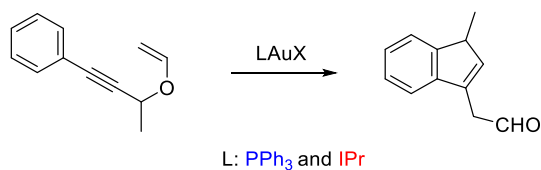
Scheme 3.48 Model reaction studied computationally.
