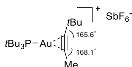
Figure 3.2 Structure of the \eta^2 -alkyne Au(I) complex.
