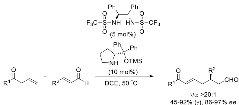
Scheme 2.25 Direct vinylogous Michael addition of unmodified linear \beta,\gamma -unsaturated ketones to \alpha,\beta -unsaturated aldehydes by Xu et al.
