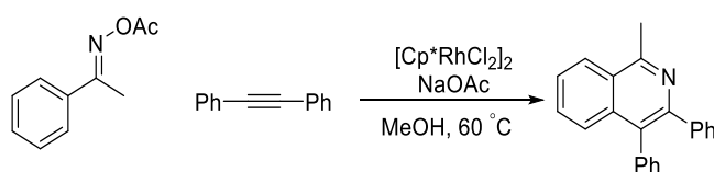
Scheme 4.23 Synthesis of isoquinolines from aryl ketone O-acyloxime derivatives and internal alkynes using [\text{Cp}^*\text{RhCl}_2]_2\text{-NaOAc} .
