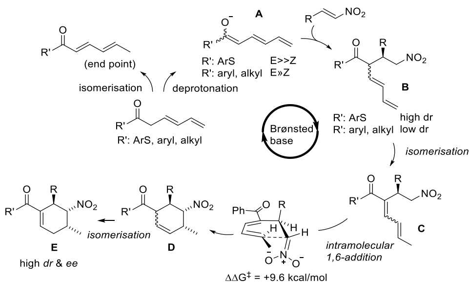
Scheme 2.47 Plausible pathway of the one-pot reactions sequence.
