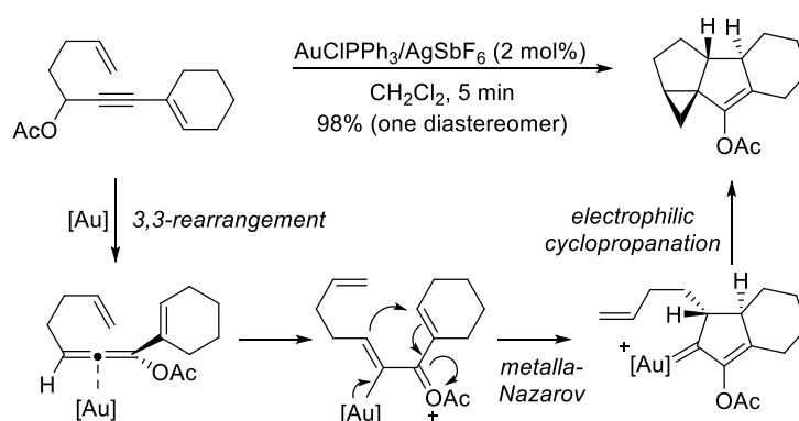
Scheme 3.18 Au-catalysed cyclisation/cyclopropanation by Fensterbank et al.
