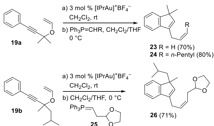
Scheme 3.47 Wittig reaction for chain elongation starting from the starting materials.
