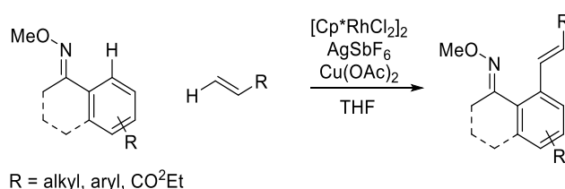
Scheme 4.28 Example of C-H activation in oximes under rhodium catalysis.
