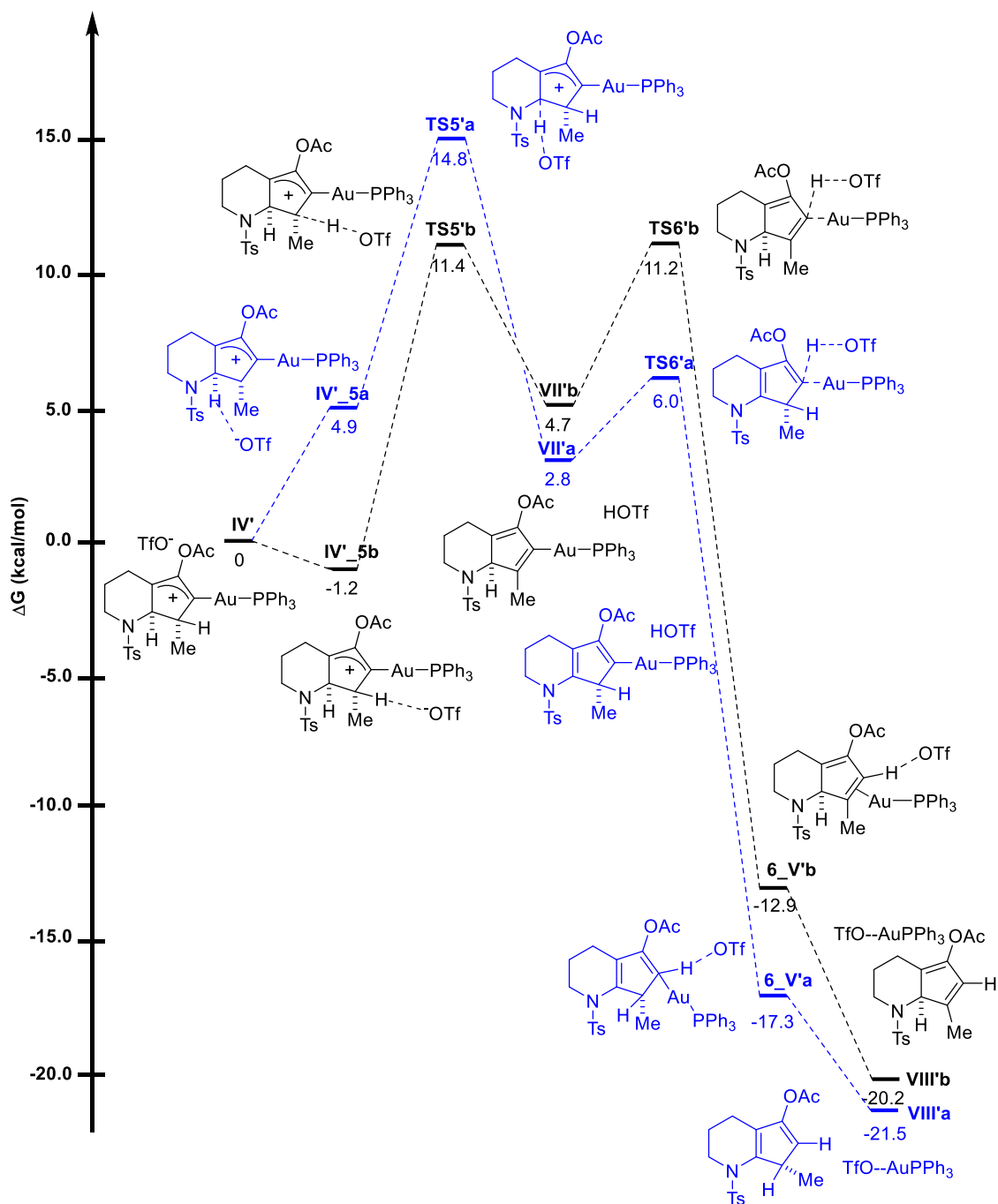
Scheme 3.31 Triflate mediated proton H_a and H_b abstraction pathways.
