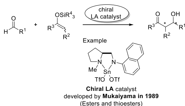
Scheme 2.6 Mukaiyama aldol reaction.
