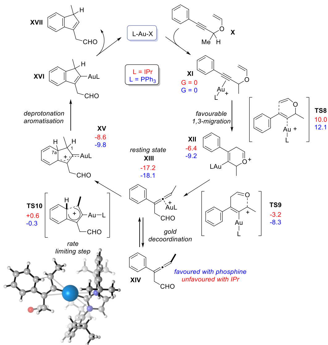
Scheme 3.49 Schematic representation of the thermodynamics associated with the tandem process. Energies in kcal/mol are calculated relative to XI (in blue for Ph 3 P ligand, in red for IPr ligand).
