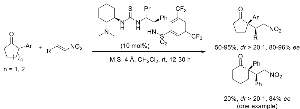
Scheme 2.20 Michael reaction of \alpha -aryl cycloalkanones catalysed by a Brønsted base/H-bond catalyst by Wang et al.
