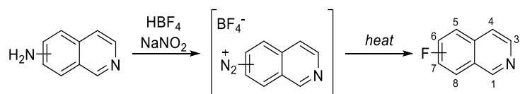
Scheme 4.4 The Baltz-Schiemann reaction.
