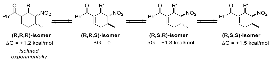
Figure 2.36 Study of the relative stability of cycloadduct E and its three diastereoisomers.
