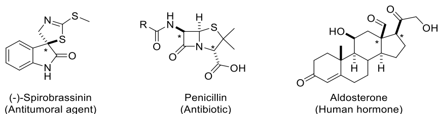
Figure 2.2 Some examples of biologically active compounds and natural products containing carbonyl groups with an adjacent stereocentre.
