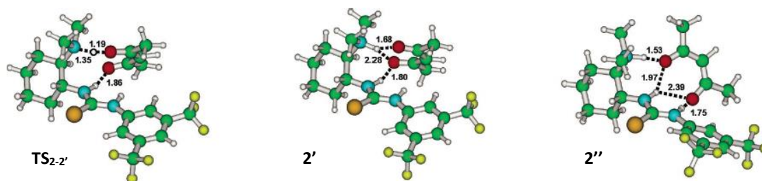
Figure 2.13 Optimised structures of stationary points located for the protonation process between catalyst and nucleophile
