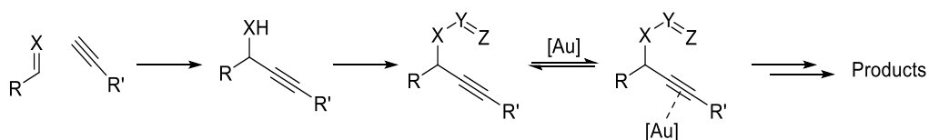
Scheme 3.11 Propargylic alcohol derivatives under gold catalysis.
