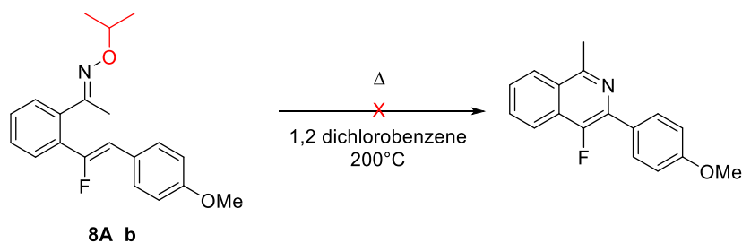
Scheme 4.47 Electrocyclisation of compound 8A_b .
