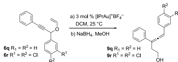
Scheme 5. Gold(I)-Catalyzed Process with Substrates 6q and 6r
