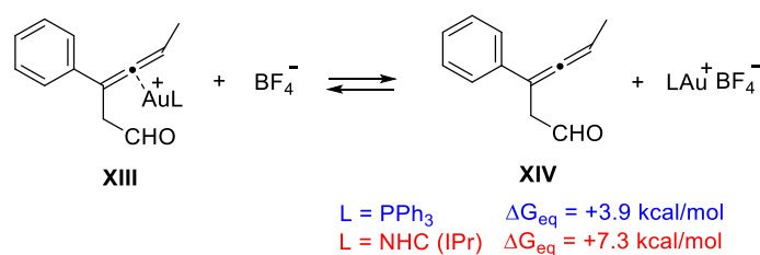
Scheme 3.51 Dissociation equilibrium of complex XIII and XIV .
