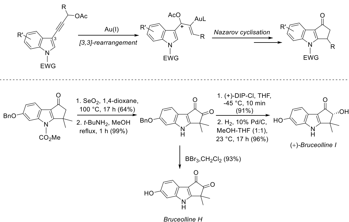
Scheme 3.22 Tandem Au(I)-catalysed [3,3]-rearrangement/Nazarov reaction and application for the synthesis of Bruceolline H and I by Occhiato et al.
