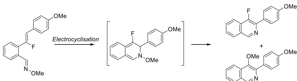
Scheme 4.49 Products formed after subjecting azatrienes to electrocycloisisation conditions.
