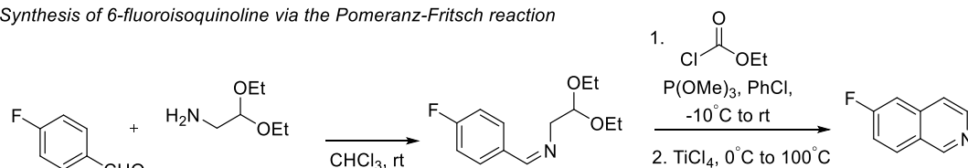
Scheme 4.14 Application of the Pomeranz-Fritsch reaction for the synthesis of 6-fluoroisoquinoline.
