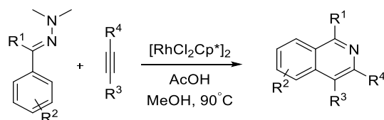
Scheme 4.24 Rh(III)-catalysed synthesis of highly substituted isoquinolines starting from hydrazones.
