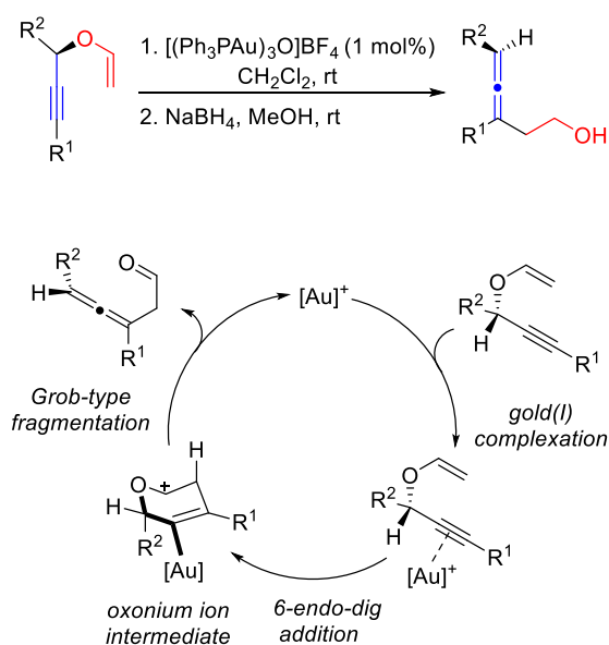
Scheme 3.38 [3,3]-sigmatropic rearrangement of propargyl vinyl ethers by Toste et al and proposed mechanism.
