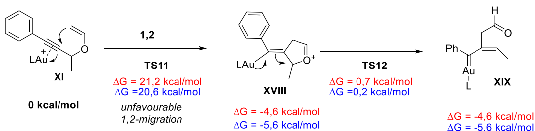
Scheme 3.50 Calculation of the energies related to the 1,2-rearrangement of substrate XI .
