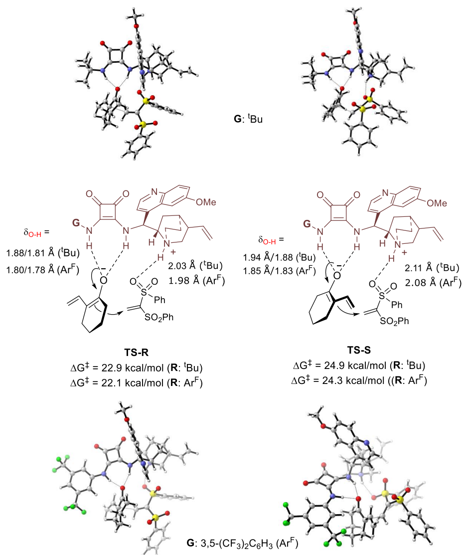
Scheme 2.32 TS structures and selected parameters for the model reaction between \alpha -branched dienolate III and bis(phenylsulfonyl)ethane.
