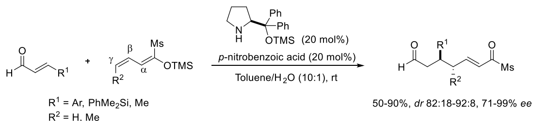
Scheme 2.22 Catalytic enantioselective Michael reaction with linear preformed dienolates by Schneider et al.
