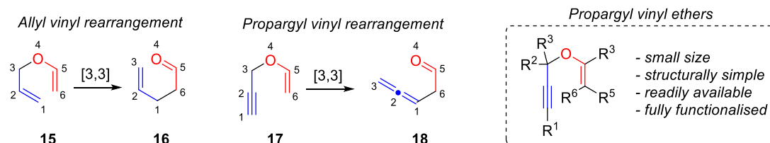
Scheme 3.37 Allyl vinyl rearrangement vs propargyl vinyl rearrangement.
