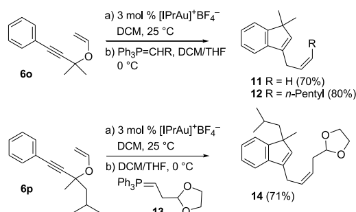
Scheme 9. Sequential Au(I)-Catalyzed Tandem Process/Wittig Olefination of Substrates 6o–p
