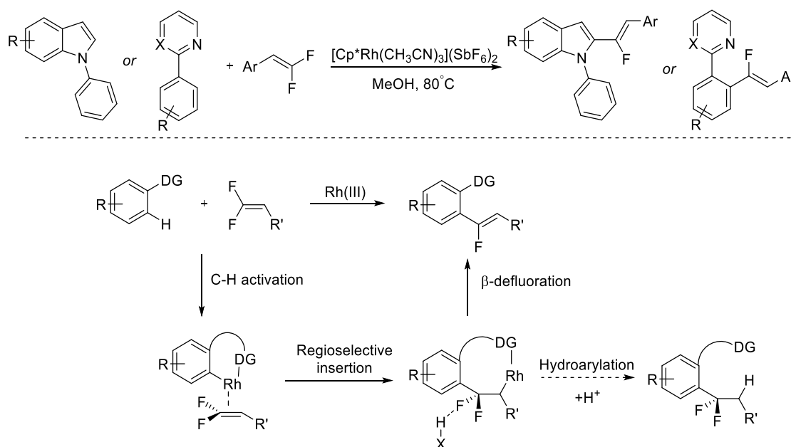
Scheme 4.29 Rh(III)-catalysed \alpha -fluoroalkenylation of (hetero)arenes.
