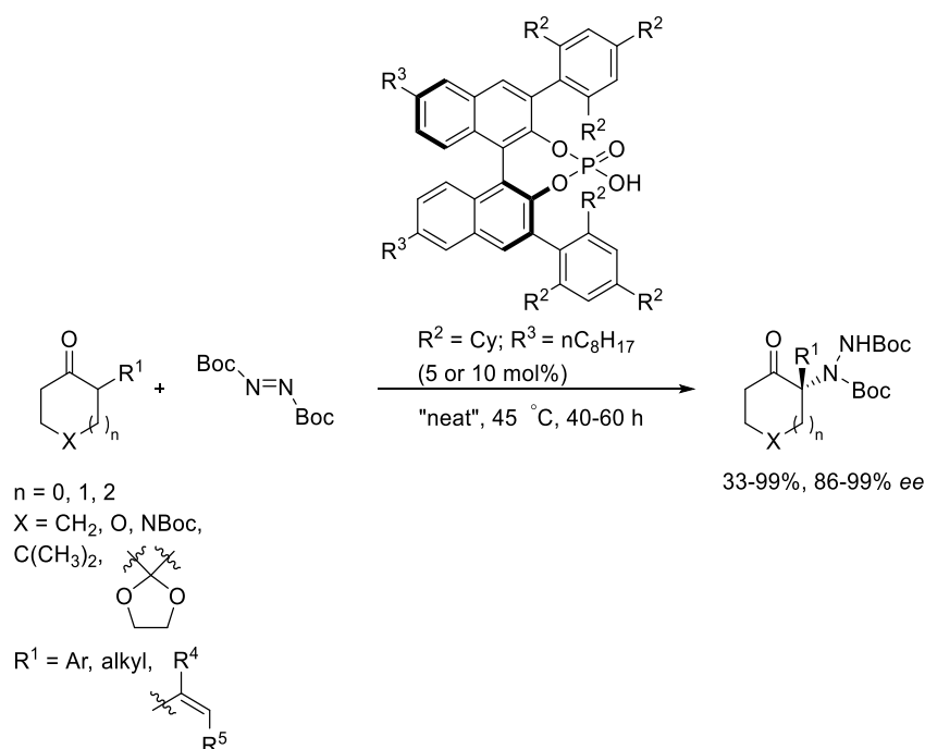
Scheme 2.29 Direct asymmetric amination catalysed by a chiral phosphoric acid to generate N -containing tetrasubstituted carbon stereocentres by Toste et al.
