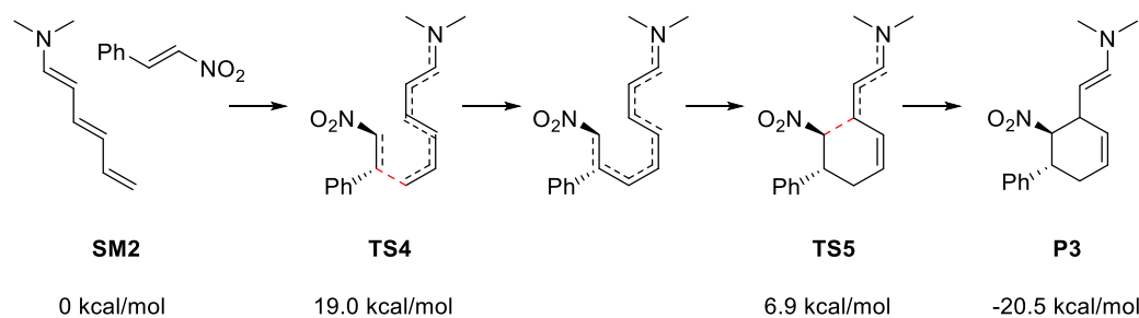
Scheme 2.44 Mechanism of Diels Alder reaction of trienamine and nitroolefin. The energies are Gibbs Energies in kcal/mol.
