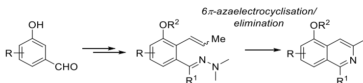
Scheme 4.40 Synthesis of isoquinolines from hydrazones.
