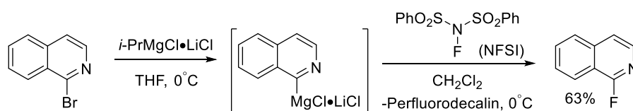
Scheme 4.12 Electrophilic fluorination of 1-isoquinolylmagnesium reagent.
