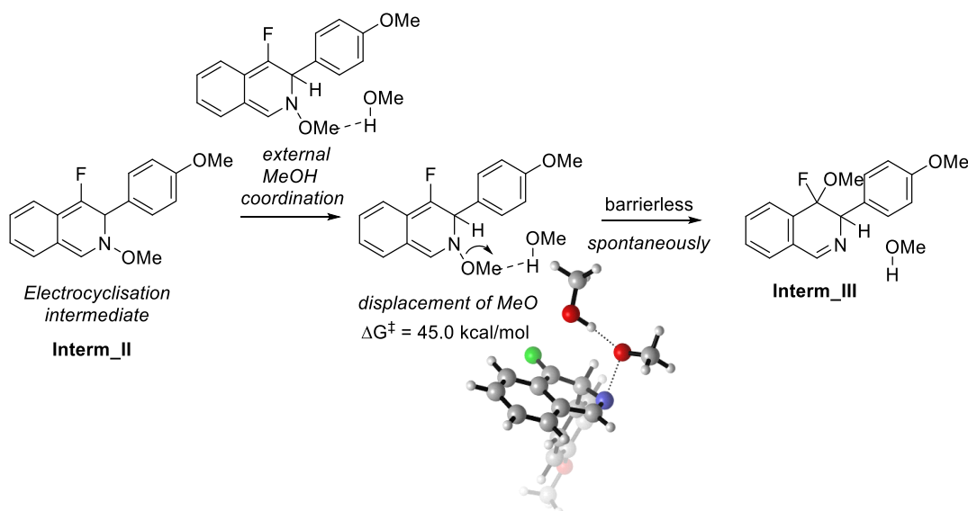
Scheme 4.52 Mechanism mediated by an external molecule of MeOH present in the reaction media. All the energies are Gibbs energies in kcal/mol using as reference interm_I (Scheme 4.50) with \Delta G = 0 kcal/mol.
