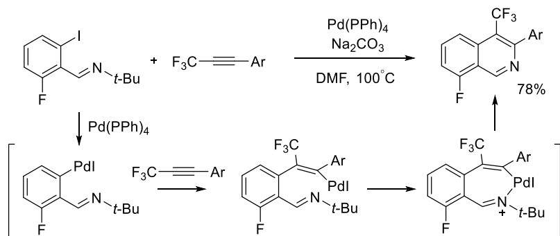
Scheme 4.16 Pd-catalysed domino insertion/cyclisation sequence for 8-fluoroisoquinoline synthesis.
