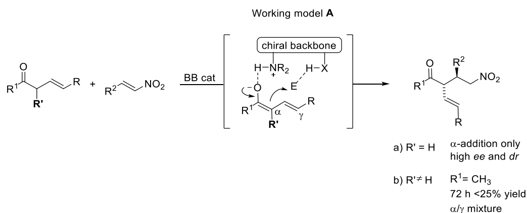
Figure 2.22 Impact of \alpha -substitution on the reactivity of transiently formed acyclic ketone dienolates.
