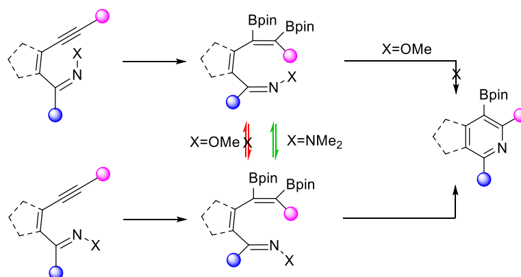
Scheme 4.39 Synthesis of borylated (heteroaromatic) pyridines and ring-fused analogues from hydrazones.
