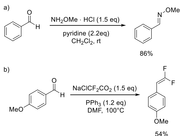
Scheme 4.42 Synthesis of the starting materials for the optimisation screening.
