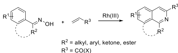
Scheme 4.27 Rh(III)-catalysed C–H activation/cyclisation of oximes and alkenes.
