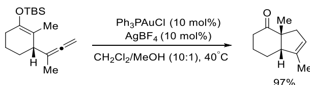
Scheme 3.43 5- endo-trig cyclisation to hexahydroindenone derivative.
