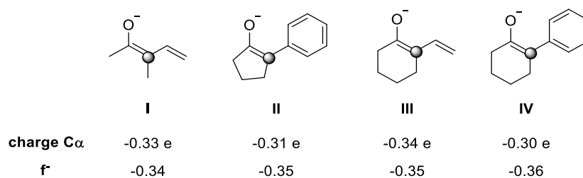
Figure 2.24 Charge distribution and Fukui nucleophilicity index ( f^* ) at the \alpha -carbon on the model linear I and cyclic enolates II-IV .
