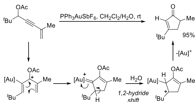
Scheme 3.17 Au-catalysed tandem [3,3]-rearrangement-Nazarov reaction by Zhang et al.
