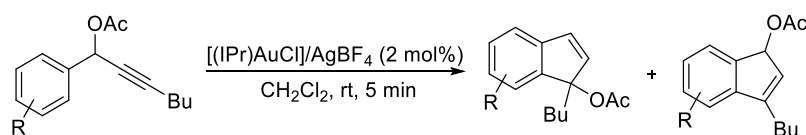
Scheme 3.34 Synthesis of indenes by Nolan group.
