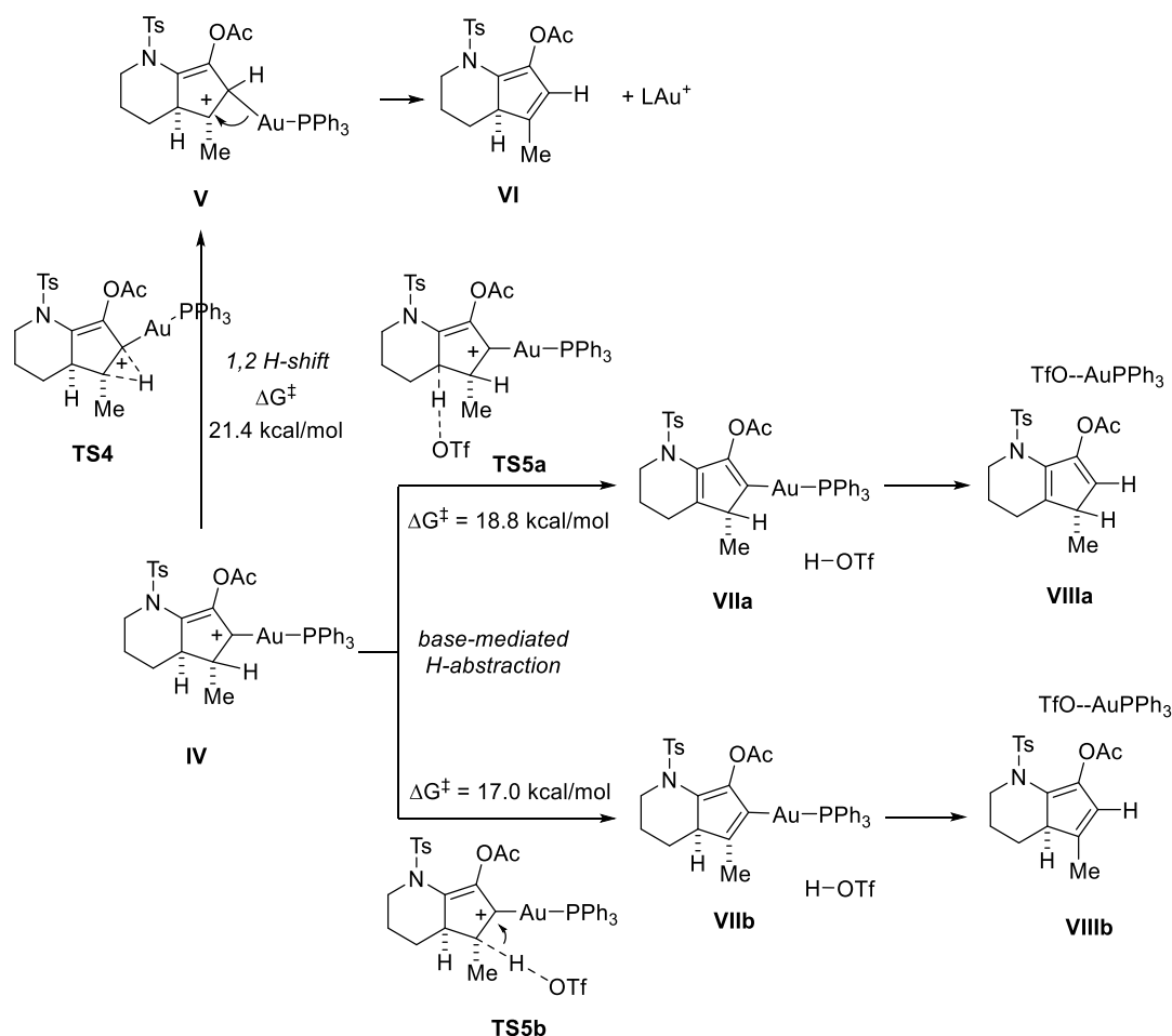
Scheme 3.26 Diene formation pathways.
