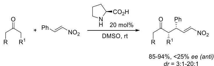
Scheme 2.9 Proline-catalysed Michael reaction by List et al. 24
