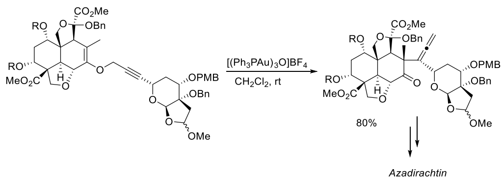
Scheme 3.42 Gold-catalysed transformation towards the total synthesis of azadirachtin.
