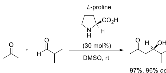
Scheme 2.3 Proline-catalysed intermolecular aldol reaction by List et al. 10,11
