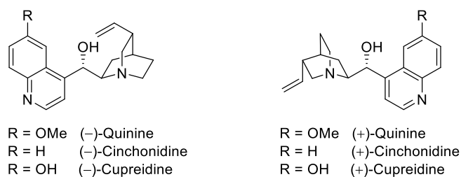
Figure 2.6 Cinchona alkaloids derivatives.
