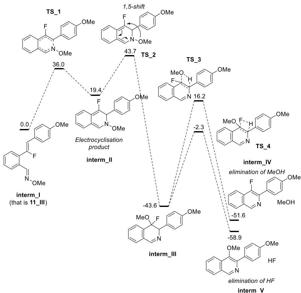
Scheme 4.50 Energetic pathways that lead to 3-fluoroisoquinoline and 3-methoxyisoquinoline. The energy of the fluorinated azatriene ( interm_I ) is taken as reference with \Delta G = 0 kcal/mol. All the energies are Gibbs energies in kcal/mol.
