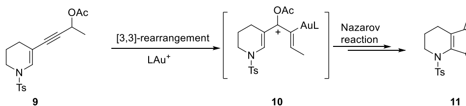
Scheme 3.24 Tandem [3,3]-rearrangement/Nazarov reaction for the 2- and 3-substituted piperidine derivatives.
