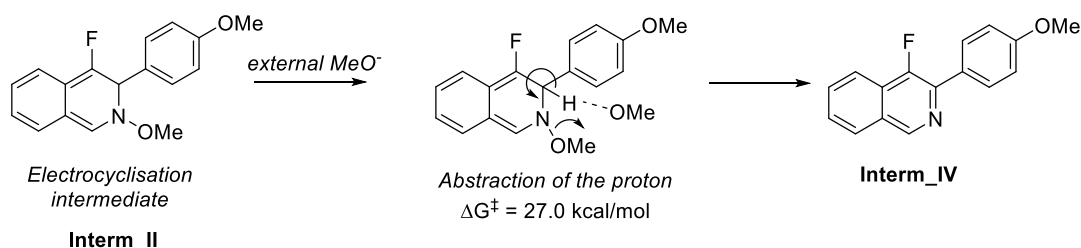
Scheme 4.53 Mechanism mediated by an external methoxy ion present in the reaction media. All the energies are Gibbs energies in kcal/mol using as reference interm_I (Scheme 4.50) with \Delta G = 0 kcal/mol.
