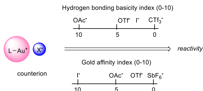
Figure 3.5 Representation of counterion hydrogen bonding basicity and gold affinity influence on the reactivity.
