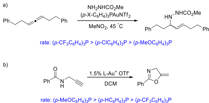
Scheme 3.7 Typical type I and type II gold-catalysed reactions.
