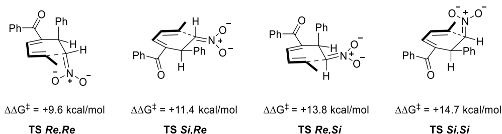
Figure 2.35 Study of the activation energies of the transition states for the carbocyclisation reaction (from deprotonated A )
