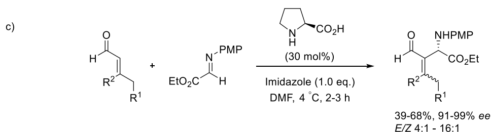
Scheme 2.27 \alpha -addition examples of dienolates or equivalents leading to MBH-type adducts.
