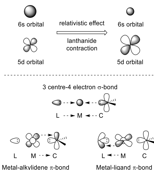
Figure 3.1 Top) effects of relativistic effect and lanthanide contraction on outer-shell orbitals of gold; bottom) Ligand-metal-substrate orbital interactions in gold carbenes [L-Au=CR_2]^+ .
