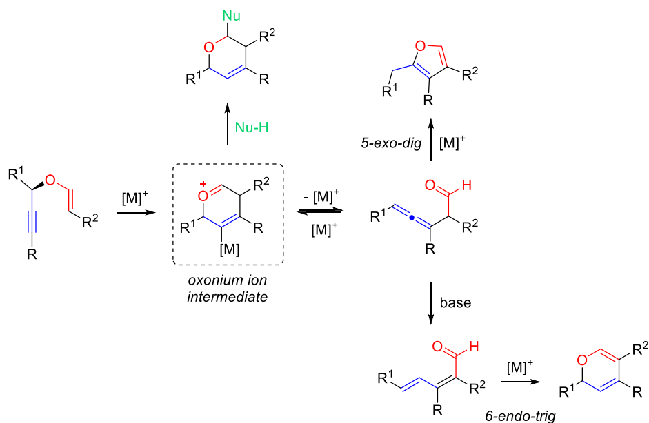
Scheme 3.39 Metal-catalysed rearrangement of propargyl vinyl ethers.
