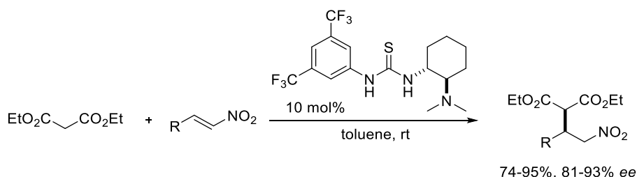
Scheme 2.12 Thiourea-tertiary amine bifunctional catalysed Michael reaction of malonates to nitroalkenes by Takemoto et al. 31
