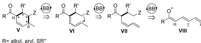
Scheme 2.39 Retrosynthetic pathway of the one-pot catalytic, enantio- and diastereoselective synthesis of stereodefined six-member carbocycles.
