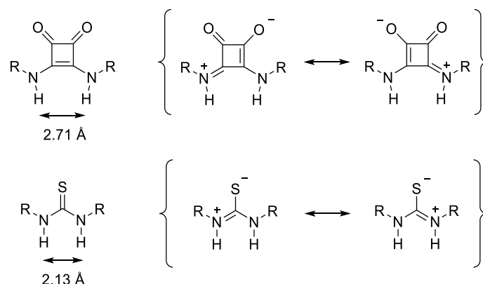
Figure 2.9 Structural differences between squaramides and thioureas.
