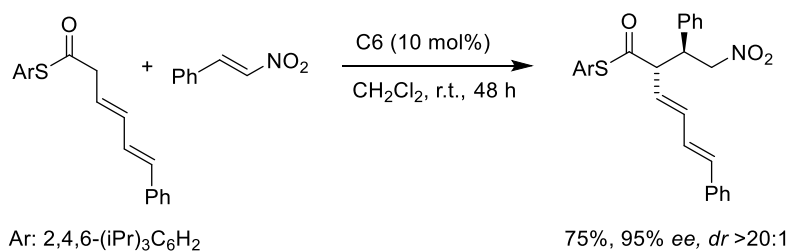
Scheme 2.40 BB/H-bond donor catalysed addition of \beta,\gamma - and \delta,\epsilon -doubly unsaturated aryl thioesters to nitroolefin.
