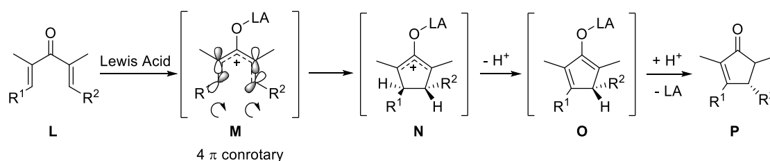
Scheme 3.19 Nazarov reaction mechanism.
