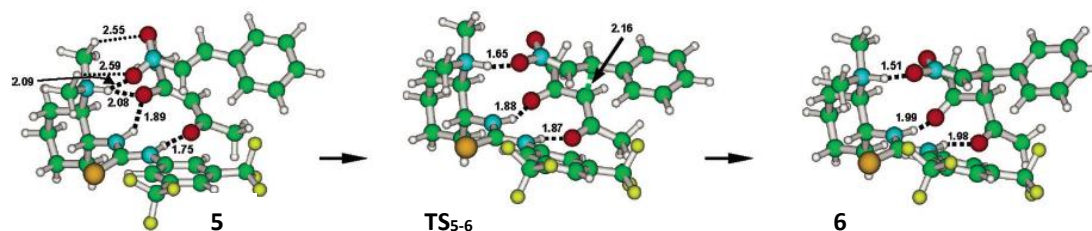
Figure 2.15 Optimised structures and selected geometric parameters of the stationary points located on route B.
