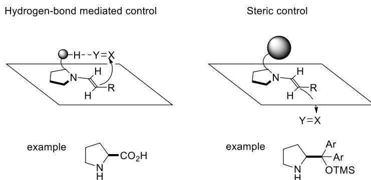
Figure 2.3 Two models to control the stereochemistry of newly formed \alpha -substituted carbonyl compounds
