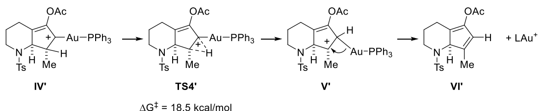
Scheme 3.29 Single-step intramolecular hydride shift pathway.
