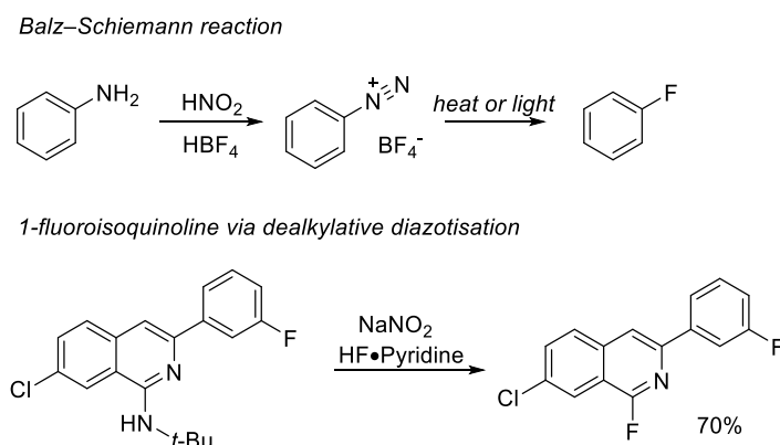
Scheme 4.8 Application of the Balz-Schiemann reaction for the synthesis of fluoroisoquinolines.
