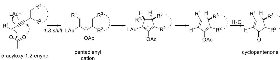
Scheme 3.10 General sequence of gold(I)-catalysed [3,3]-rearrangement/Nazarov reaction for the synthesis of cyclopentenones.
