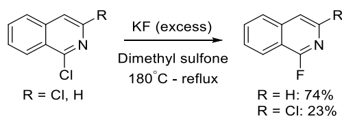
Scheme 4.5 The Halex reaction towards 1-fluoroisoquinolines.
