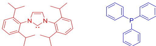
Figure 3.9 Carbene ligand IPr in red and triphenylphosphine ligand \text{PPh}_3 in blue.
