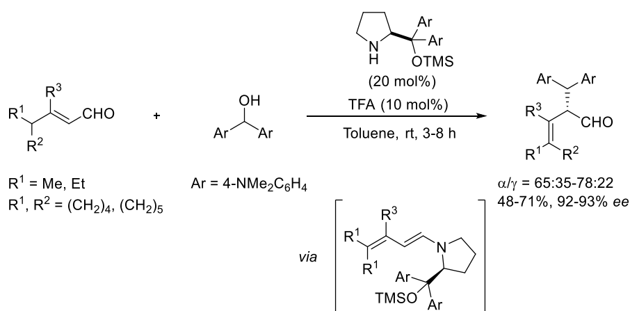
Scheme 2.28 \alpha -addition of \gamma,\gamma -disubstituted enals to stabilised carbocations as electrophiles via activation as dienamine intermediates by Christmann et al.
