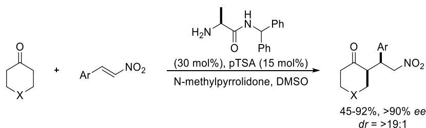
Scheme 2.10 Primary amine-catalysed Michael addition by Córdova et al. 28
