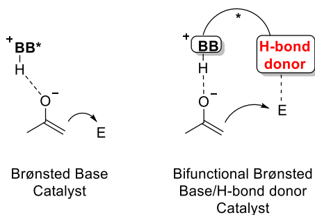
Figure 2.5 Transition states in Brønsted base catalysis and bifunctional Brønsted base/H-bond donor catalysis.
