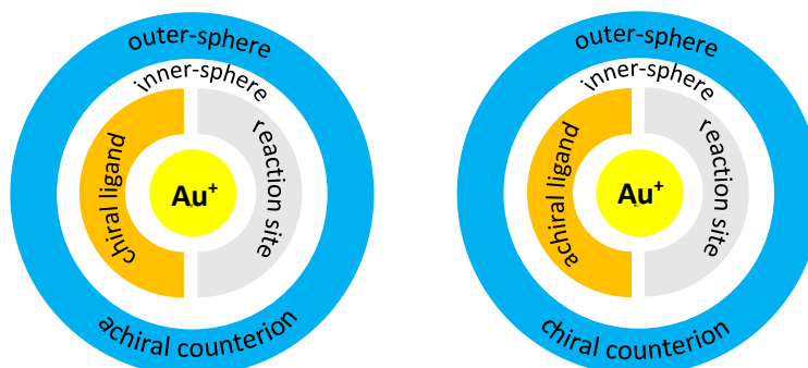
Figure 3.7 Schematic representation of the chiral ligand-based (left) and chiral counterion-based (right) approaches in asymmetric gold catalysis.
