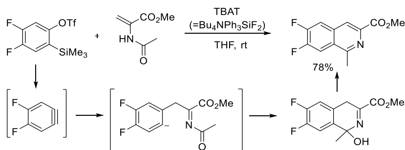
Scheme 4.15 Synthesis of 6,7-difluoroisoquinoline via the reaction of N -acetylenamine with benzyne.
