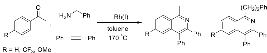
Scheme 4.21 Three-component reaction of aromatic ketone with benzylamine and alkyne affording isoquinolines.
