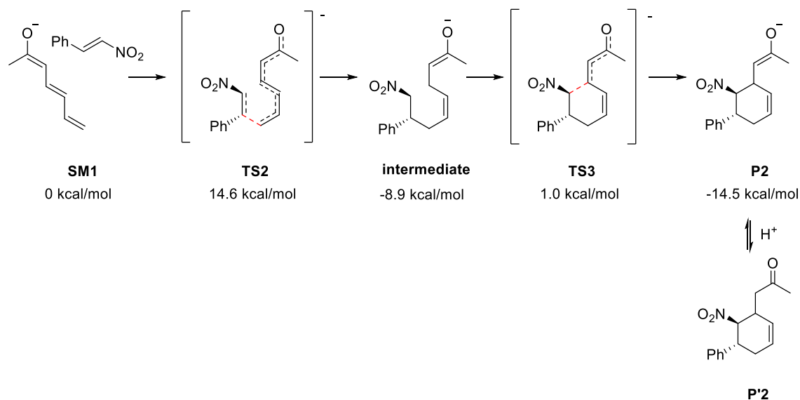
Scheme 2.43 Mechanism of Diels Alder reaction of trienolate and nitroolefin. The energies are Gibbs Energies in kcal/mol.
