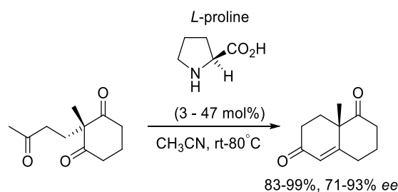
Scheme 2.2 The Hajos-Parrish-Eder-Sauer-Wiechert reaction. 8,9
