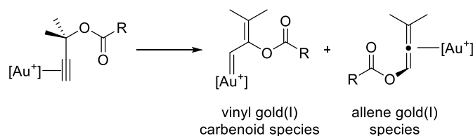
Scheme 3.3 Key intermediates in the propargylic migrations.
