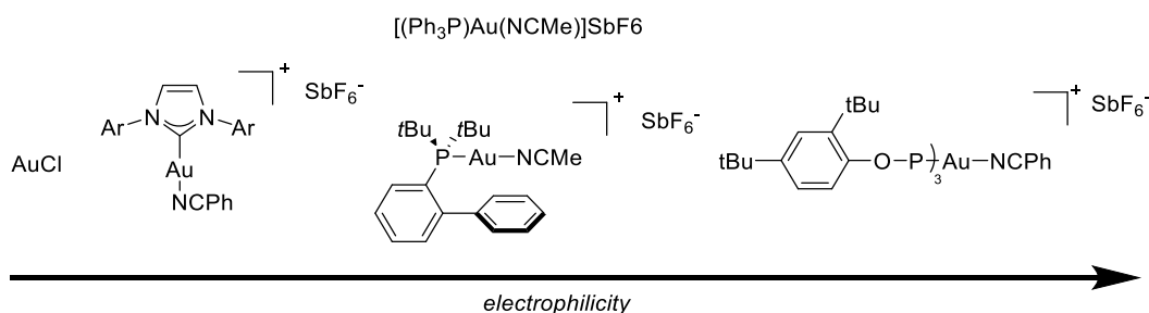
Figure 3.4 Increase in electrophilicity with decreasing donating ligand ability in gold(I) complexes.
