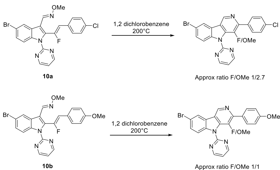
Scheme 4.48 Electrocyclisation for substrates 10a and 10b .
