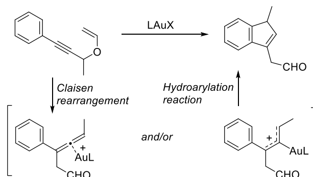
Scheme 3.45 Tandem gold(I)-catalysed Claisen rearrangement/hydroarylation reaction
