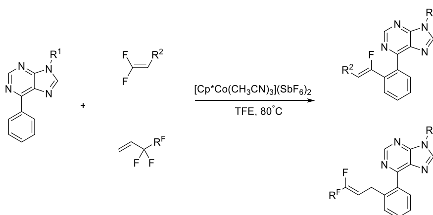
Scheme 4.33 Synthesis of fluorine-containing 6-arylpyridine derivatives via Cp*Co(III)-catalysed C–H bond activation.
