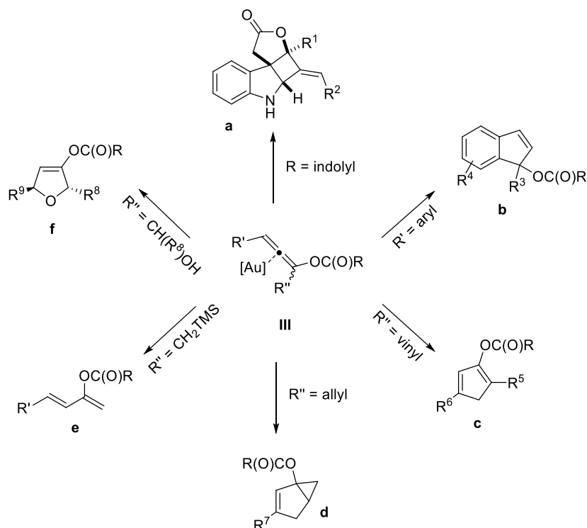
Scheme 3.16 Au assisted allene activation and product diversification.
