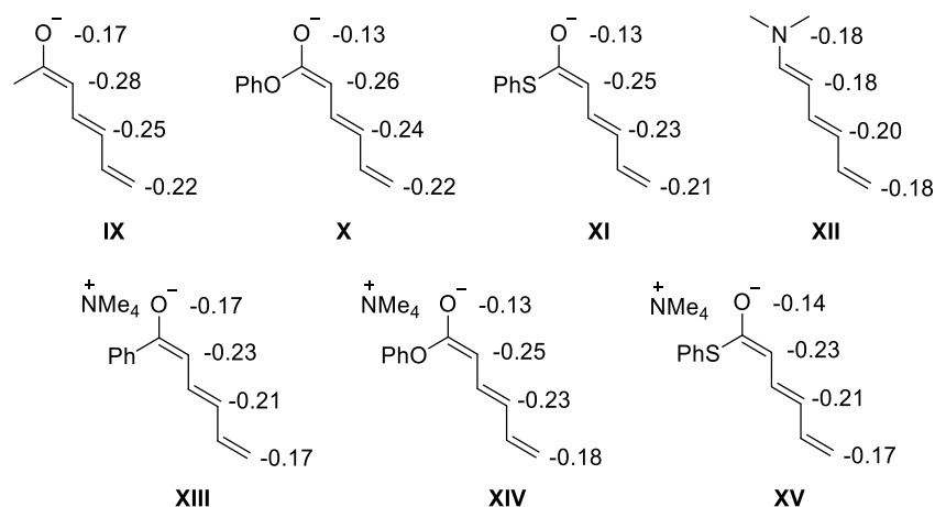
Figure 2.30 Fukui indices of relevant trienolates (alkoxy or ammonium salt form) and trienamine.
