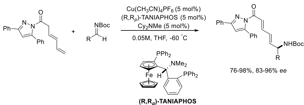
Scheme 2.36 \varepsilon -Selective catalytic asymmetric bisvinylogous Mannich reaction catalysed by a copper(I) complex by Yin et al.
