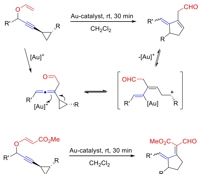
Scheme 3.41 Gold(I)-catalysed Claisen rearrangement – cyclopropyl ring opening – cyclisation.
