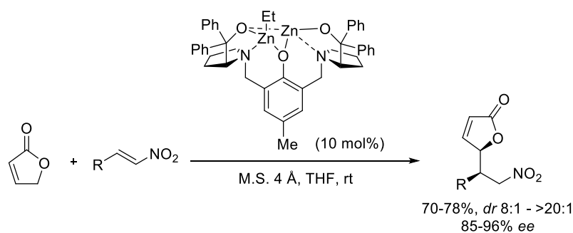
Scheme 2.23 Asymmetric Michael addition of 2(5H)-furanone to nitroalkenes catalysed by a dinuclear zinc catalyst developed by Trost.
