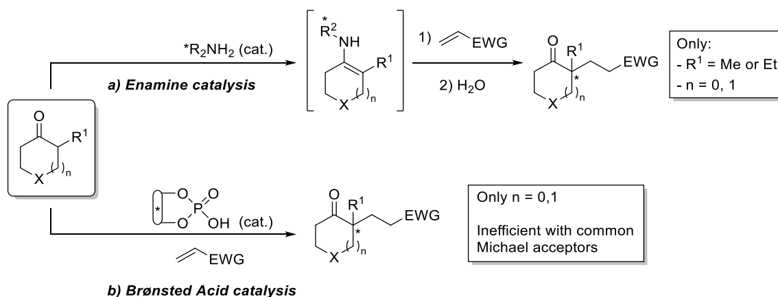
Figure 2.18 \alpha -functionalisation of \alpha -branched cycloalkanones via a) enamine and b) Brønsted acid catalysis.
