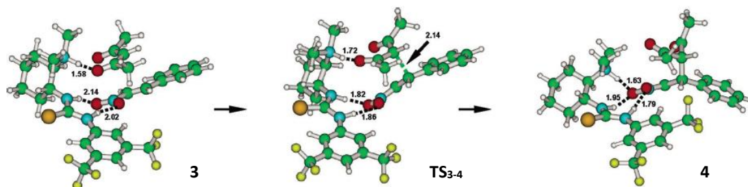
Figure 2.14 Optimised structures and selected geometric parameters of the stationary points located on route A.
