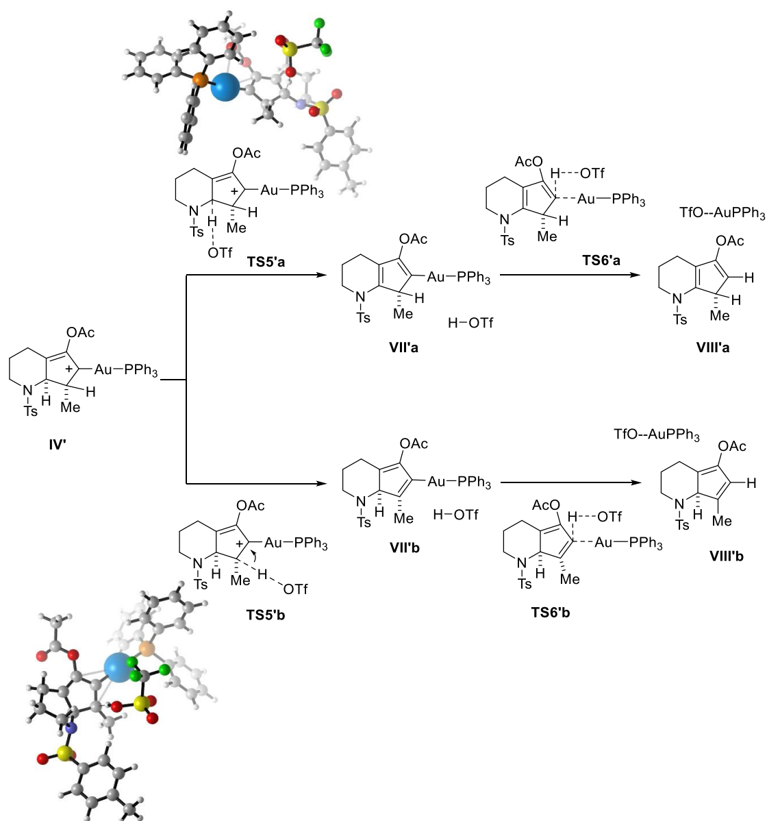
Scheme 3.30 Regioselectivity depending of the H-abstraction.
