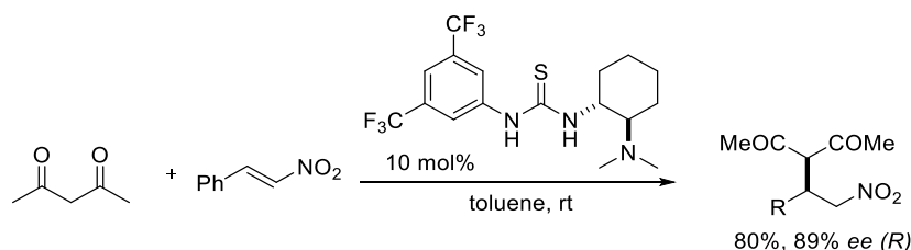
Scheme 2.16 Takemoto reaction (as in Scheme 2.12) considered in the theoretical analysis by Papai.
