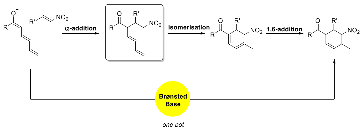
Figure 2.29 One-pot catalytic, enantio- and diastereoselective synthesis of stereodefined six-member carbocycles.
