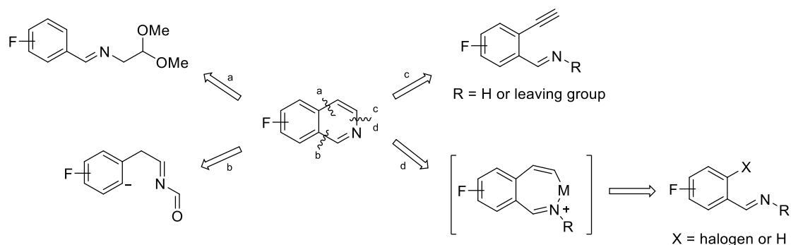
Scheme 4.13 Approaches to fluoroisoquinolines starting from imines bearing a fluoroaryl group.
