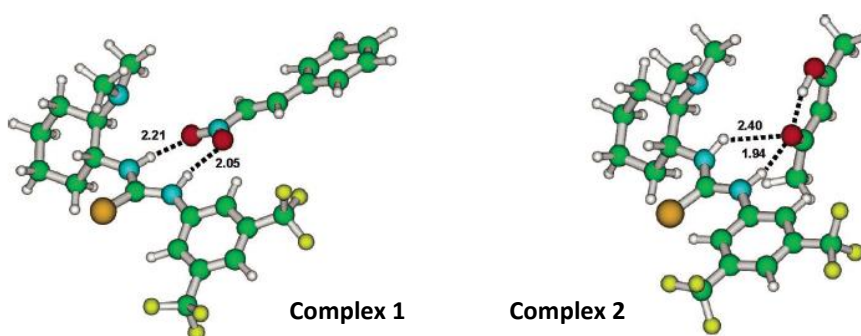
Figure 2.12 Optimised structures of the most stable catalyst-substrate adducts. H-Bond distances in angstroms.
