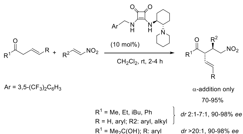
Scheme 2.30 First direct Michael reaction of \beta,\gamma -unsaturated alkyl ketones with nitroolefins to afford exclusively \alpha -addition products under bifunctional Brønsted base/H-bond catalysis by Palomo et al.
