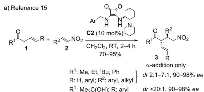
Scheme 2. Impact of ketone side-chain R^1 on the reactivity of derived dienolates.
