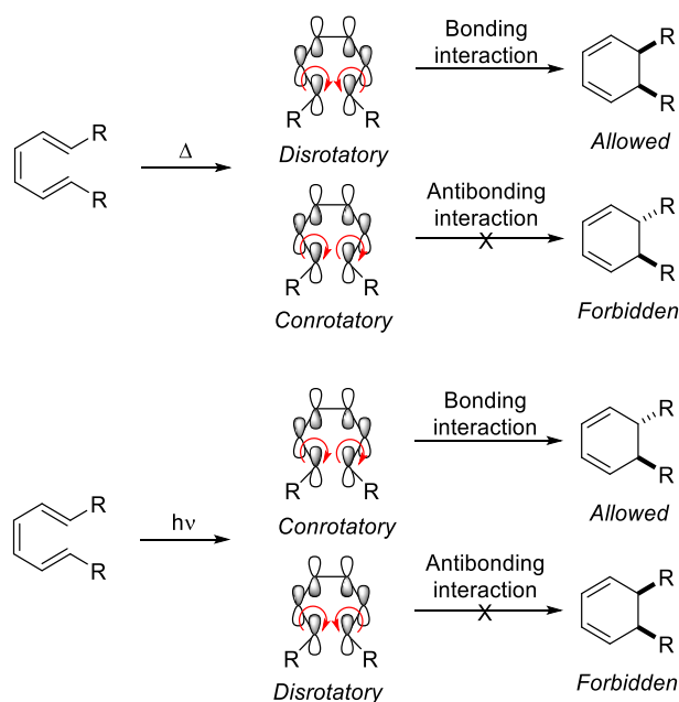
Figure 4.2 Molecular orbital interactions and products distribution for thermal and photochemical 1,3,5-hexatriene cyclisations.
