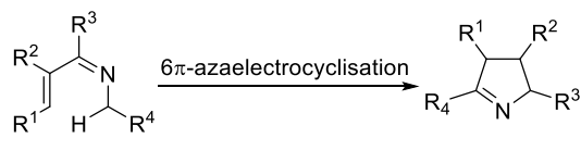
Scheme 4.37 Different 6\pi -electrocyclisations and corresponding heterocyclic products.
