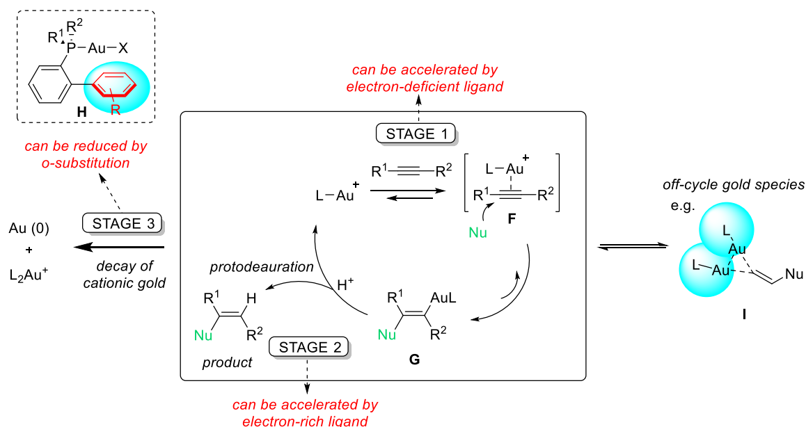
Scheme 3.6 Gold catalytic cycle in three main steps.
