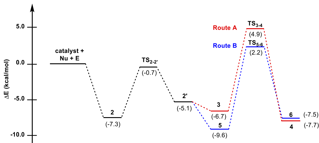
Figure 2.16 Energy profile of the C-C bond formation pathways corresponding to the formation of the ( R ) configuration of products as obtained from gas-phase calculations.
