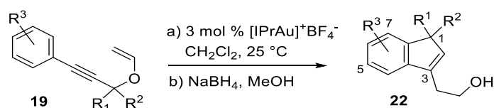
Scheme 3.46 Model reaction for the scope.
