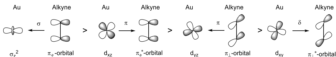
Figure 3.3 Scheme of the Au(I)-alkyne bonding interactions described by the Dewar-Chatt-Duncanson model.
