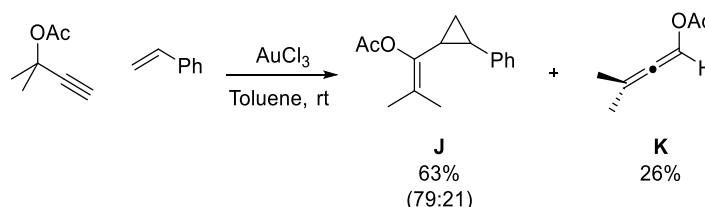
Scheme 3.12 Results of Miki, Ohe and Uemura.
