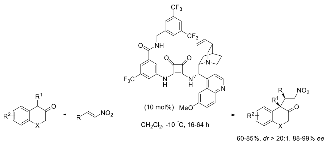
Scheme 2.21 Brønsted base/H-bond-catalysed \alpha -alkylation of \alpha -substituted \beta -tetralones with nitroolefins by Palomo et al.
