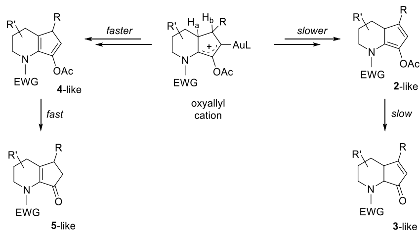
Scheme 3.23 On the top tandem Au(I)-catalysed [3,3]-rearrangement/Nazarov reaction by Occhiato et al. and on the bottom the two competing pathways to 3 - and 5 -like compounds.
