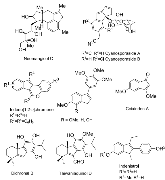
Figure 1. Examples of natural compounds embedding the indene core.
