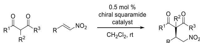
Scheme 2.14 Squaramide catalyzed conjugate addition of 1,3-dicarbonyl compounds to nitroalkenes by Rawal et al. 35
