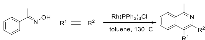
Scheme 4.22 Rh-catalysed synthesis of isoquinoline by Cheng et al.
