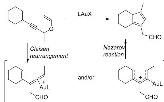
Scheme 3.35 Tandem gold(I)-catalysed Claisen rearrangement/Nazarov reaction.
