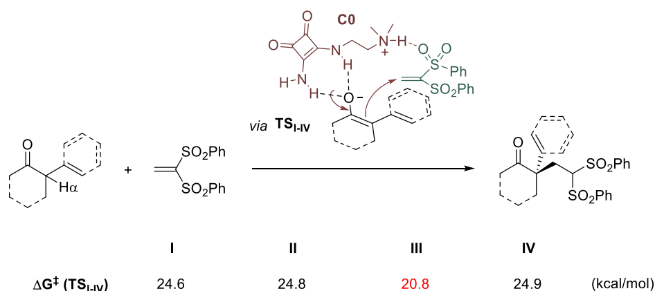
Figure 2.25 Energy barriers for the reactions between ketones I-IV and bis-sulphone 4 in the presence of a model achiral squaramide-tertiary amine catalyst C0 .
