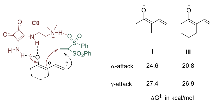
Figure 2.27 \alpha - vs \gamma -reactivity of linear and cyclic \alpha -substituted dienolates in presence of a model catalyst C0 .
