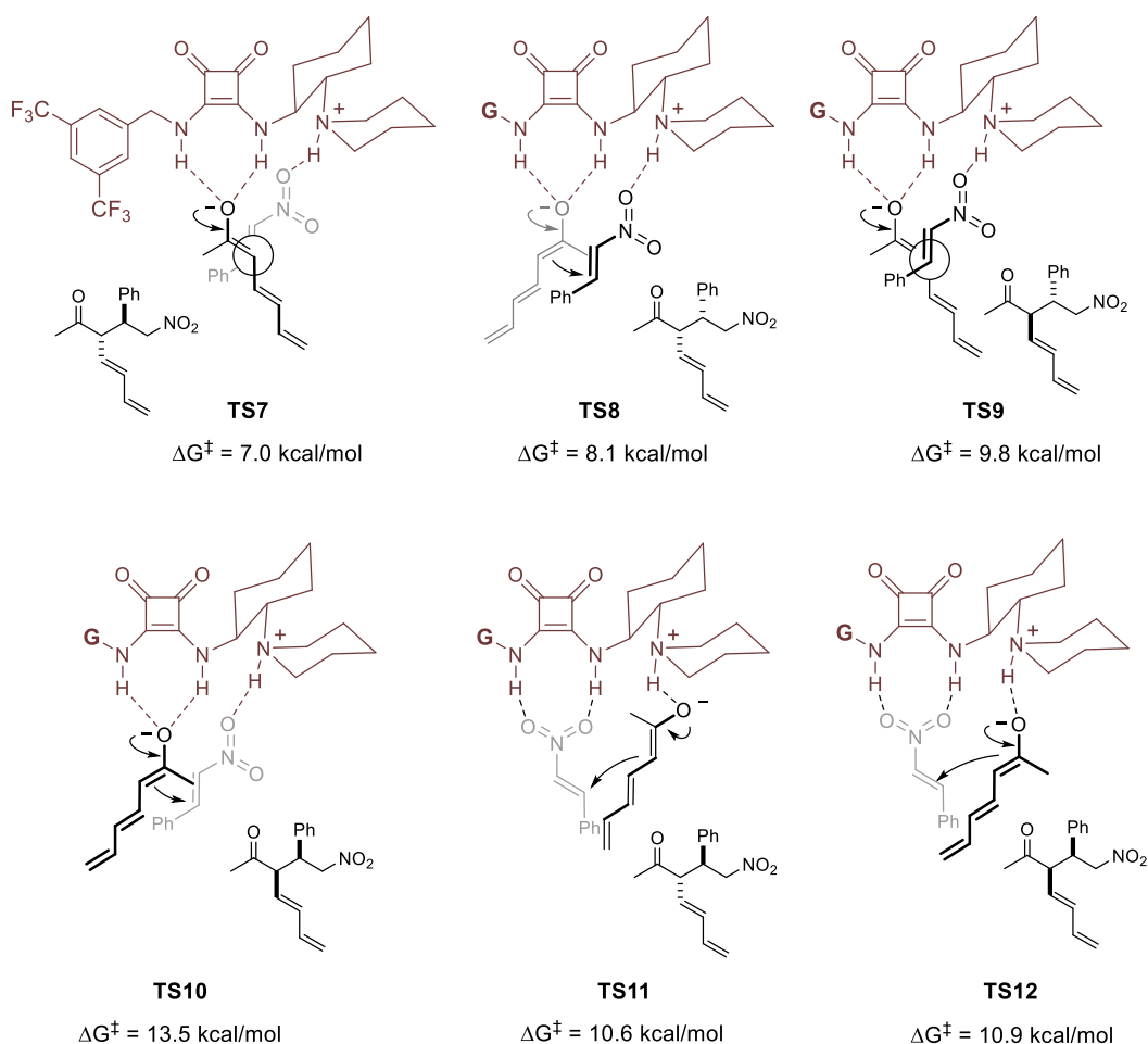
Figure 2.33 Geometries and Gibbs energies of the located TS for the catalysed reaction.
