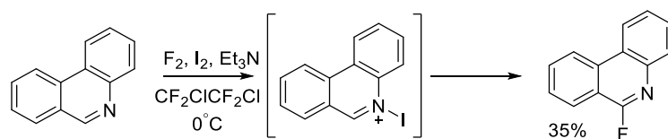
Scheme 4.10 Synthesis of 6-fluorophenanthridine via fluorination with F 2 and I 2 .
