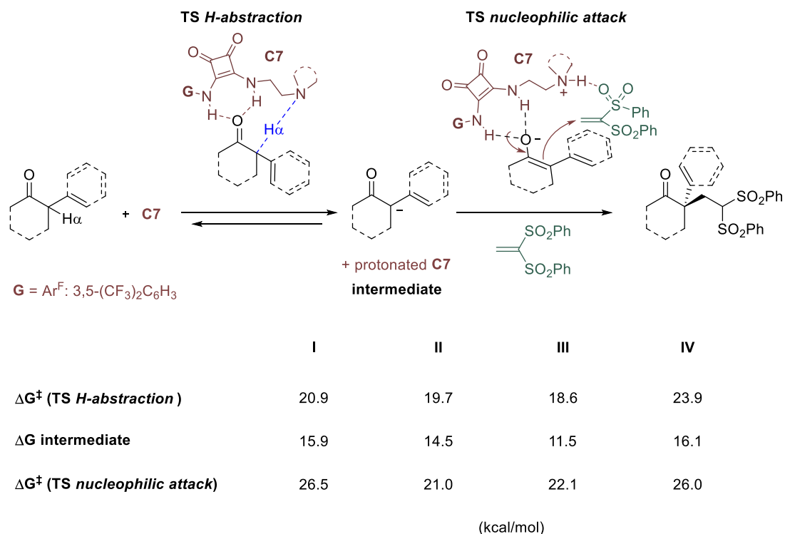
Figure 2.26 Energies for the reaction of ketones I-IV with bis-sulfone in presence of C7 . All the energies are Gibbs Energies in kcal/mol.
