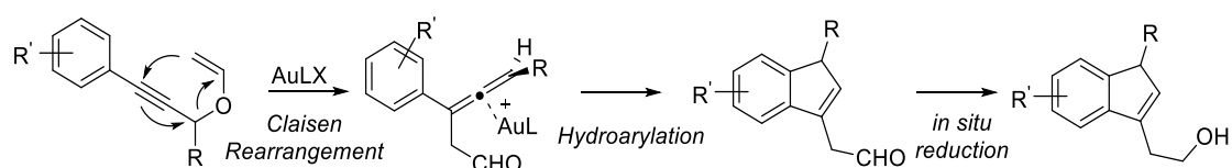
Scheme 3.36 Tandem gold(I)-catalysed Claisen rearrangement/hydroarylation reaction.
