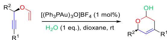
Scheme 3.40 Gold(I)-catalysed synthesis of 2-hydroxy dihydropyrans.
