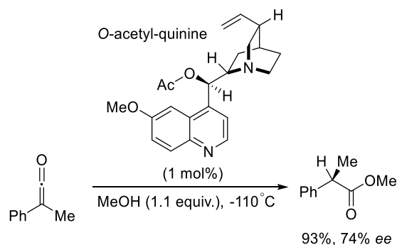
Scheme 2.1 Alkaloid-catalysed addition of methanol to a prochiral ketene by Pracejus et al. 6,7
