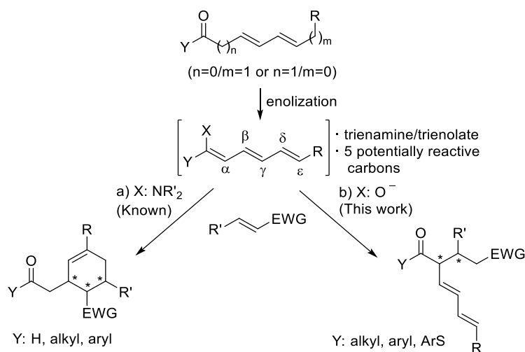
Scheme 2.38 Difference in reactivity between trienamines and trienolates.
