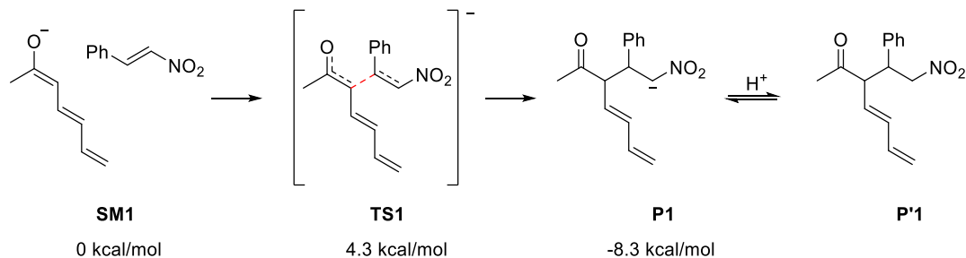
Scheme 2.42 Mechanism of Michael addition of trienolate to nitroolefin. The energies are Gibbs Energies in kcal/mol.
