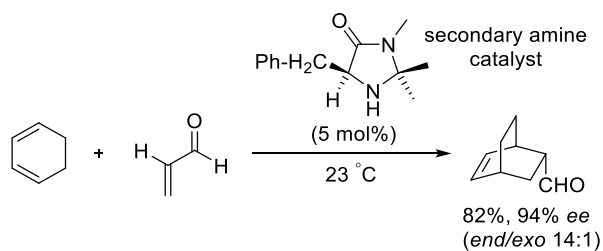
Scheme 2.4 Secondary amine-catalysed Diels-Alder reaction by MacMillan et al. 4
