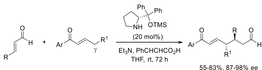
Scheme 2.24 Direct diastereo- and enantioselective vinylogous Michael addition of linear enones by Brenner-Moyer et al.
