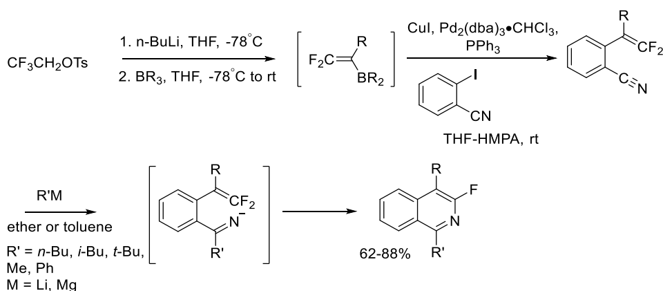
Scheme 4.18 Synthesis of 3-fluoroisoquinolines via intramolecular \text{S}_{\text{N}}\text{V} reaction of iminyl metal intermediates.
