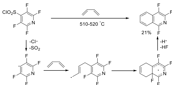
Scheme 4.17 Synthesis of 1,3,4-trifluoroisoquinoline via copolyrlysis of pyridine-4-sulfonyl chloride with butadiene.
