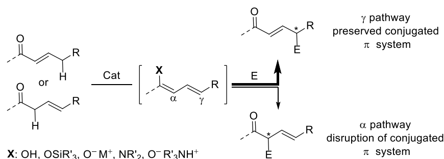
Figure 2.20 Divergent reaction pathways of dienolates and equivalents.
