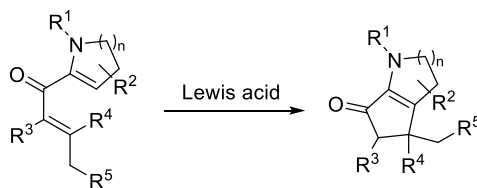
Scheme 3.20 Alternative substrate undergoing Nazarov cyclisation.
