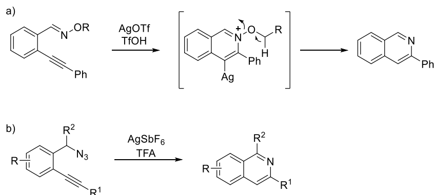
Scheme 4.3 a) AgOTf and TfOH co-catalysed isoquinoline synthesis; b) Ag-catalysed cyclisation of o -alkynyl-benzylazides.
