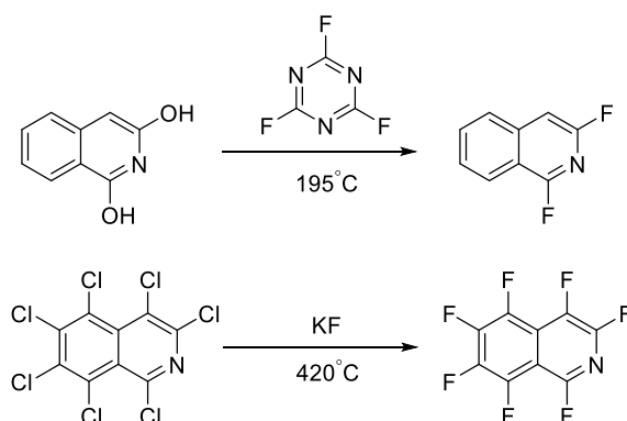
Scheme 4.6 Syntheses of di- and perfluorinated isoquinolines.
