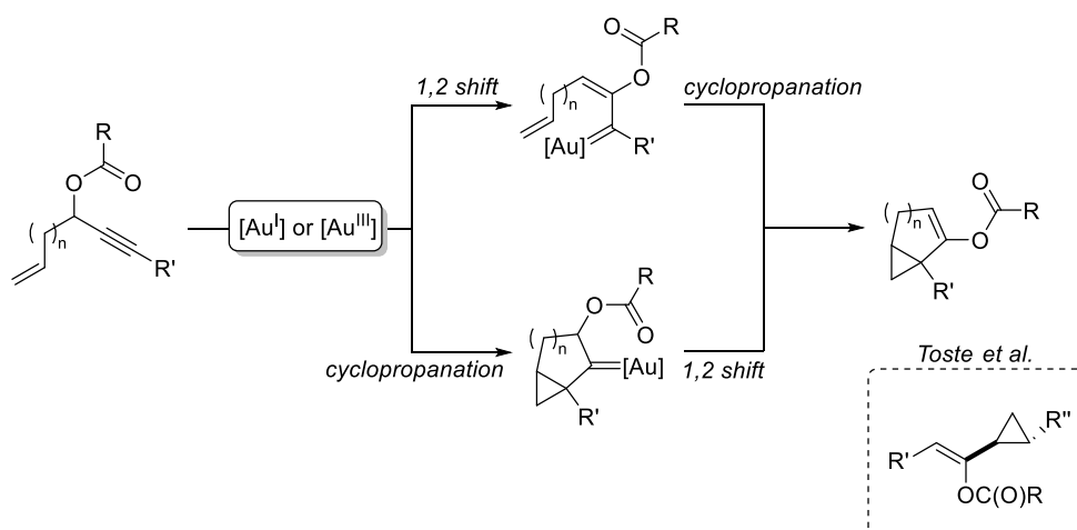
Scheme 3.15 Au-catalysed tandem 1,2-shift/cyclopropanation.
