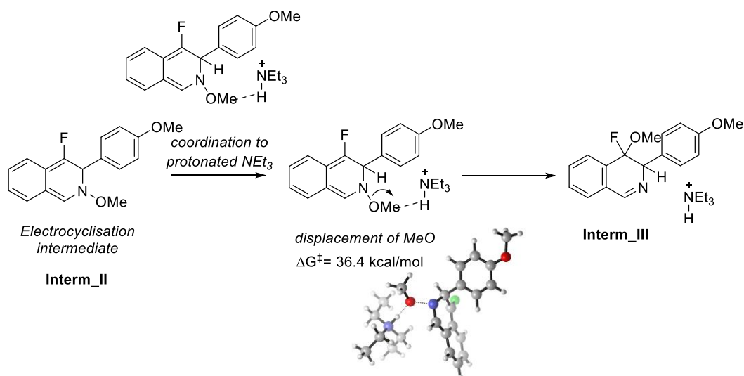
Scheme 4.55 Mechanism mediated by a molecule of protonated Et 3 N as model protonated base present in the reaction media. All the energies are Gibbs energies in kcal/mol using as reference interm_I (Scheme 4.50) with \Delta G = 0 kcal/mol.
