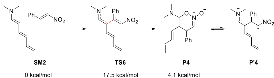
Scheme 2.45 Mechanism of Michael addition of trienamine to nitroolefin. The energies are Gibbs Energies in kcal/mol.
