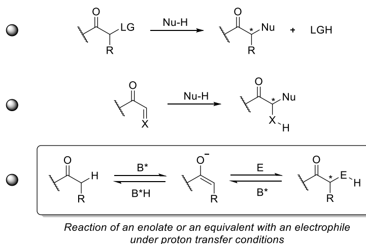
Scheme 2.5 Approches for the stereoselective formation of stereogenic centres at the \alpha -position of a carbonyl compound.
