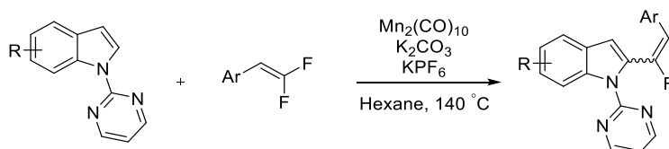
Scheme 4.34 Mn-catalysed synthesis of monofluoroalkenes via C–H activation and C–F cleavage.
