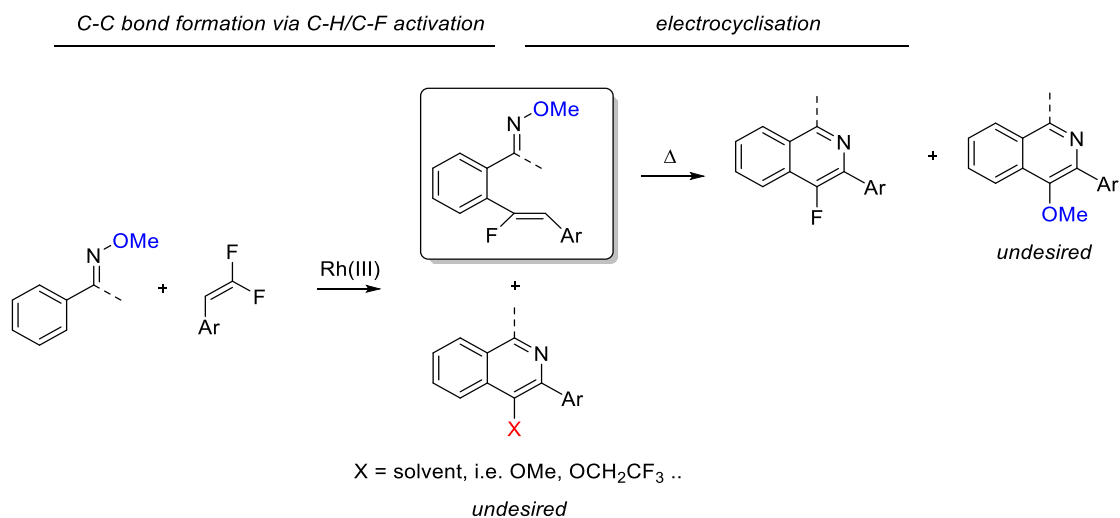
Scheme 4.41 General strategy of our work for the synthesis of fluorinated isoquinolines.
