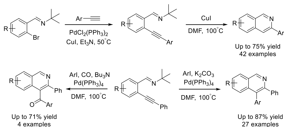
Scheme 4.1 Larock synthesis of isoquinolines.
