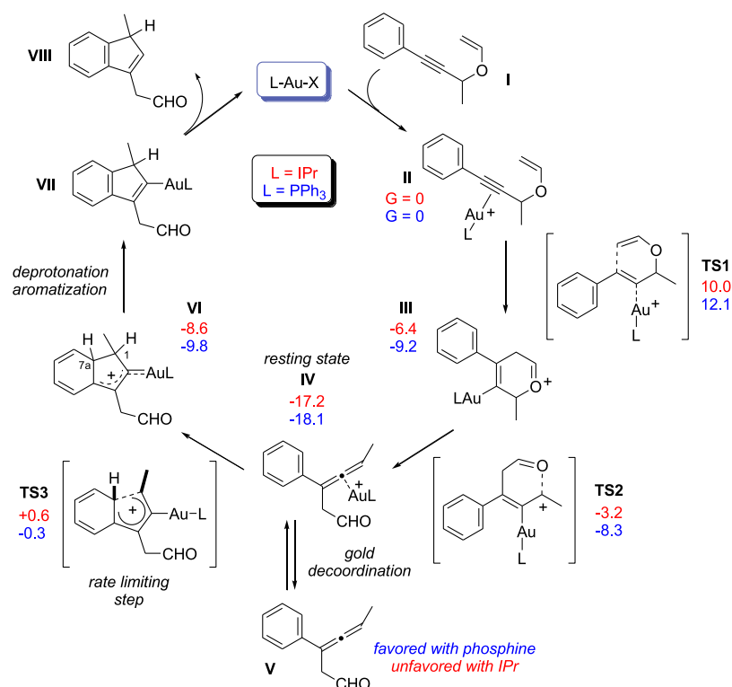
Scheme 6. Catalytic Cycle with Calculated Energies a
