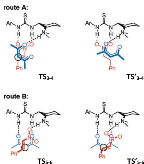
Figure 2.17 Transition States leading to the R and S isomers of Michael products on the two alternative routes.
