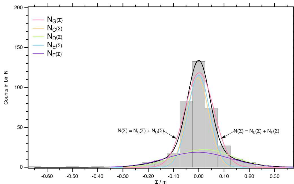
Figure E1. Histogram of the difference data with cubic spline interpolation \Sigma_i = S(D_1, \dots, D_{k-1}, D_{k+1}, \dots, D_n) - S(D_1, \dots, D_i, \dots, D_n) for the match points between EGRIP and NGRIP1/2.
