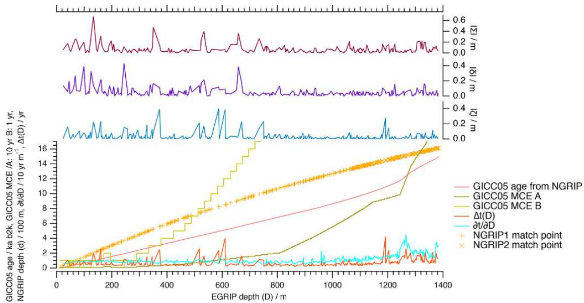
Figure E2. The (EGRIP, NGRIP) match points, the (EGRIP depth, GICC05 time) scale, the (EGRIP depth, GICC05 MCE) curve, |\delta| , |\Sigma| , |\zeta| , \frac{\partial t_{\text{GICC05}}}{\partial D_{\text{EGRIP}}} , \Delta t(D) = \left| \frac{\partial t}{\partial D} \right| \sqrt{(\Delta t)^2 + \zeta^2} .
