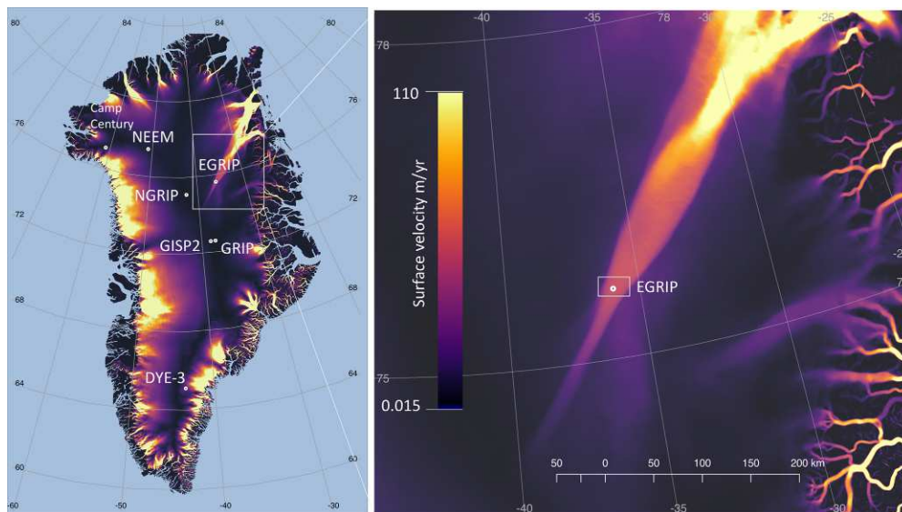
Figure 1. Locations of deep ice-core drill sites: EGRIP, NEEM, NGRIP, GRIP, GISP2, DYE-3 and Camp Century in Greenland, and close-up of the EGRIP drill site inside the Northeast Greenland Ice Stream (NEGIS). Colours show surface flow velocities from satellite data (Joughin et al., 2018).
