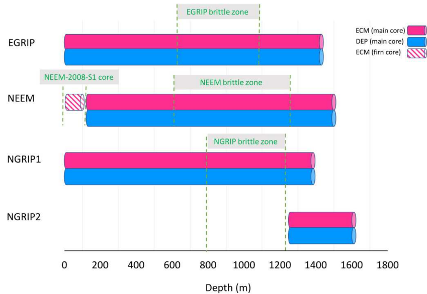
Figure 2. Overview of DEP and ECM that we used for the synchronization between ice cores over the Holocene and late last glacial periods.
