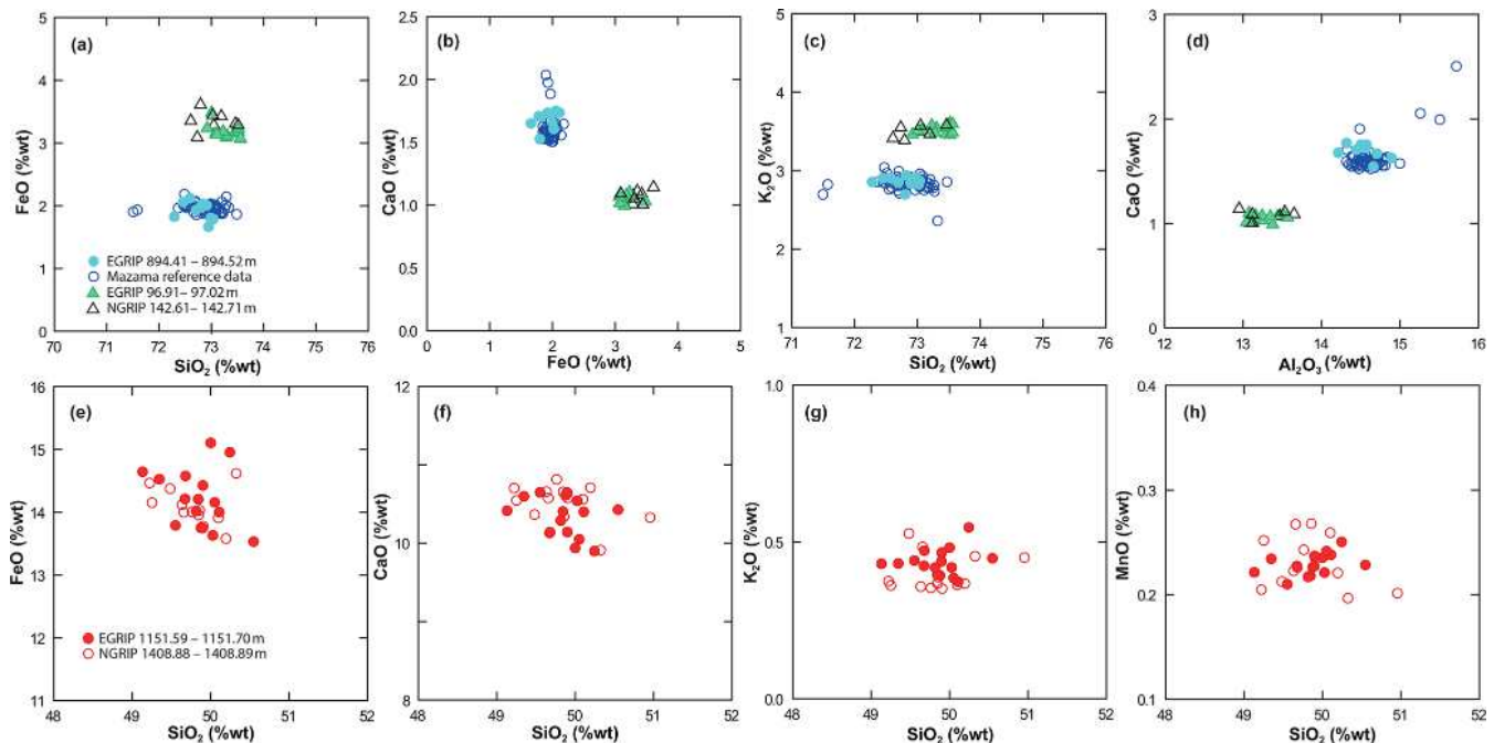
Figure 7. Element–element biplots showing geochemical matches between EGRIP and NGRIP samples with the exception of EGRIP at 894.41–894.52 m (EGRIP bag 1627), which is shown here with Mazama data from Jensen et al. (2019). Geochemical data are normalized to 100 % (anhydrous basis), and analyses with totals below 94 %wt were excluded. Panels (a–d) are for EGRIP bags 177 and 1627; panels (e–h) are for EGRIP bag 2094.
