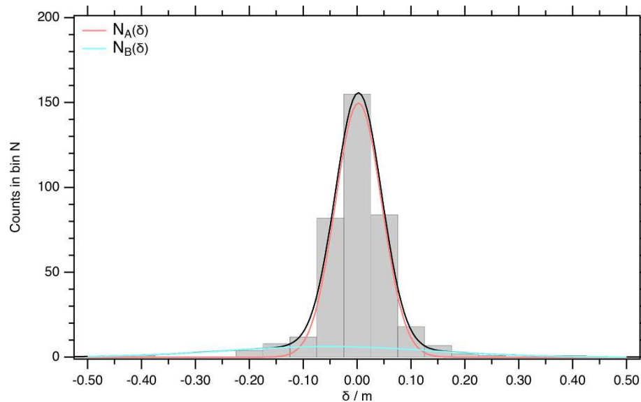
Figure D1. Histogram of the difference data with linear interpolation \delta_i = (D_{i+1} - D_{i-1}) / (d_{i+1} - d_{i-1})(d_i - d_{i-1}) + D_{i-1} - D_i for the match points between EGRIP and NGRIP1/2.
