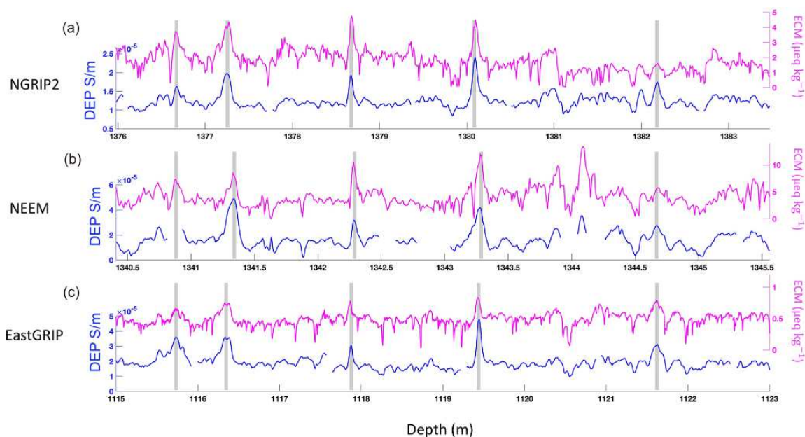
Figure 8. Example of the ECM and DEP data match between the NGRIP2 (a), NEEM (b) and EGRIP (c) cores. The match points are marked by grey bands.
