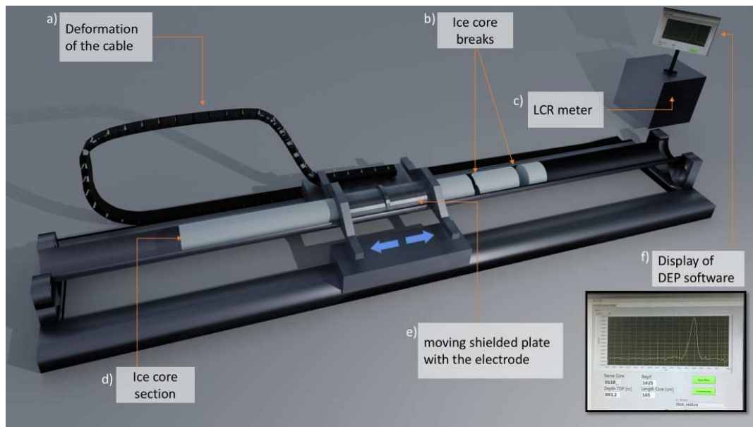
Figure 4. Schematic of the DEP instrument.
