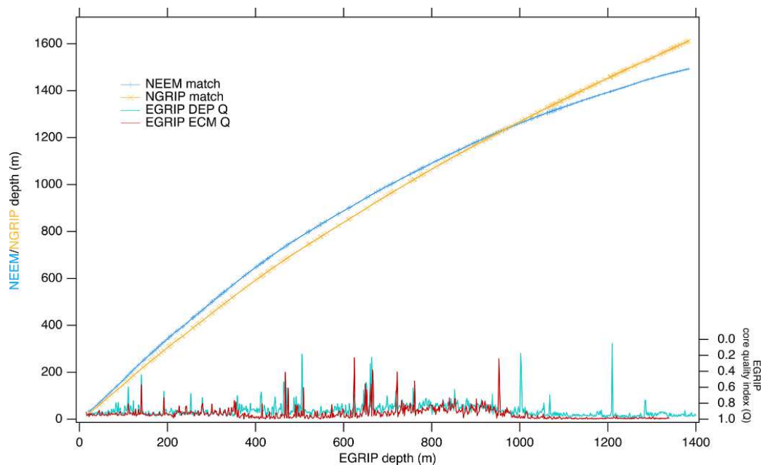
Figure 3. Match points between EGRIP, NEEM (blue) and NGRIP (yellow) ice cores based on the DEP and ECM data sets. The core quality index Q is derived from the validated DEP (blue) and ECM (red) data, respectively.
