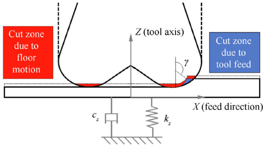
Fig. 4 Milled zones generated by axial motion of part sample.
