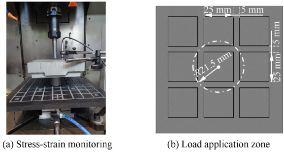
Fig. 1 Compression test set up.
