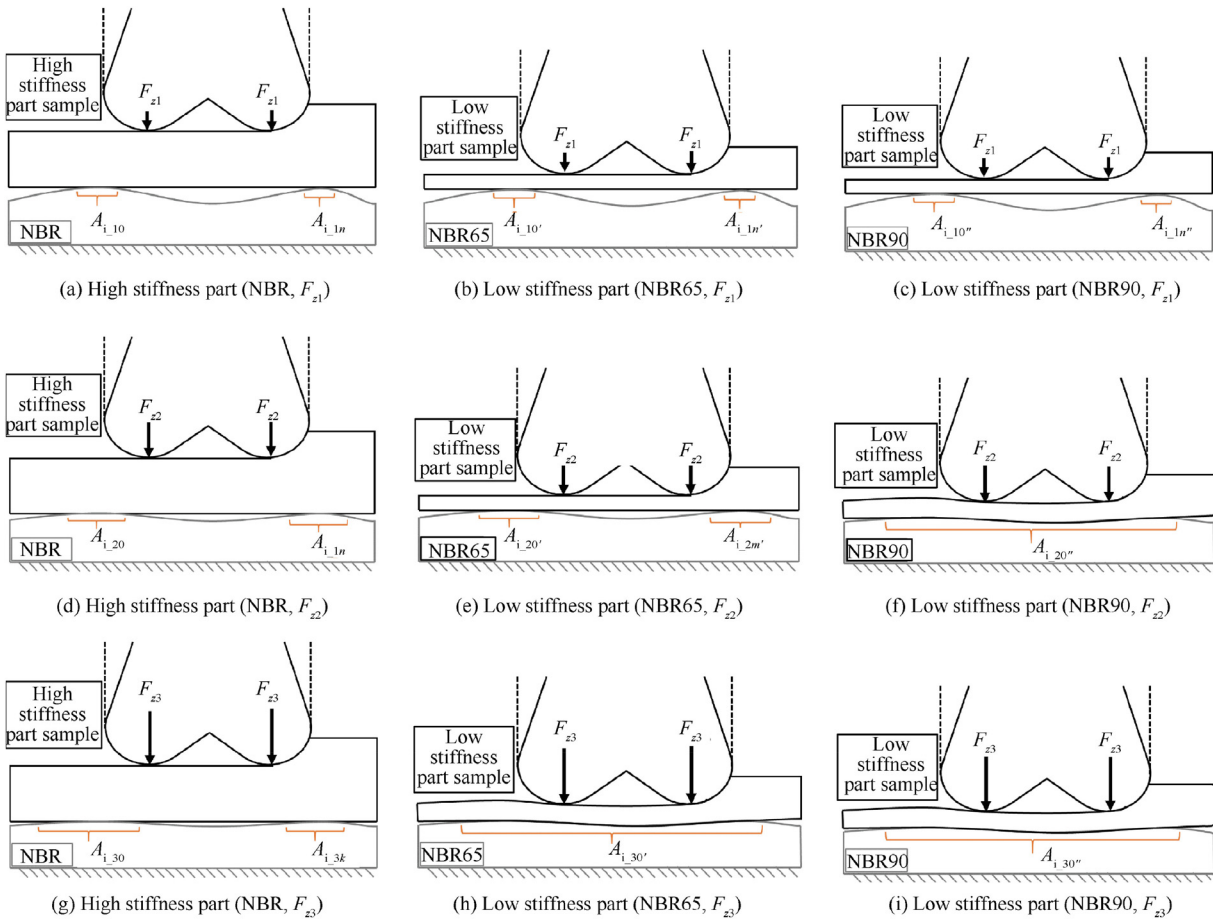
Fig. 6 Clamping suitability evolution for high and low stiffness parts with NBR65 and NBR90 fixtures.
