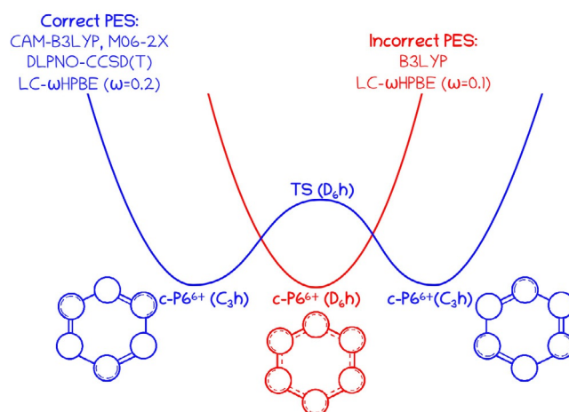
Figure 2. Sketch of the potential energy surface of c-P6 6+ around the energy minimum as described by different DFAs.
