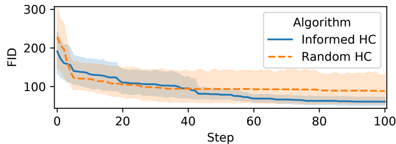
Fig. 4.6: Evolution of the FID (in the y axis) of the best CNN-GAN structure found at each step (x axis). The solid line represents the median of all 30 runs. The translucent bands represent the 95% confidence interval. The broken orange line represents runs performed with the random hill climbing, whereas the blue continuous line does so for the hill climbing guided by the metamodel.
