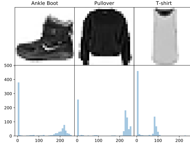
Fig. 5.3: This figure displays three gray-scale images that correspond to three different examples in the fashion-MNIST database. Their respective titles show what class they belong to (those used for the classification task), whereas the bar plots show the 32-bin-histograms representing the frequency (y axis) of pixel values (x axis) in the image (used for the regression task). The clothing image itself is used for the sampling task.
