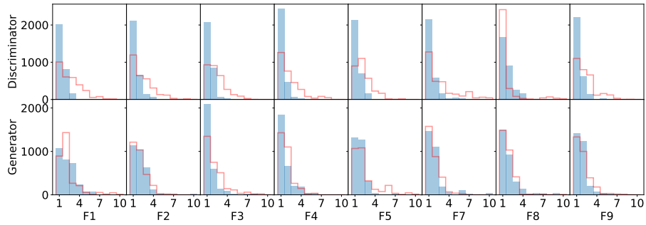
Fig. A.6: Number of layers present in the two networks of fully evolved GANs, for all functions with both problem dimensions.
