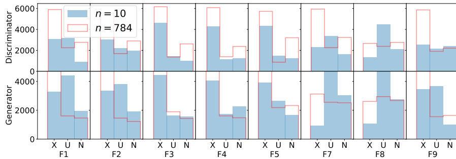
Fig. A.4: Initialization functions present in the two networks of fully evolved GANs, for all functions with both problem dimensions. X: Xavier initialization, U: random Uniform, N: random Normal.
