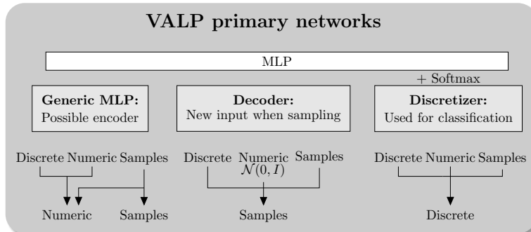
Fig. 5.1: Primary networks and their functionality inside VALP. The decoder must take (at least) numeric values when training. When running the model, these values are replaced with samples from a \mathcal{N}(0, I) distribution to ensure that the Decoder can create new data.
