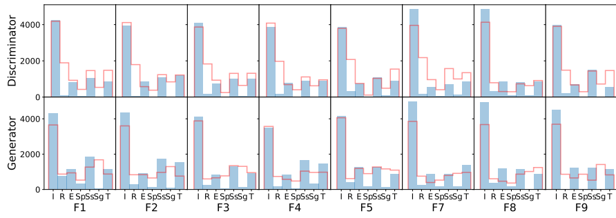
Fig. A.5: Activation functions present in the two networks of fully evolved GANs, for all functions with both problem dimensions. I: Identity function, R: Rectified linear unit, E: Exponential Linear Unit, Sp: Softplus function, Ss: Softsign function, Sg: Sigmoid function, T: Tanh function.
