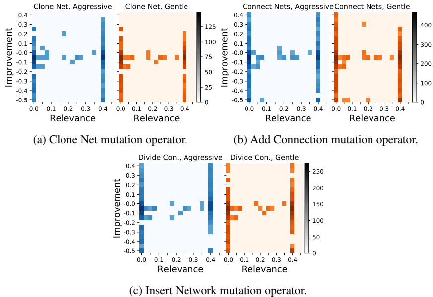
Fig. 6.5: Percentage improvement observed over the regression output of the VALP in logarithmic scale (in the y axis), by different mutation operators, with respect to the relevance of the network affected by the operator, also in logarithmic scale (x axis, the larger, the more relevant a network to the output).
