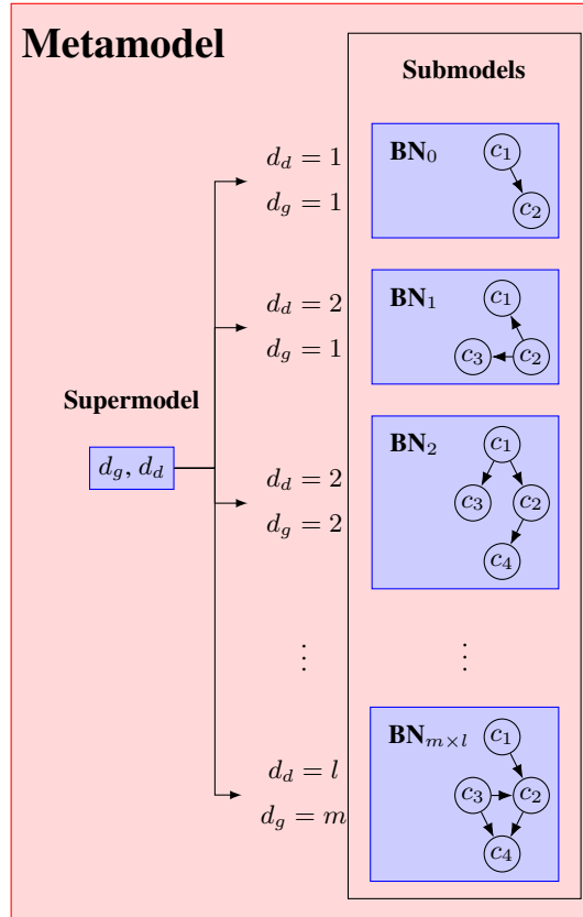
Fig. 4.1: Graphical representation of the metamodel. This visualization assumes that the generator and the discriminator are codified within a single individual. If the DNNs were evolved separately, a single submodel per DNN per depth would be required. The example BN graphs do not represent a realistic scenario in terms of number of nodes. An example of a BN submodel learned for the metamodel can be seen in Figure 4.2. l and m represents the maximum number of hidden layers in the discriminator and generator, respectively. The c_n represent the different components in a GAN.
