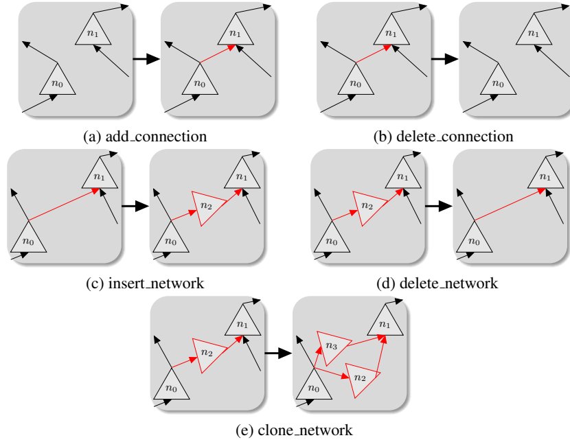
Fig. 6.1: Examples of the different operators. In all cases, the variation is performed relative to the VALP component in the middle of the figure (in red). For Figures 6.1a, 6.1b, and 6.1c, a connection. For Figures 6.1d, and 6.1e, a network ( n_2 ).
