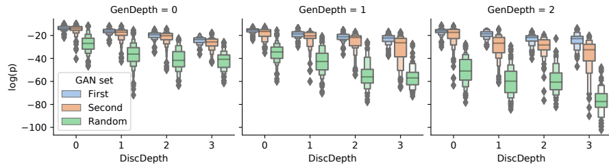
Fig. 4.3: Probabilities (in logarithmic scale) provided by the metamodel to GANs present in the three defined sets.
