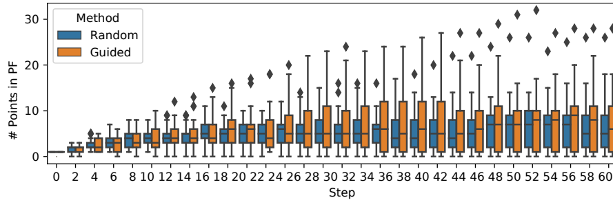
Fig. 6.6: Boxplot showing the number of points (y axis) in the PFs generated from combining the pairwise HC runs (blue for random, orange for guided), per step (x axis).
