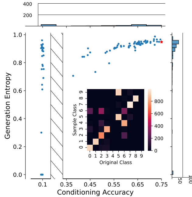
Fig. 5.6: Sampling performance of the 100 VALPs according to conditioning capability and distribution over the possible classes. The red star represents the VALP configuration with the largest conditioned accuracy. The small heatmap represents a confusion matrix, comparing the class of the conditioning examples and the generated sample images by the VALP represented with the red star.
