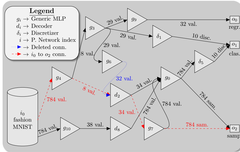
Fig. 5.7: Schematic representation of the VALP configuration that showed the maximum conditioning from the input example in the produced sample. The arrow tags represent the size of the data; how many variables there are, “val.” stands for numeric values, “disc.” are discrete values, and “sam.” stands for samples. The dashed red lines denote the conditioning path. The dotted blue lines denote connections that are removed and replaced with \mathcal{N}(0, I) when running the model.
