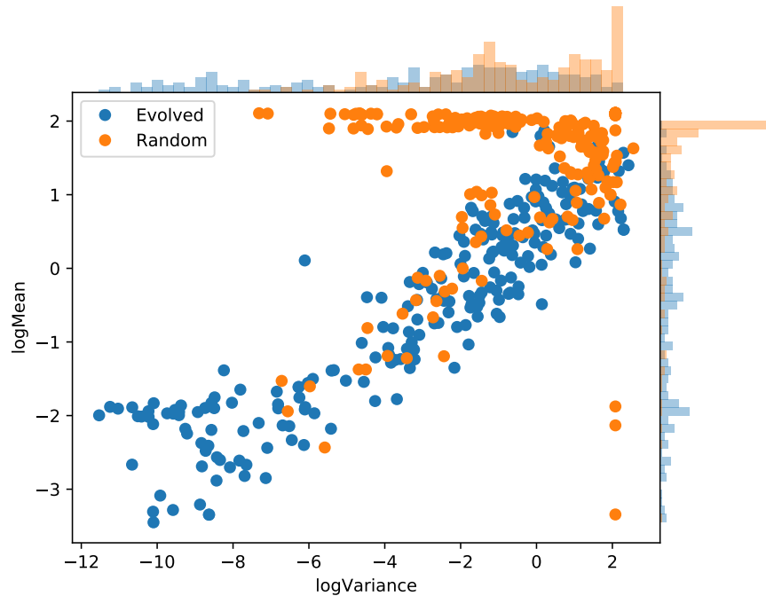
Fig. 3.11: Plot showing the distribution of the variances and the means of the 5-repetition sets. Marginal distributions are also shown.
