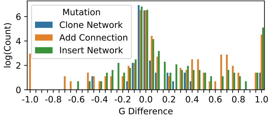
Fig. 6.3: Frequency (y axis, in logarithmic scale) of the G difference values (x axis) observed when comparing the improvements obtained by VALPs after being modified by gentle operators, and their aggressive versions. Positive values indicate a better performance of the gentle operator, whereas negative ones do the exact opposite. Larger numbers represent larger differences between operators.
