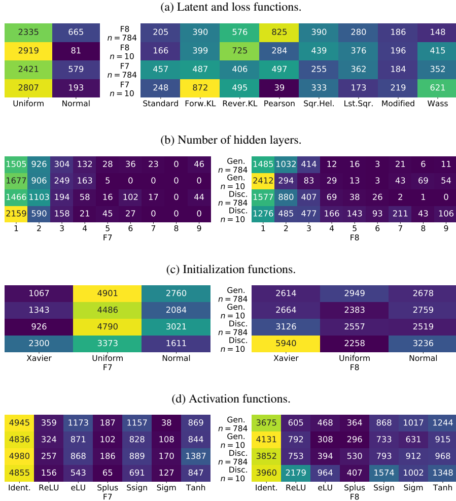
Fig. 3.12: Different characteristics present in the GANs evolved in the last populations of all 30 runs. The x axis represents the different choices for each component, and the numbers and colors represent the appearance frequency on the GANs (the lighter, the more frequent). Colors maintain consistency within subfigures, with the exception of Figure 3.12a, where the color palette is independent for the left and right-hand sides of the subplot.
