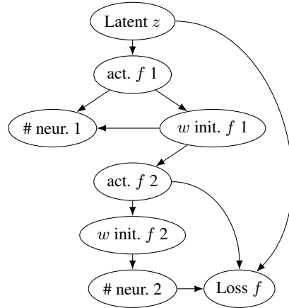
Fig. 4.2: Submodel example. In this case, for the sake of simplicity, only one network of two layers is represented (composed of the number of neurons, the activation function, and the weight initialization function). Two other key components of a GAN, the distribution of the latent variable and the loss function used to train the model are also included.
