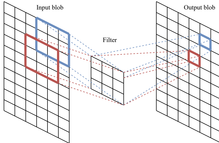
Fig. 2.2: Example of a single filter performing over a 2D blob.
