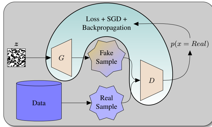
Fig. 3.1: Schematic representation of GAN. The generator network G receives a random noise input for transforming it into a sample as similar as possible to the real ones. The discriminator receives samples both from the original dataset and the generator and attempts to distinguish them apart. Finally, the weights are updated in both networks depending on the ability of the discriminator. Examples correctly classified affect the weights in the generator, whereas the misclassified ones serve for improving the discriminator.
