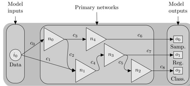
Fig. 5.2: Schematic representation of a VALP.
