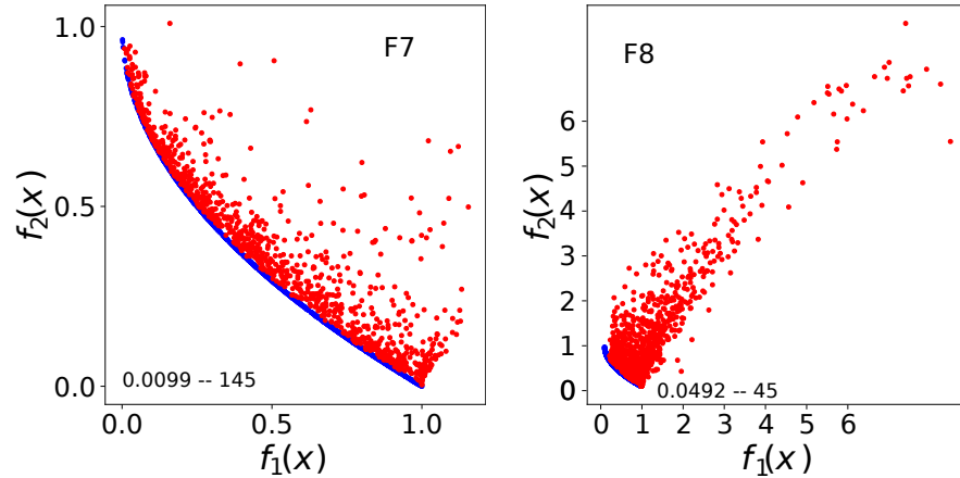
Fig. 3.6: Two PF approximation examples with n = 10 in both cases. The line formed by the blue points shows the true PF, and the approximation made by the GAN is represented in red. The x and y axis represent the values achieved in each objective functions by the best approximation found in two random runs for F7 (left) and F8 (right).
