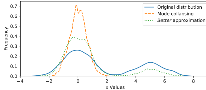
Fig. 3.2: Mode collapsing example.
