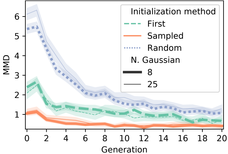
Fig. 4.5: Best MMD value (y axis) corresponding to the samples generated by GANs at different generations (x axis) during the evolutionary procedures. The solid lines represent the mean of the 20 individuals \times generation \times 30 runs = 600 computed MMDs at each generation, whereas the translucent bands show the 95% confidence interval of all these runs. Runs for the 2 variations of the problem and three NE initialization methods are displayed.
