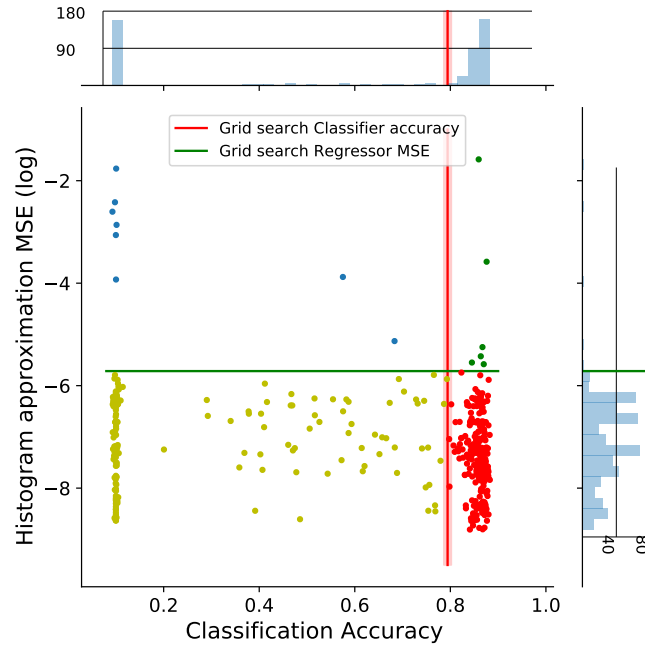
Fig. 5.4: Performances of the models plotted in terms of both classification accuracy and MSE reached on the regression problem. The vertical red line represents the performance of the MLP specifically learned for the classification problem. The horizontal green line represents the performance of that same MLP extended for addressing the regression problem. Blue points represent VALP configurations that performed worse than both baselines, yellow points are models that improved only the regression problem results, and models represented in green did so in the classification problem. The red ones offered better results than both baselines.
