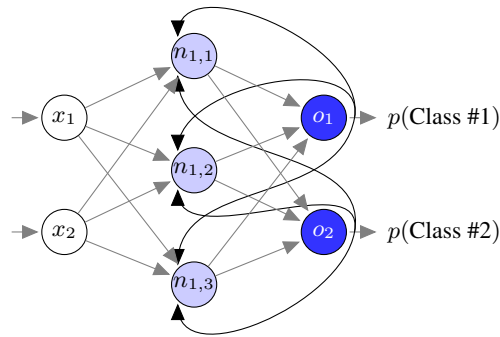
Fig. 2.3: Schematic representation of a minimalist RNN of a single layer, in which the output of the network is redirected to the neurons in the hidden layer.
