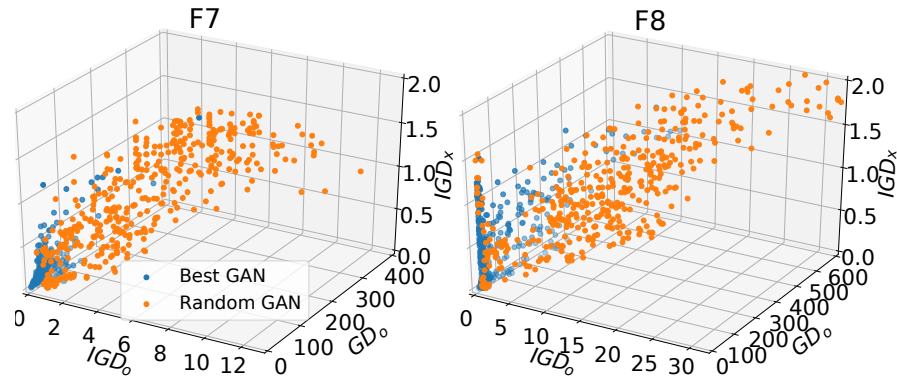
Fig. 3.8: Scatter plots showing the IGD_o , IGD_x and GD_o obtained by the best GANs for F7 and F8.
