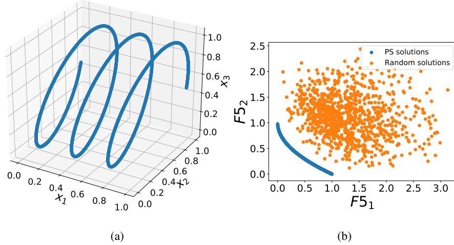
Fig. 3.3: First three decision variables of points known to be in the PS of F5 (left). Comparison of these variables in the objective space, i.e., the PF, to random generated decision variables (right).
