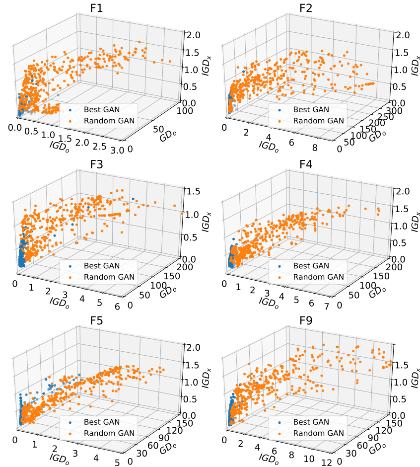
Fig. A.1: Relation of IGD_o , IGD_x , and GD_o for functions F1 , F2 , F3 , F4 , F5 , and F9 .
