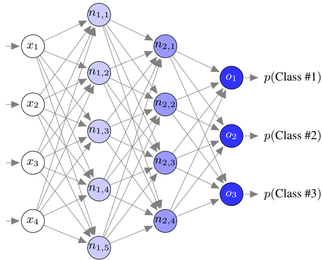
Fig. 2.1: Schematic representation of a DNN for a three-class classification problem. An observation (represented by its features) is placed in the input of the network and is subjected to a list of matrix transformations as well as a possible application of a non-linear activation function. Each arrow represents one scalar multiplication. The first index in the neurons is the layer they belong to. Each neuron n performs a summation of all the incoming values. The output layer (in the general case) consists of one neuron per possible class, each being interpreted as the probability of the observation placed in the input belonging to a certain class (if activated with a softmax function).
