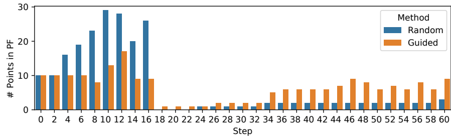
Fig. 6.7: Barplot showing the number of points (y axis) in the combined PF from each approach (blue for random, orange for guided), per step (x axis).
