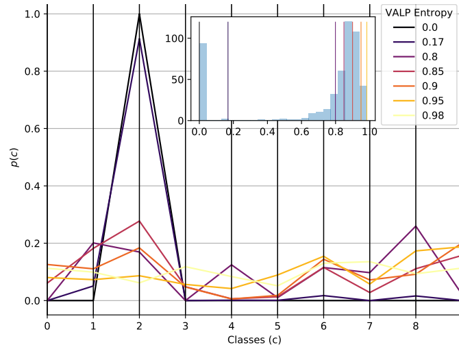
Fig. 5.5: The box in the top shows the distribution of entropy values of the 500 VALP configurations, and the seven representative VALP examples (the vertical lines). Each representative example is displayed by a vertical line. The probabilities of generating a sample of a certain class by each representative example are shown in the general parallel coordinates.
