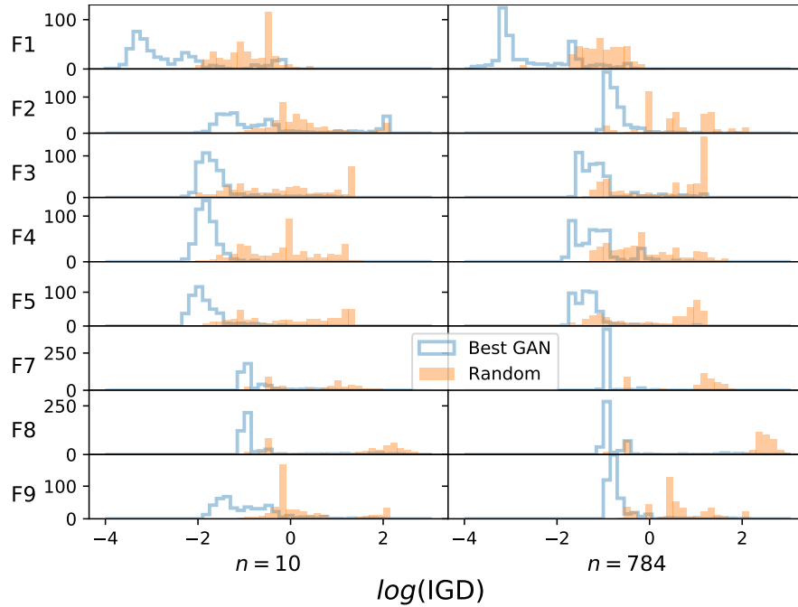
Fig. 3.7: Histograms showing the 30 \text{ GANs} \times 15 \text{ runs} = 450 IGD values (in logarithmic scale, the lower, the better) computed for each function (y axis), for the two problem dimensions (x axis). Solid orange lines describe results obtained by a random GAN, whereas the blue contour display the results obtained by the evolved GANs.
