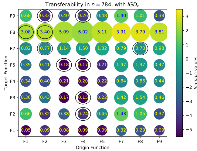
Fig. A.2: Transferability of the best GANs evolved with n = 784 across different functions.
