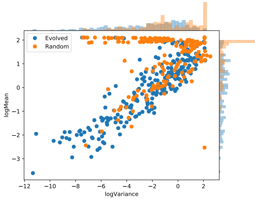
Fig. A.3: Transferability of GANs evolved with functions with n = 784 .
