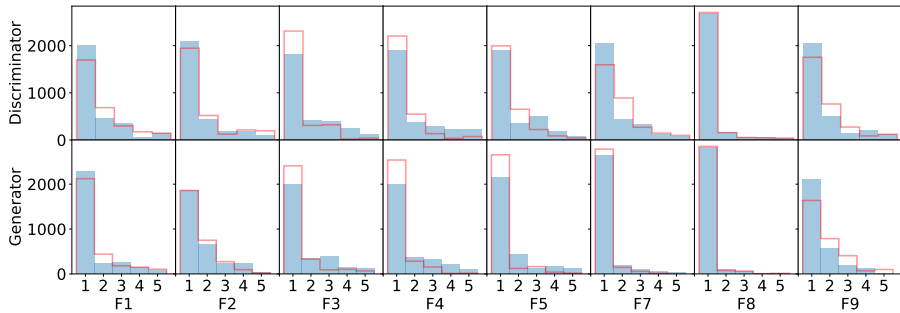
Fig. A.9: Loop parameters used by the fully evolved GANs, for all functions with both problem dimensions.
