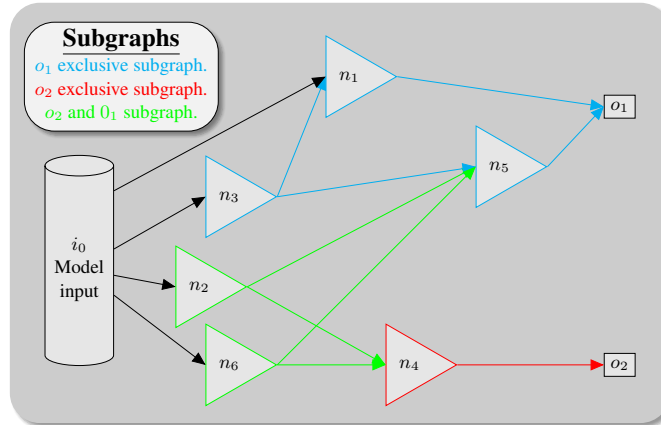
Fig. 6.2: Example of a VALP, with its different subgraphs. The n_1 , n_3 , and n_5 sub-DNNs would be part of the exclusive subset of o_1 , as they are exclusively connected to o_1 . Idem for the n_4 sub-network and o_2 . Adding the n_2 and n_6 sub-DNNs to either subset would result in o_1 and o_2 subsets respectively, as these would contain all the sub-networks involved in these outputs, including sub-DNNs which are involved in other outputs.
