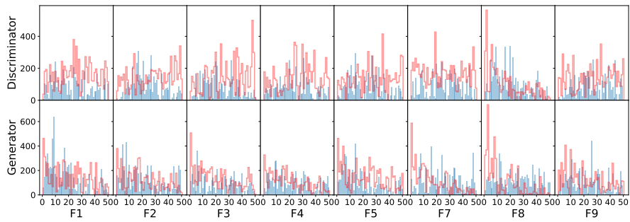
Fig. A.8: Layer sizes used by the fully evolved GANs, for all functions with both problem dimensions.
