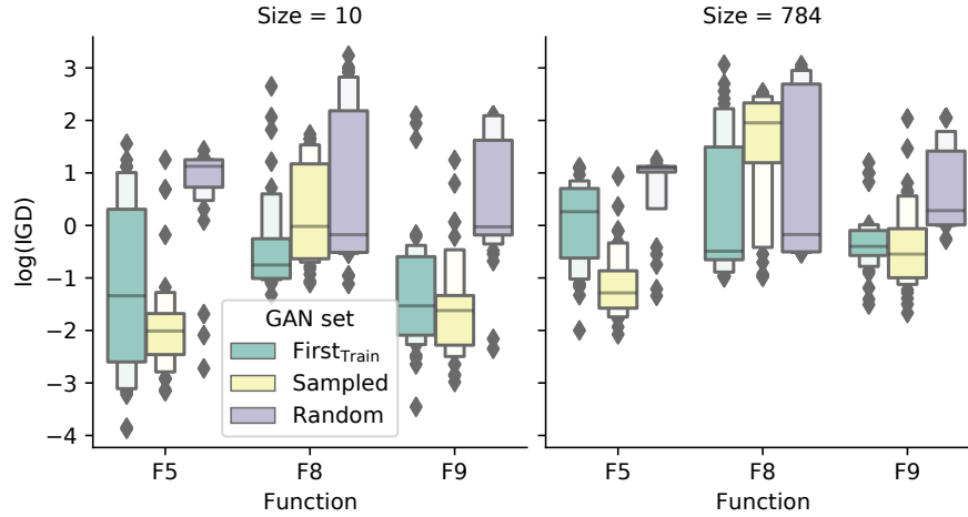
Fig. 4.4: IGD values obtained by GANs in the \text{First}_{\text{train}} set, GANs sampled from the metamodel, and GANs from the \text{Random}_{\text{train}} set.
