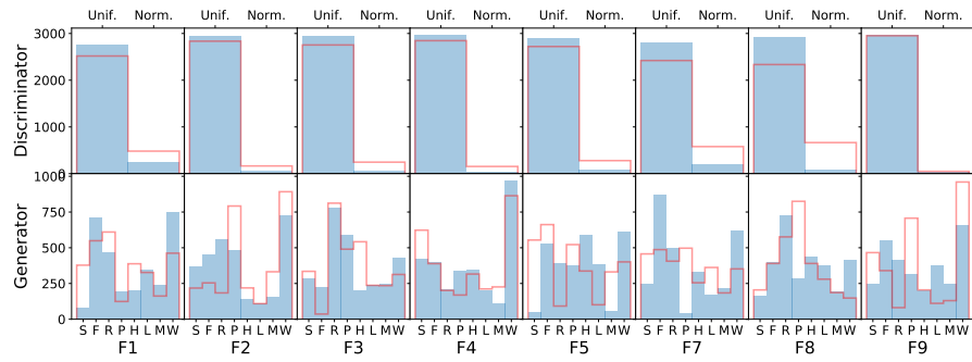
Fig. A.7: Loss functions and prior distributions used by the fully evolved GANs, for all functions with both problem dimensions. T: Total variation, S: Standard divergence, F: Forward KL, R: Reverse KL, P: Pearson \chi^2 , L: Least Squares.
