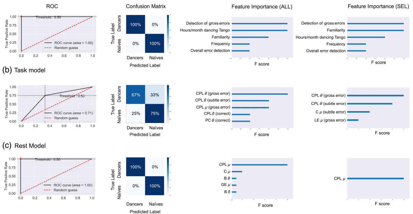
FIGURE 2 Machine learning results. Classification analysis (Tango dancers vs. Naïves) based on behavioral (a), task (b), and rest (c) functional connectivity features. On the left side, we plot the ROC curve and area under the curve (AUC) for each model. In the center, we provide the confusion matrix for each classifier. On the right side, we list the main features in order of importance for both classification analysis, with the approach including all the features (ALL) and the one including only those selected (SEL) based on the Recursive Feature Elimination (RFE) approach. B, betweenness centrality; C, clustering coefficient; CPL, characteristic path length; GE, global efficiency; LE, local efficiency; PC, participation coefficient; \delta : delta (1.5–4 Hz); \theta : theta (4–8 Hz); \mu : mu (8–13 Hz)
