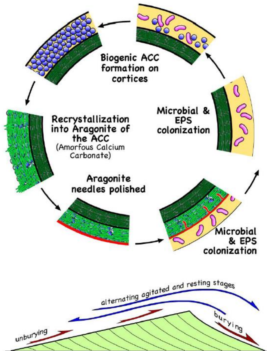
Figure 9. Conceptual multiphase model for the oolite cortex accretion. Abbreviations: ACC (amorphous CaCO 3 ) and EPS (extracellular polymeric substances). (This figure is an interpretation by L. Pomar based on cited sources [70,71]).
