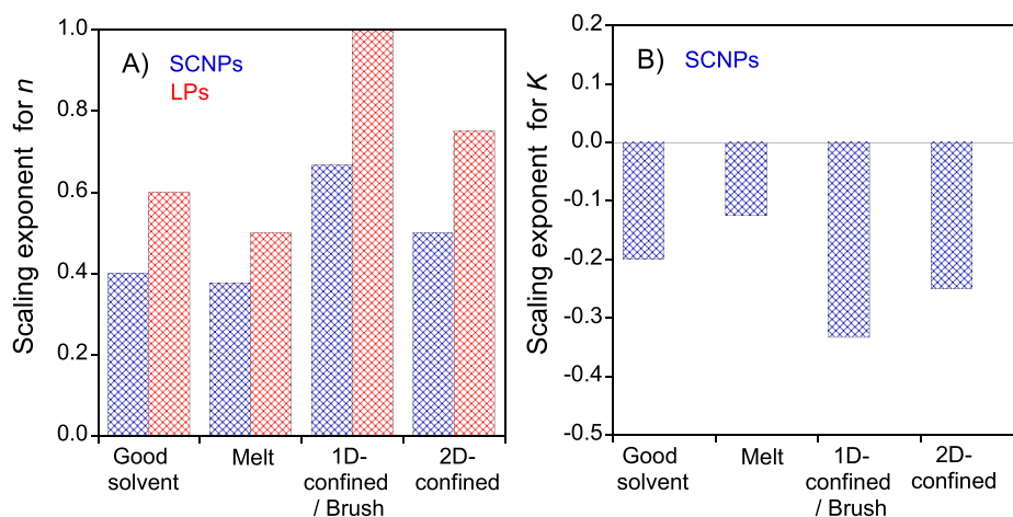
Fig. 3. A) Comparison of the scaling exponent for n corresponding to the conformational properties under different conditions (see Table 1) of elastic SCNPs (blue grid bars) vs. flexible linear polymers (red grid bars). B) Scaling exponent for K (see Table 1) of elastic SCNPs in different conditions. (For interpretation of the references to color in this figure legend, the reader is referred to the Web version of this article.)
