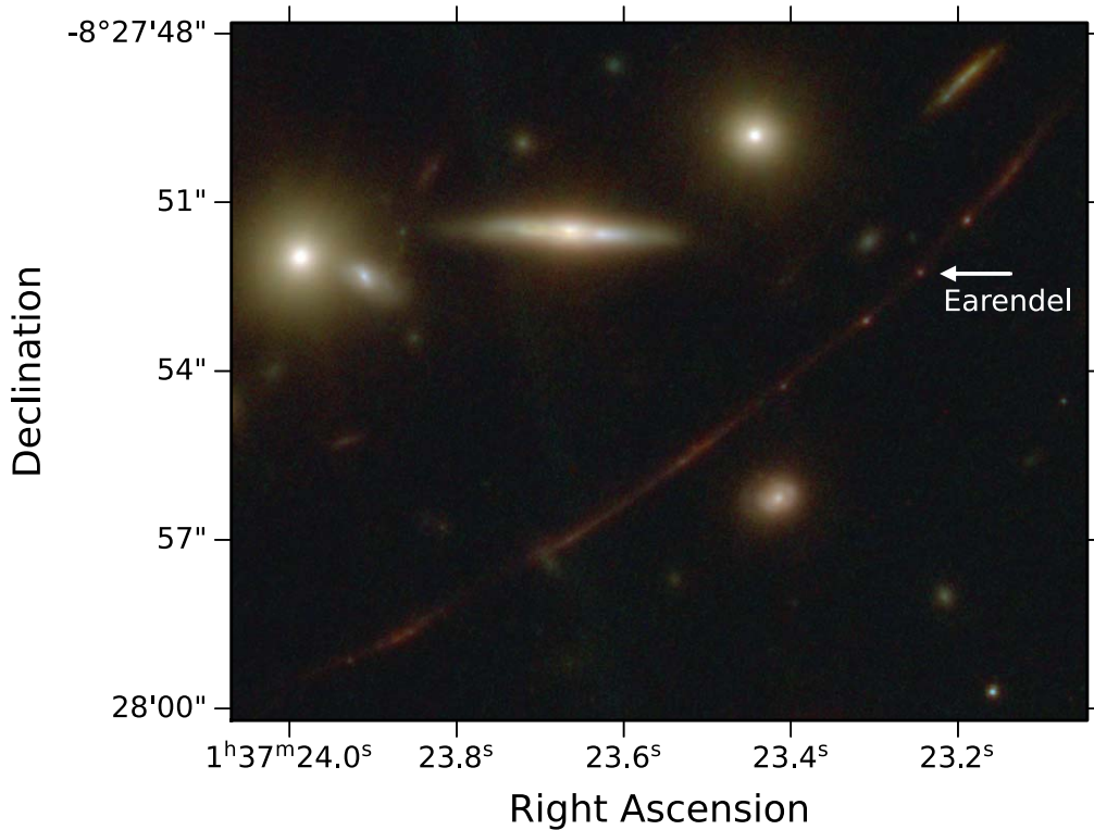
Figure 1. JWST NIRCcam image of the z \sim 6.2 Sunrise Arc, including the lensed star Earendel, marked with an arrow. This 15''.2 \times 12''.4 color image combines all eight NIRCcam images on a 0''.02 pixel scale.
