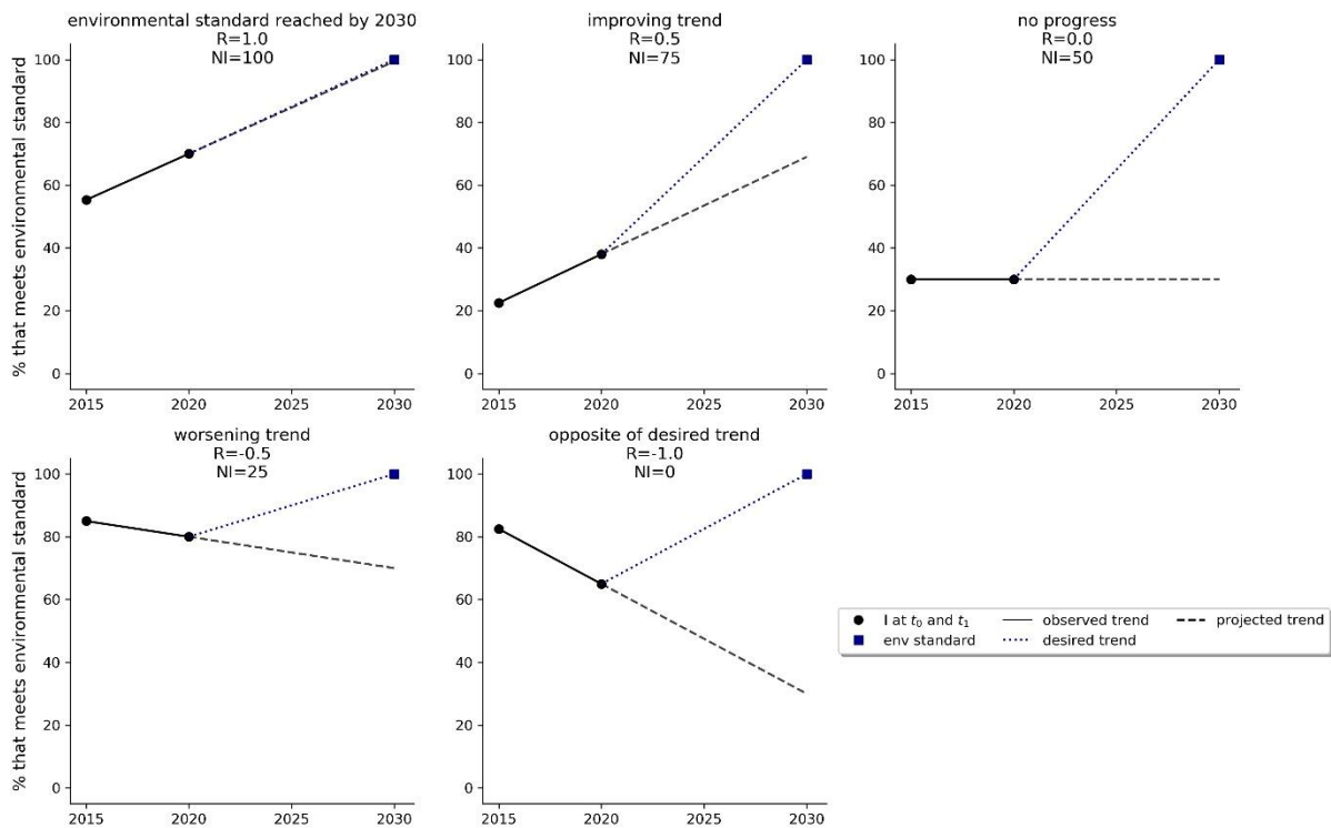
1 Figure 1: Interpretation of the normalised scores for a fictional indicator in different fictional 2 countries
