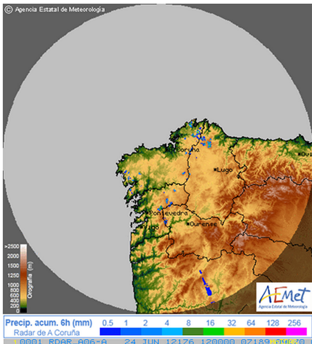
Fig. 4. Six hours accumulated rainfall map estimated by a C-band pulsed Doppler radars of the Spanish, weather radar network, in a sunny day without rain precipitation. Most of the blue colored areas do not correspond to precipitation, but to reflected signals from wind farms. (For interpretation of the references to color in this figure legend, the reader is referred to the web version of this article.) (Source: AEMET [78]).
