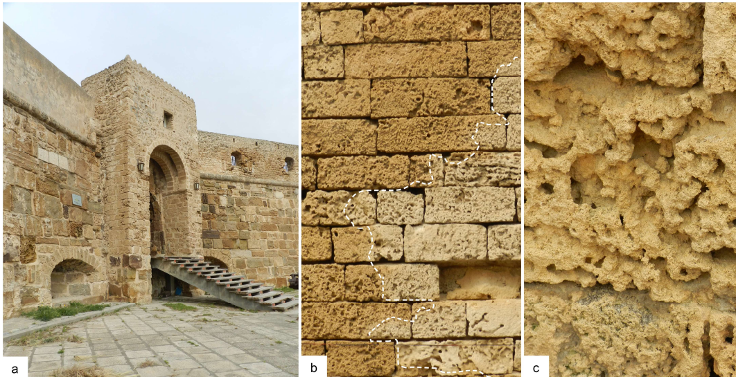
Figure 1. a) Spanish Fort of Bizerta (view from the port); b) Wall of the Fort with honeycomb weathering and moisture problems; c) Honeycomb weathering and loss of material on decayed stone ashlar
