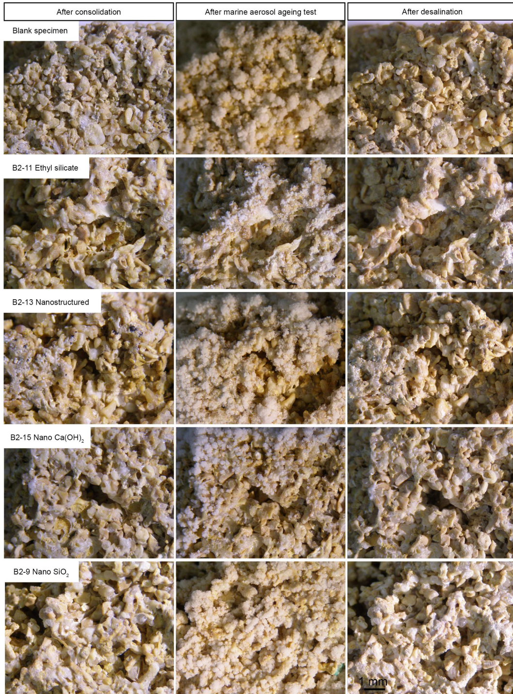
Figure 5. Surface detail images of the treated stones specimens (upper left corner) after one month from the consolidating product application, after marine aerosol ageing test and after being cleaned with water. The pictures were taken with an Olympus binocular loupe (SZ51) and a Olympus camera (C5060WZ, 5.1 megapixels, 5.7-22.9 mm)
