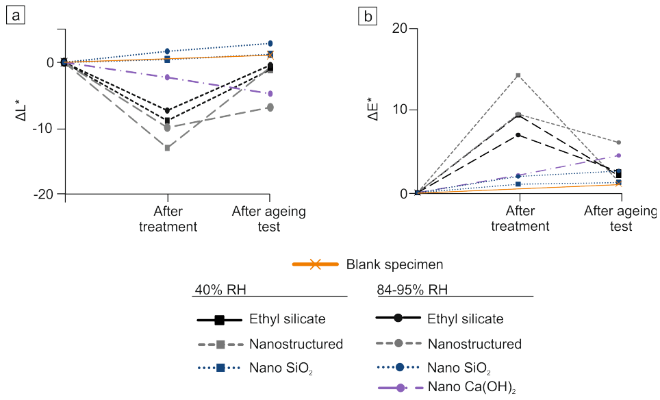
Figure 8. Comparison of luminosity ( \Delta L^* ) and total color ( \Delta E^* ) variations promoted on the stone specimens after one month from the application of different consolidating products and then after the marine aerosol ageing test
