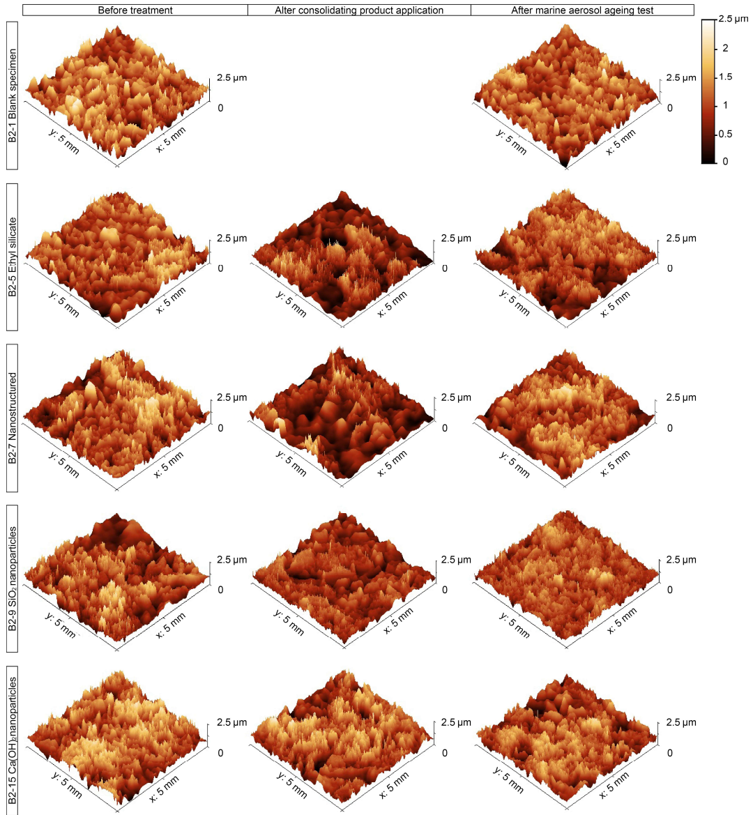
Figure 6. Surface roughness 3D height maps obtained under optical surface roughness (OSR) on the top surface of specimens before, after consolidating product application and after marine aerosol ageing test.
