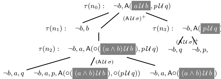
Figure 8: Application of (A\mathcal{U}\sigma)^+ and (A\mathcal{U}\sigma) rules to \{-b, A(a\mathcal{U}b, p\mathcal{U}q)\}
