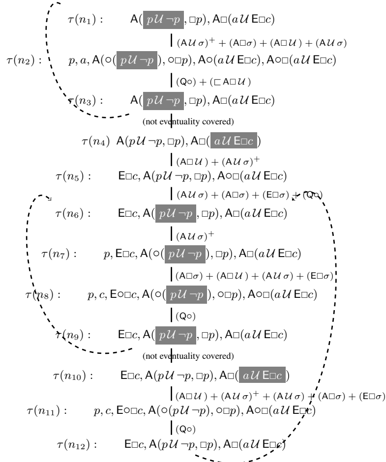
Figure 10: A branch in the systematic tableau for A(p\mathcal{U}\neg p, \Box p), A\Box(a\mathcal{U}E\Box c)
