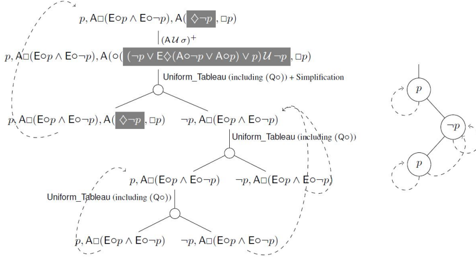
Figure 12: Open bunch in the tableau for p, A□(E◦p ∧ E◦¬p), A(◇¬p, □p) and represented model.
