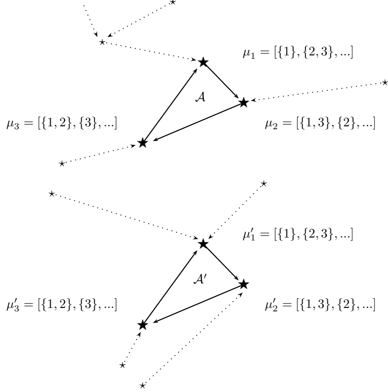
Figure 2.- The two absorbing sets of the roommate problem in Example 2.
