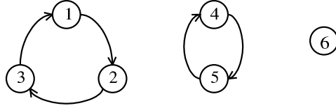
Figure 1.- A stable partition P .
