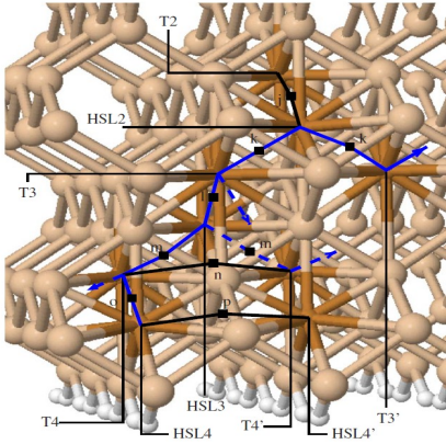
FIG. 4: (Color online) Migration routes for contaminating Cu inside bulk Si. The lowest (possible) energy routes are displayed in solid (dashed) blue lines whereas black solid lines indicate the rest of the considered migration routes.
