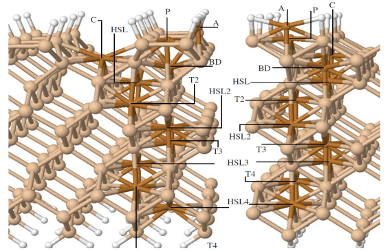
FIG. 2: (Color online). Adsorption sites considered within this work both on the surface (P, C, A and B) and beneath (T4, T3, T2, HSL4, HSL3, HSL2, HSL, and BD).
