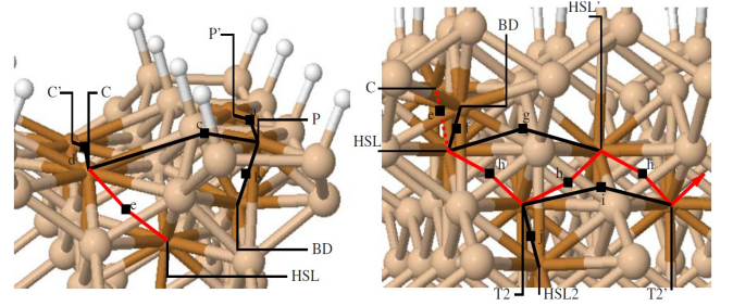
FIG. 3: (Color online) Migration routes for Cu deposited from vacuum: (a) surface routes and (b) subsurface routes. The lowest energy routes are displayed in red whereas black indicates the rest of the migration routes considered. Atoms at HSL could also move towards C where they would return to HSL and would finally migrate to T2. This fact is reflected in the dashed red line between HSL and C.
