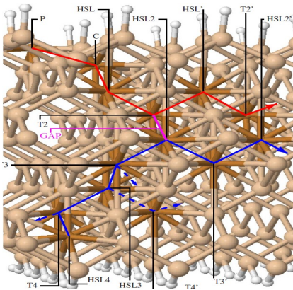
FIG. 5: (Color online) Lowest-energy migration routes for both depositing Cu from vacuum and contaminating Cu from bulk Si. The migration route for depositing Cu from vacuum is displayed in red whereas blue is used for contaminating Cu. Alternative possible migration routes followed by contaminating Cu along both parallel and perpendicular directions to the dimer row are displayed in blue dashed lines. Magenta is used to represent the large energy barrier opened between the T2 and HSL2 sites.
