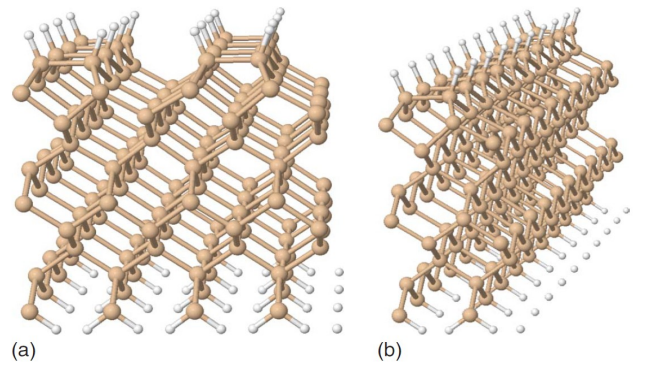
FIG. 1: (Color online). Slab geometries used for simulating H-passivated si(001) surface: left, square cell; right, nanoline cell
