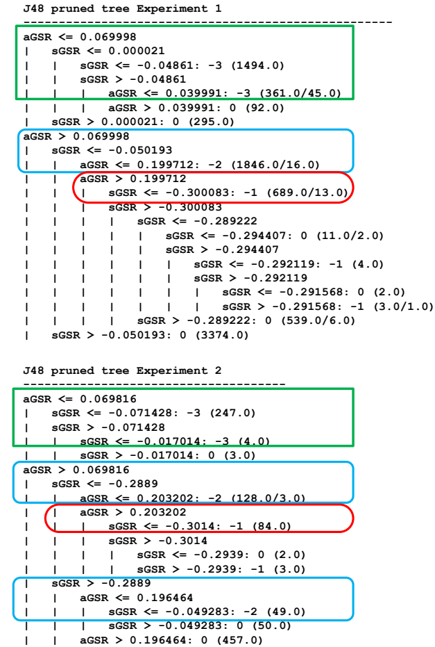
FIGURE 5. The sets of rules extracted from the Decision Trees for each experiment.
