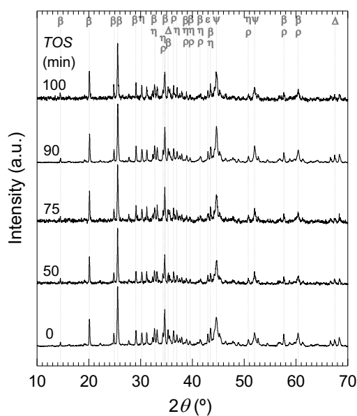
Figure 2. XRD spectra of the reduced fresh catalyst (0 min) and deactivated at several values of time on stream. Assigned bands: \text{Ni}^0 ( \psi ); \text{NiO} ( \epsilon ); \text{Al}_2\text{O}_3 ( \Delta ); \text{CaO}(\text{Al}_2\text{O}_3)_2 ( \beta ), \text{CaAl}_2\text{O}_4 ( \eta ); \text{CaAl}_{12}\text{O}_{19} ( \rho ).
