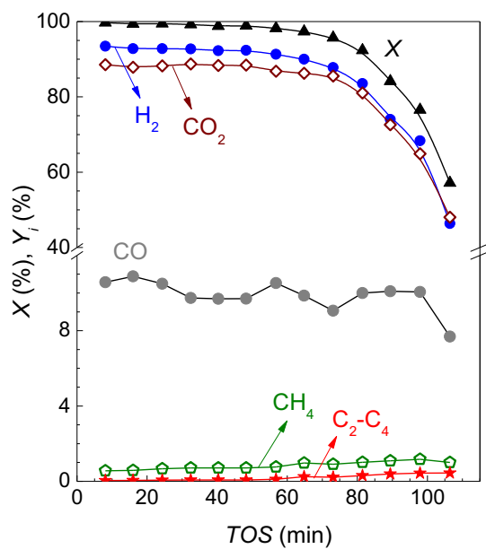
Figure 1. Evolution with time on stream of the conversion of volatiles from biomass pyrolysis ( X ) and yield of products ( Y_i ).
