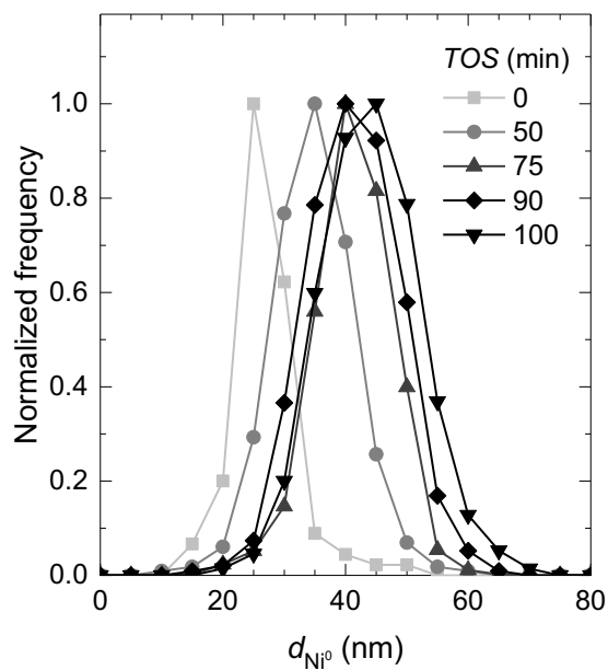
Figure 6. Evolution with time on stream of the distribution of Ni^0 crystal size of the catalyst, based on TEM images.
