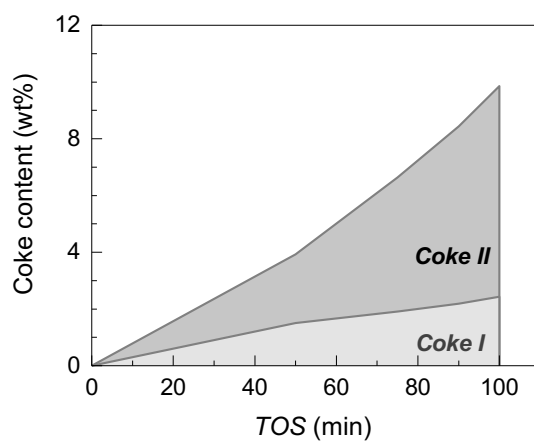
Figure 8. Evolution with time on stream of the content of coke deposited on the catalyst.
