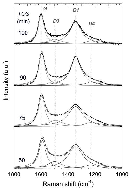
Figure 9. Evolution with time on stream of the Raman spectra (1000-1800 \text{cm}^{-1} region) of the coke deposited on the catalyst.
