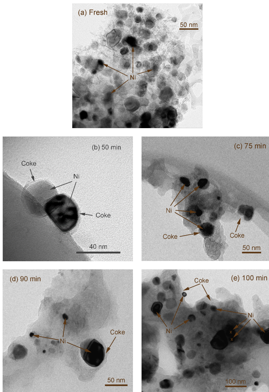
Figure 5. TEM images of the fresh catalyst (a) and used at time on stream values of 50 min (b), 75 min (c), 90 min (d) and 100 min (e).
