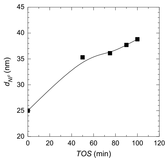
Figure 3. Evolution with time on stream of Ni^0 crystal size of the fresh reduced and deactivated catalysts, determined by XRD.
