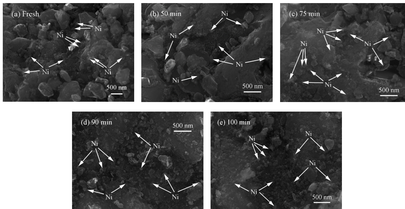
Figure 4. SEM images of the fresh catalyst (a) and deactivated at several values of time on stream: 50 min (b); 75 min (c); 90 min (d); 100 min (e).
