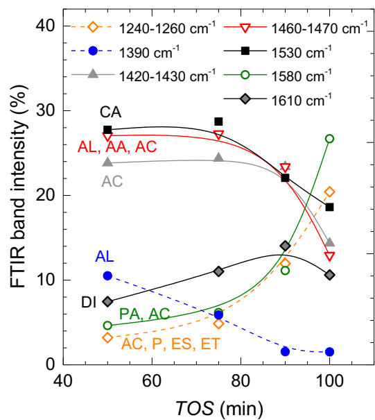
Figure 11. Evolution with time on stream of the relative intensities of several representative FTIR bands corresponding to functional groups in the deposited coke. Abbreviations: alkyl aromatics (AA), aliphatics (AL), acetates (AC), carbonates (CA), dienes (DI), esters (ES), ethers (ET), phenols (P), polyaromatics (PA).
