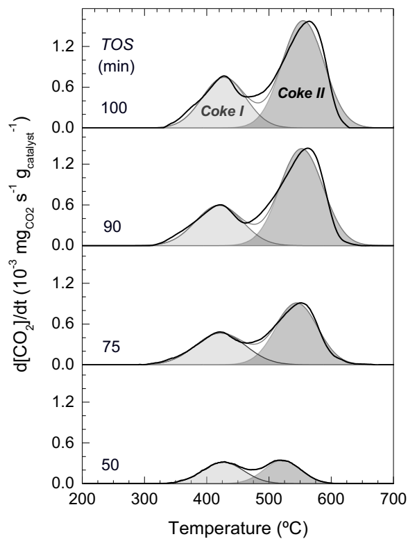
Figure 7. Evolution with time on stream of the TPO profiles of coke combustion.
