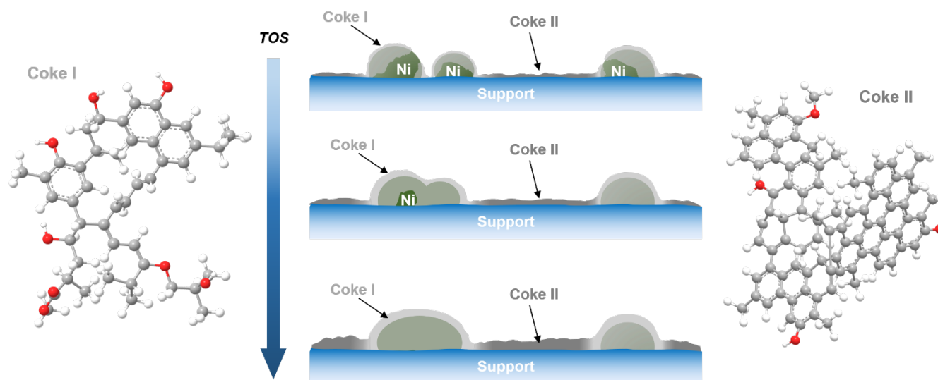
Figure 12. Proposed molecular structures and location of coke with time on stream, based on its characterization.
