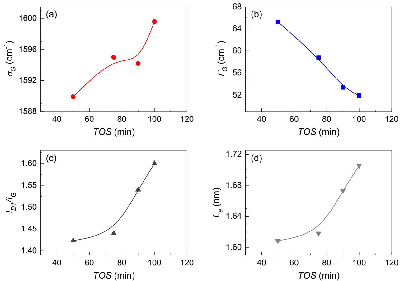
Figure 10. Evolution with time on stream of representative Raman parameters of the coke deposited: G band position ( \sigma_G ) (a); G band width ( \Gamma_G ) (b); I_{D1}/I_G ratio (c); size of carbon domain ( L_a ) (d).
