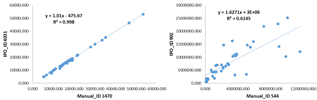
Figure S.2. Correlation graph between two features obtained by IPO and Manual selection criteria for Liver ESI+. The left graph a good correlation and same features are shown (IPO_ID4031 = Manual_ ID1470), whereas the right graph shows the opposite situation (IPO_ID902 ≠ Manual_ID544).
