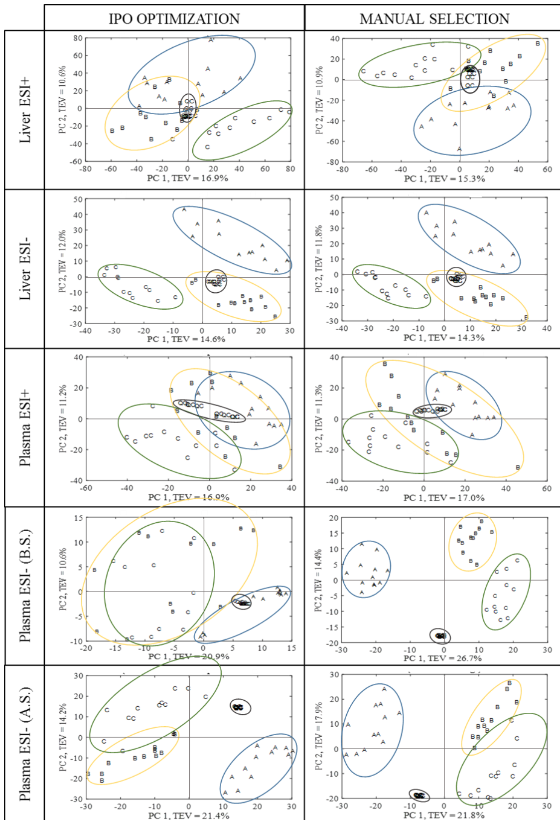
Figure S.1. PCA scores plot, before intensity drop correction and pertinent transformation obtained with IPO and manual parameters selection criteria for the all data sets (Liver ESI+, Liver ESI-, Plasma ESI+, Plasma ESI- B.S., and Plasma ESI- A.S.). Piglets groups: newborns (A), neonates (B) and infants (C).
