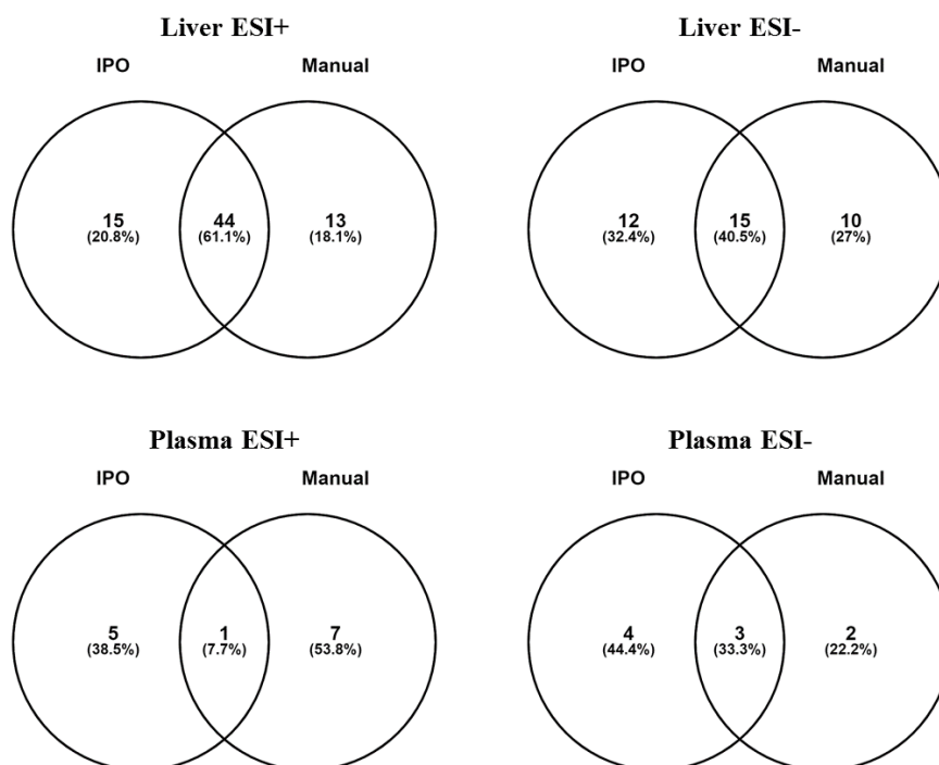
Figure 2. Venn Diagrams highlighting the common and uncommon features of interest for liver and plasma matrices at both positive and negative ionization modes.
