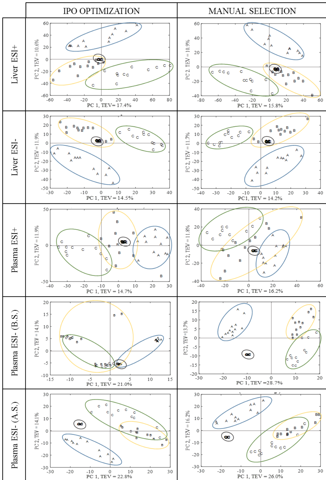
Figure 1. PCA scores plot obtained with IPO and manual parameters selection criteria for the all data sets (Liver ESI+, Liver ESI-, Plasma ESI+, Plasma ESI- B.S., and Plasma ESI- A.S.). Piglets groups: newborns (A), neonates (B) and infants (C).
