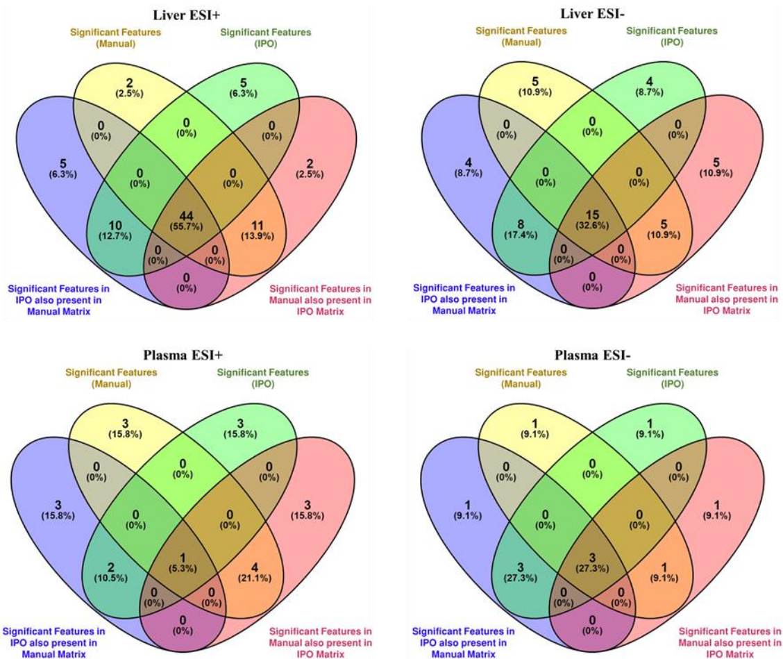
Figure 3. Venn diagrams highlighting the significant features detected with IPO or Manual approaches that are coincident in the other approach matrix (but did not meet the statistical tests to be considered as significant features).
