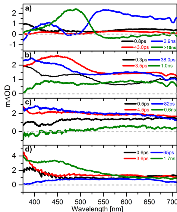
Fig. 5 Decay associated spectra (DAS) for the four studied AIs in ACN. The graphs show the weights along the spectra of the lifetimes derived from the modelling of the TA data obtained after excitation at 267 nm. See Experimental section for details.
