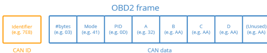
Figure 3: OBD2 frame structure. [5]
