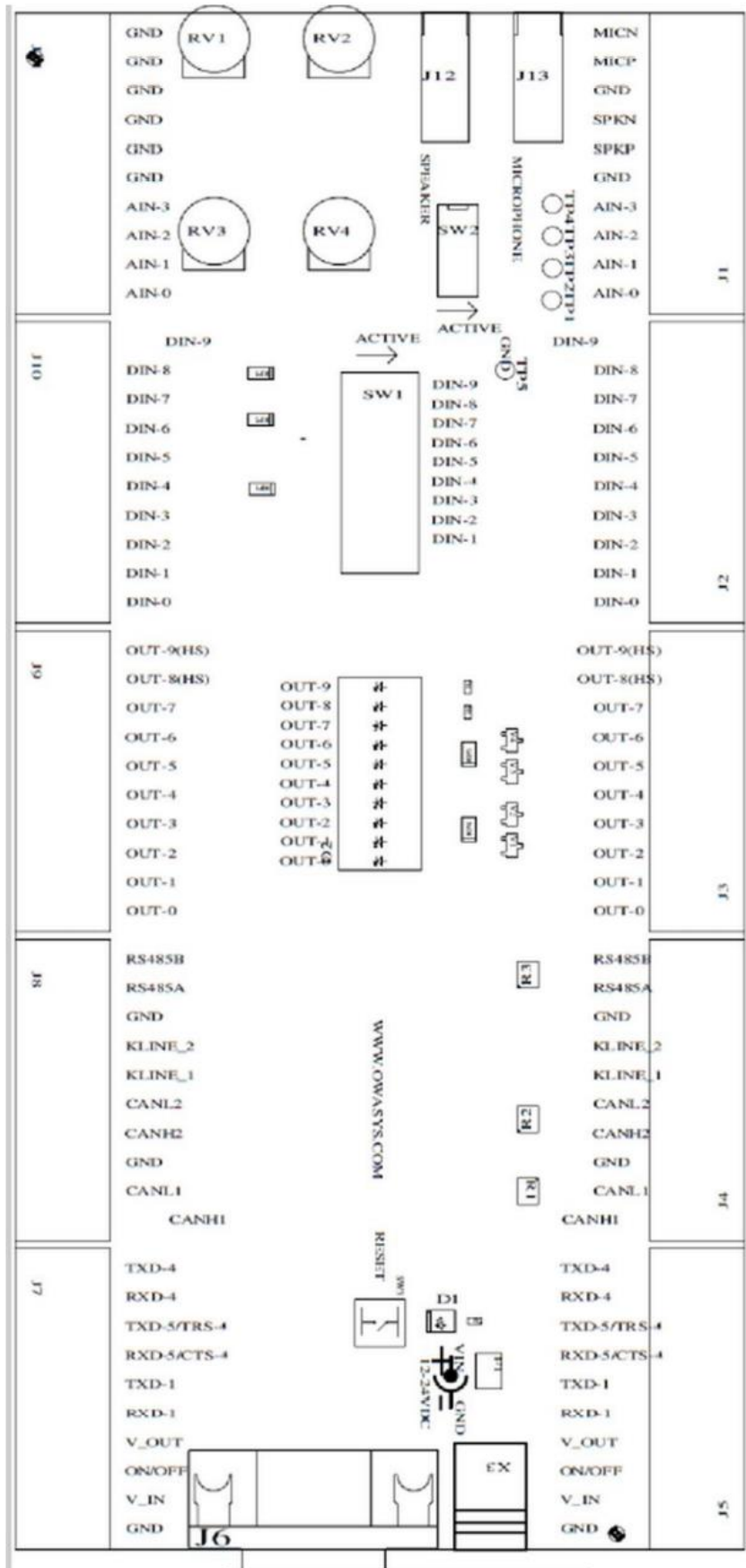
Figure 6: Owasys developers board physical description.
