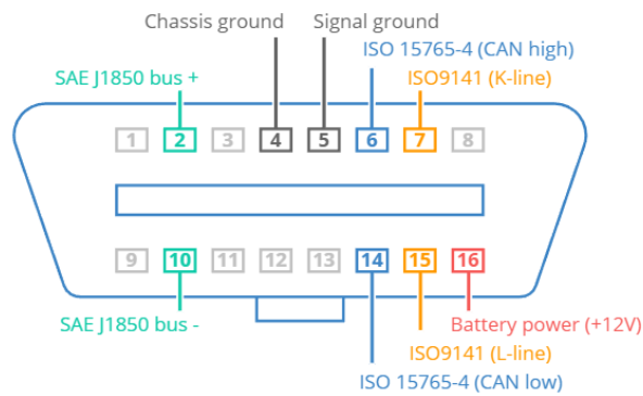
Figure 8: OBD connector pinout. [5]
