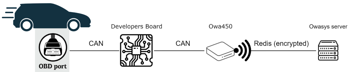
Figure 9: Graphic representation of the implemented setup
