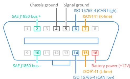
Figure 2: OBD connector pinout. [5]
