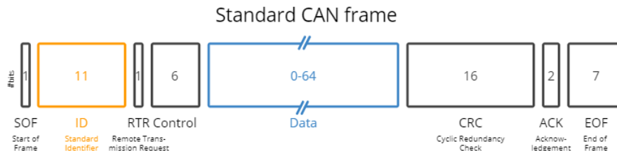
Figure 1: CAN frame structure. [5]
