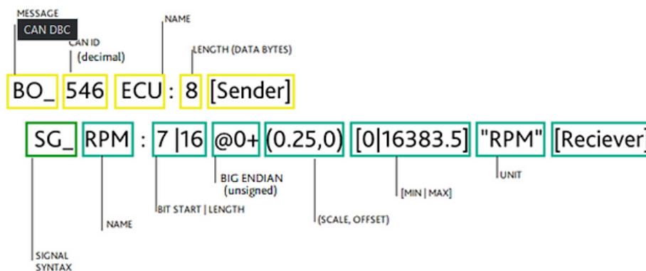
Figure 4: DBC file entry example.
