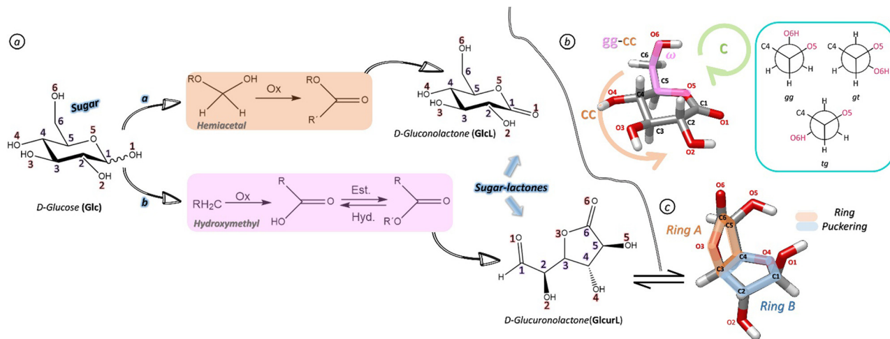
Fig. 1 (a) Scheme of the oxidation reactions from D-glucose ( Glc ) to D-gluconolactone ( GlcL ) (pathway a) and D-glucuronolactone ( GlcUrL , linear form) (pathway b). Reaction intermediates are shown in the orange and pink squares. (b) Labelling used for GlcL , together with the three plausible staggered configurations of the CH 2 OH group with respect to the sugar ring shown in blue. The green arrow (clockwise, c ) and the orange arrow (counterclockwise, cc ) show the two possible orientations of the cooperative hydrogen bonding network. (c) Labelling used for GlcUrL (bicycle furanose form, in chemical equilibrium with the linear one) and ring-puckering marked in orange and blue.
