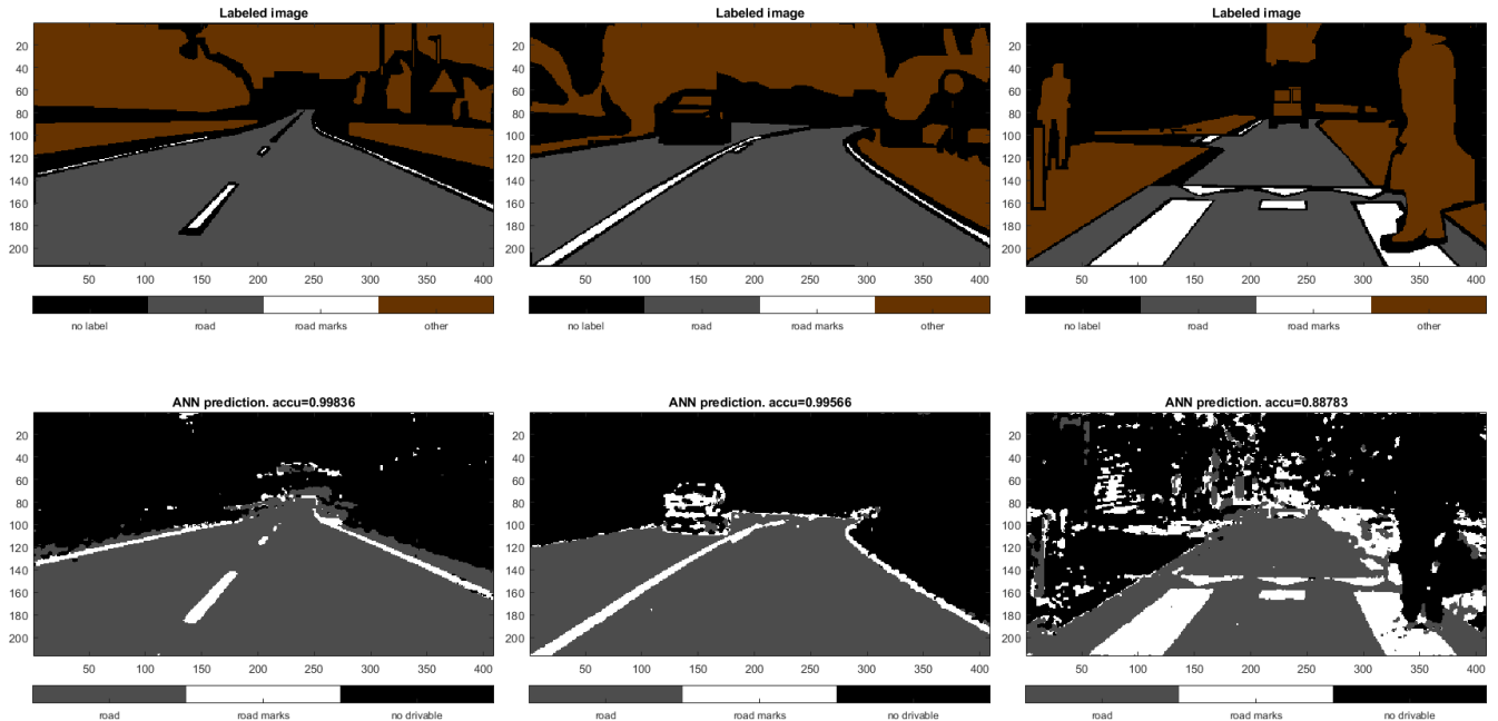
Fig. 4: Image segmentation examples for experiment 1: ground-truth images (top) and segmented images (bottom)
