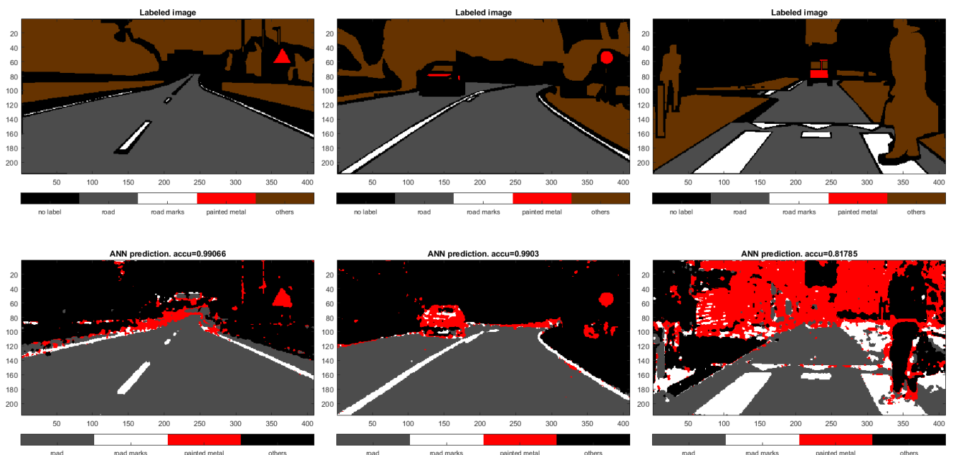
Fig. 5: Image segmentation examples for experiment 2: ground-truth images (top) and segmented images (bottom)
