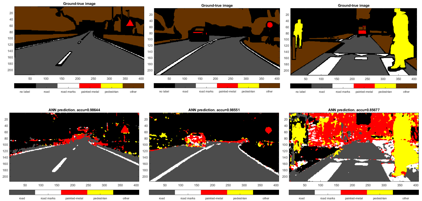
Fig. 6: Image segmentation examples for experiment 3: ground-truth images (top) and segmented images (bottom)
