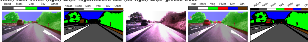
Fig. 7. Image 566 (f4, AG2, 10ms), captured during a winter, sunny morning, in a road with overexposure: (far left) Exp2 segmentation, (left) Exp2 ground-truth, (center) false color, (right) Exp3 segmentation and (far right) Exp3 ground-truth.
