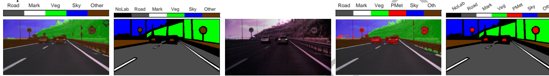
Fig. 3. Image 557 (f4, AG2, 10ms), captured during a winter, sunny morning, in a highway: (far left) Exp2 segmentation, (left) Exp2 ground-truth, (center) false color, (right) Exp3 segmentation and (far right) Exp3 ground-truth.
