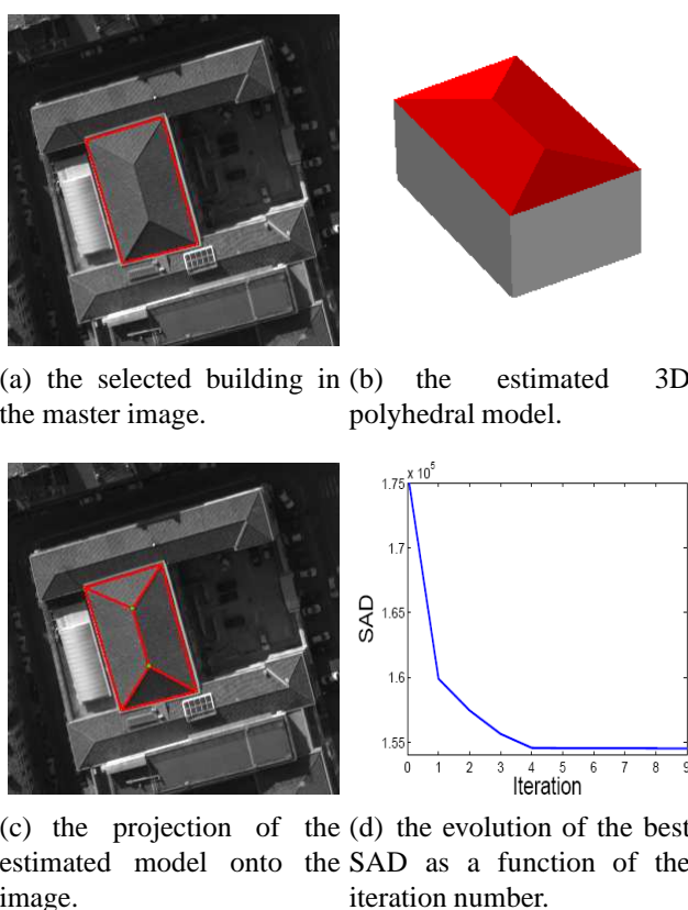
Figure 13. Estimated 3D polyhedral building model and related convergence.
