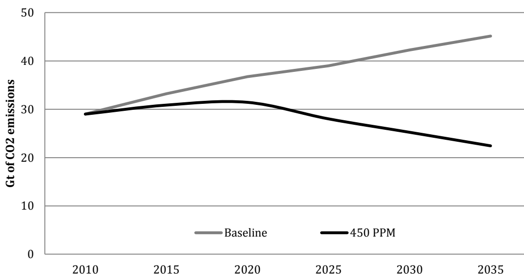
Figure 2: CO2 emissions paths along Baseline and 450 PPM (Gt of CO2). Source: own elaboration on GDynE results calibrated with WEO 450PPM Scenario(IEA, 2013)
