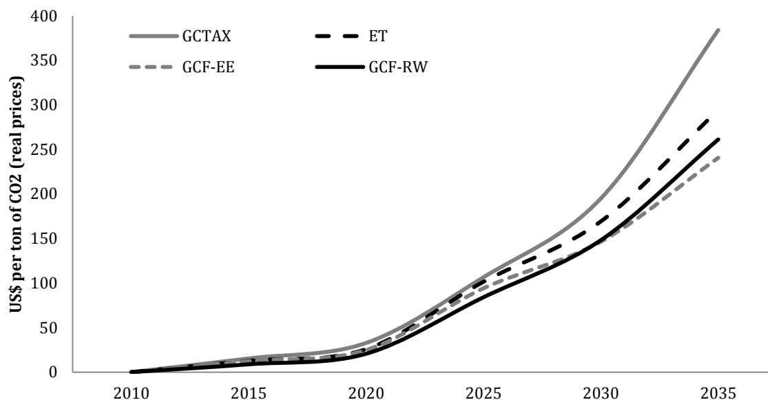
Figure 3: Real carbon price in different scenarios on track for 450 PPM (US$ per ton of CO 2 ). Source: own elaboration on GDynE results calibrated with WEO 450PPM Scenario (IEA, 2013b)
