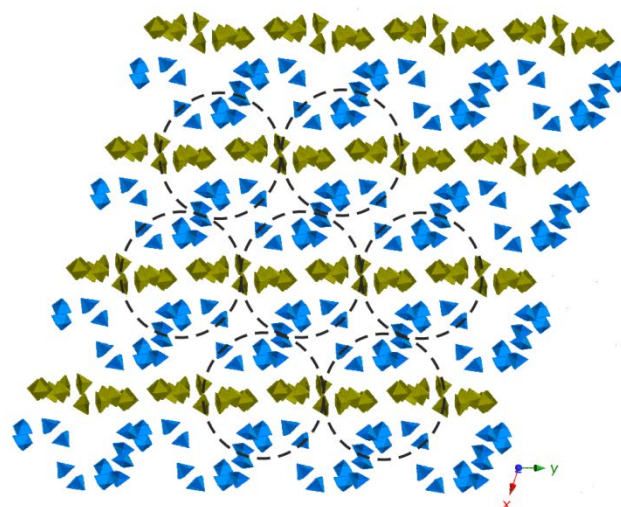
Fig. 3 [001] view of the supramolecular 3D framework for compound 1 .
