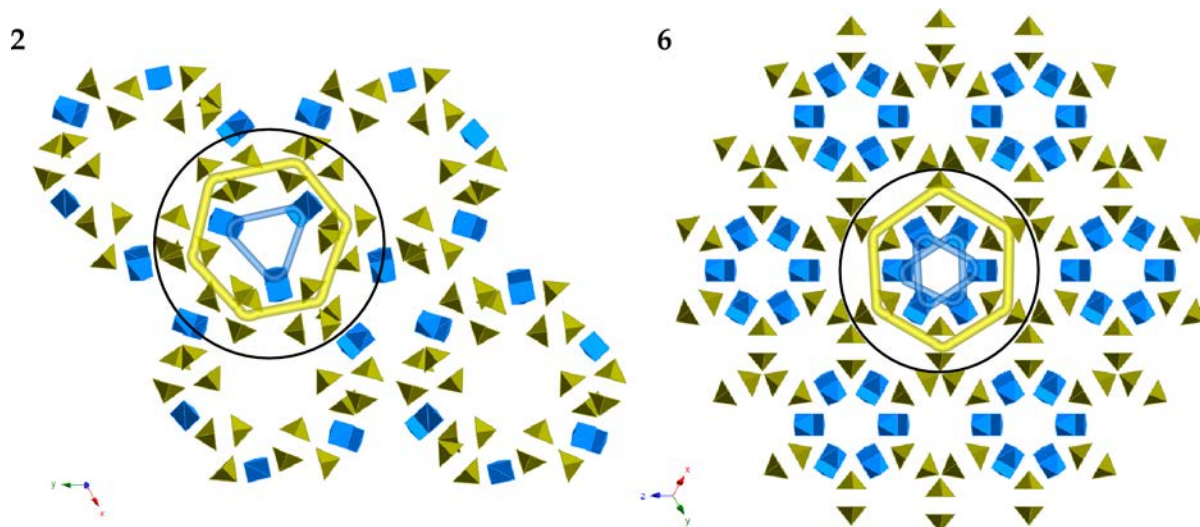
Fig. 8 Mother structures for Cu 24 -clusters: HCP-type (compound 2 ) and CCP-type (compounds 6 and 7 ).
