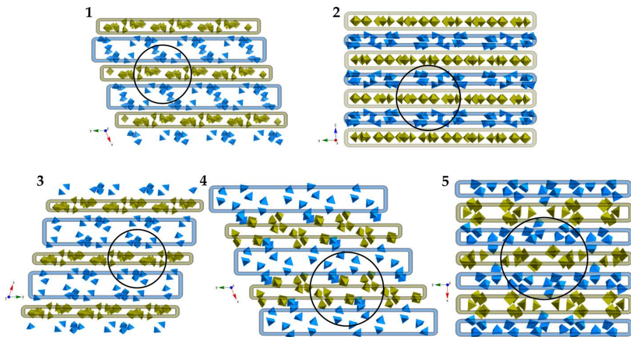
Fig. 6 Layered 3D frameworks for compounds 1-5. Dotted circles mark the \text{Cu}_{24} -clusters. Green and blue polyhedra are the twelve dimmers per \text{Cu}_{24} -cluster.
