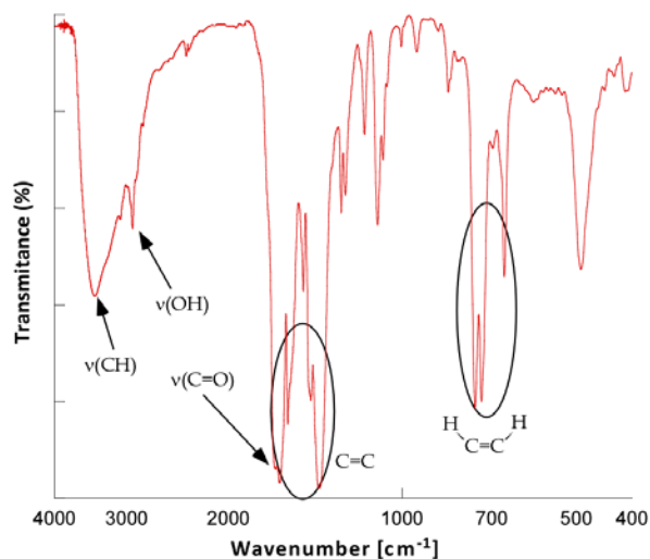
Fig. 4 Infrared spectra for compound 1 .
