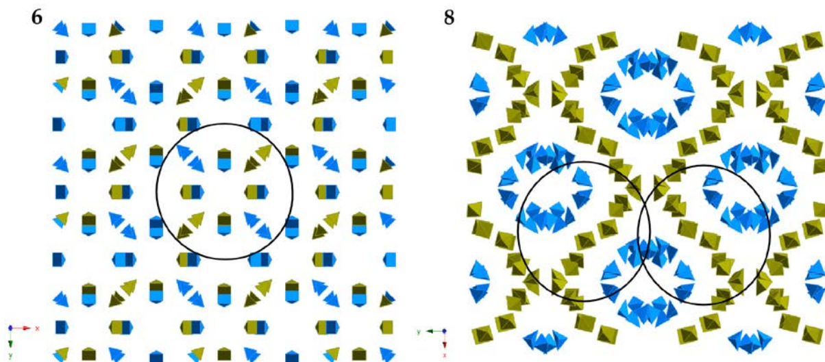
Fig.7 3D framework for compounds 6 (or 7) and 8. Dotted circles mark the \text{Cu}_{24} -clusters. Green and blue polyhedra are the twelve dimmers per \text{Cu}_{24} -cluster. Clusters for 8 are packed in two different orientations.
