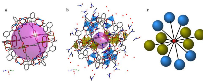
Fig. 2 View of the Cu 24 -cluster (a) where solvent molecules have been omitted, and (b) where localized solvent molecules per formula unit are shown. The purple spheres represent the accessible volume: (a)=2145 Å 3 , (b)=904 Å 3 . Other color codes: C, grey; O, red; Cu (central), green; and Cu (upper and lower), blue. Hydrogen atoms are omitted for clarity. (c) Schematic view of the Cu 24 -cluster where blue and green spheres account for the twelve dimers per cluster.
