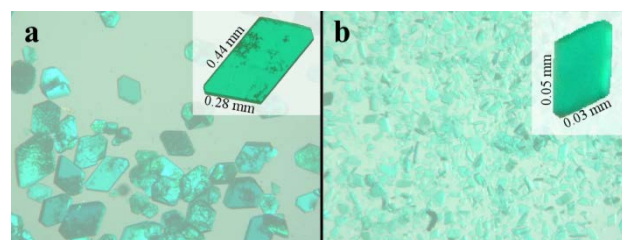
Fig. 1 Single crystals of compound 1 using the protoporphyrin IX as a crystallization helper (a), and without it (b).
