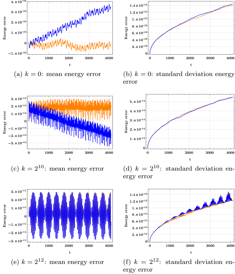
Figure 1: Evolution of mean (left) and standard deviation (right) of relative errors in energy for fixed-point implementation (blue), and Newton implementation (orange). Non-stiff case k = 0 (a,b), one stiff case k = 2^{10} (c,d) and second stiff case k = 2^{12} (e,f)
