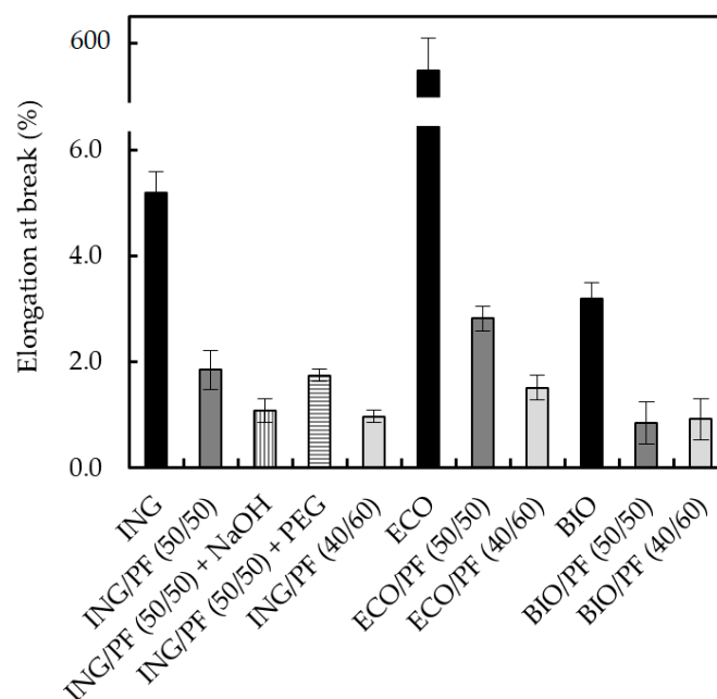
Figure 8. Elongation-at-break values of neat polymers and the different biocomposites containing 50 and 60 wt % of CFs.
