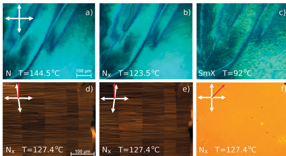
Fig. 2 Polarisation microscopy textures observed in (a–c) sandwich cells of compound 1 at different temperatures and (d–f) in 2.4 \mu\text{m} cell at 127.4\text{ }^\circ\text{C} . (d and e) Inversion of the N_x domain contrast under 15^\circ analyzer uncrossing (clock- and anti-clockwise) in the extinction position (right-side area still in N phase). (f) Sample rotated 45^\circ with respect to the crossed polarisers.
