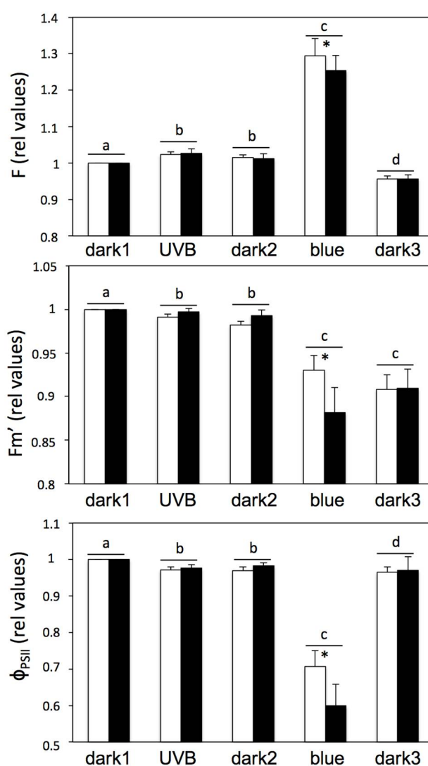
Figure 3. Effect of UV-B and blue light treatments on F, Fm', and \phi_{PSII} on thalli with (open bars) or without (closed bars) parietin, following the kinetic assay described in Supplementary Figure S2. Control values (first measurement in darkness) for \phi_{PSII} were 0.588 \pm 0.020 and 0.532 \pm 0.044 (nonsignificant differences) for samples with and without parietin, respectively. Data are average \pm SE ( n = 6 ). Significant differences among light treatments are indicated with different letters and between thalli with or without parietin with an asterisk ( p < 0.05 ).
