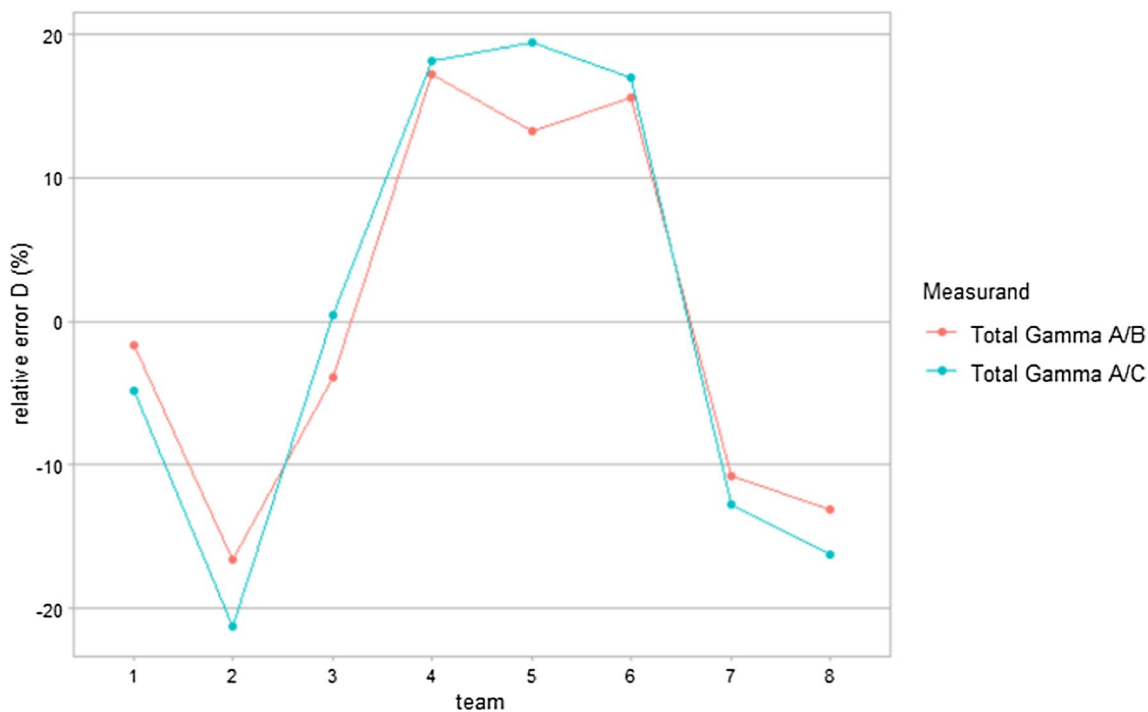
Fig. 3 Relative deviation from consensual value for total gamma measurement ratios
